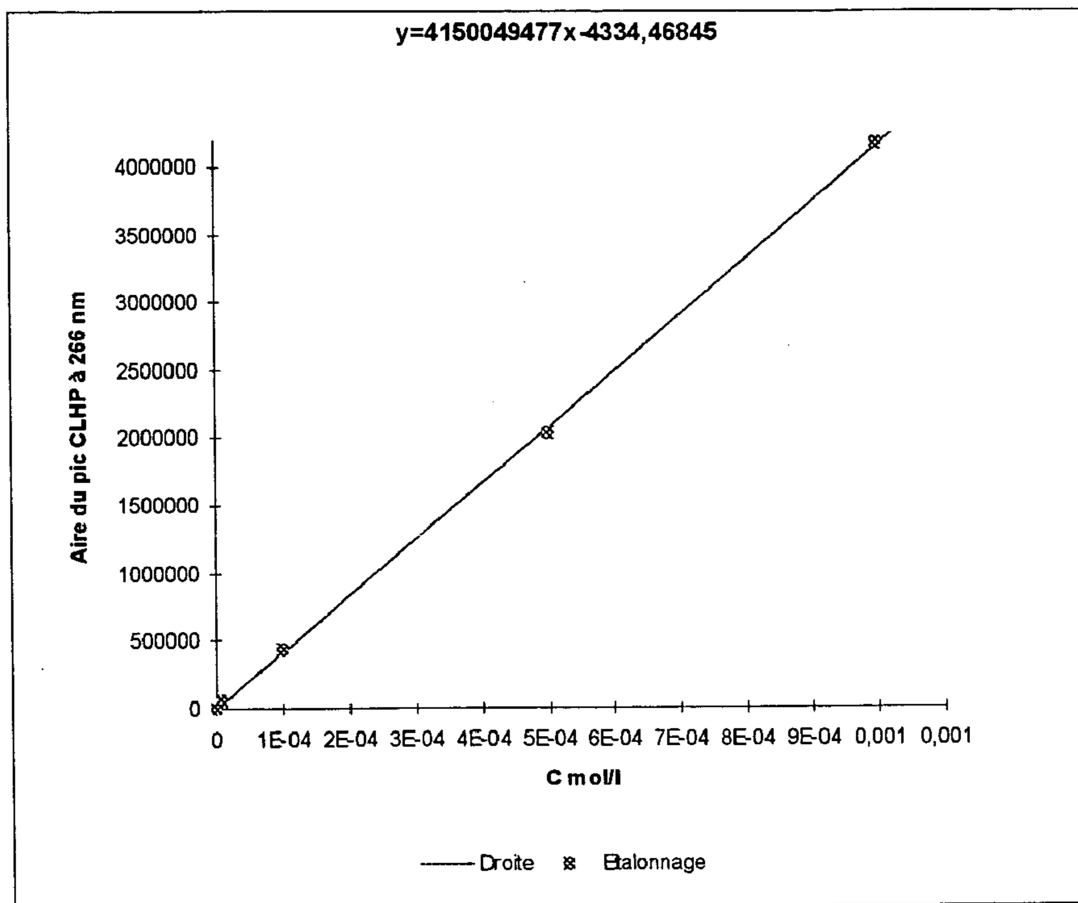
Figure 8a Solubility Calibration Curve for D-dC
