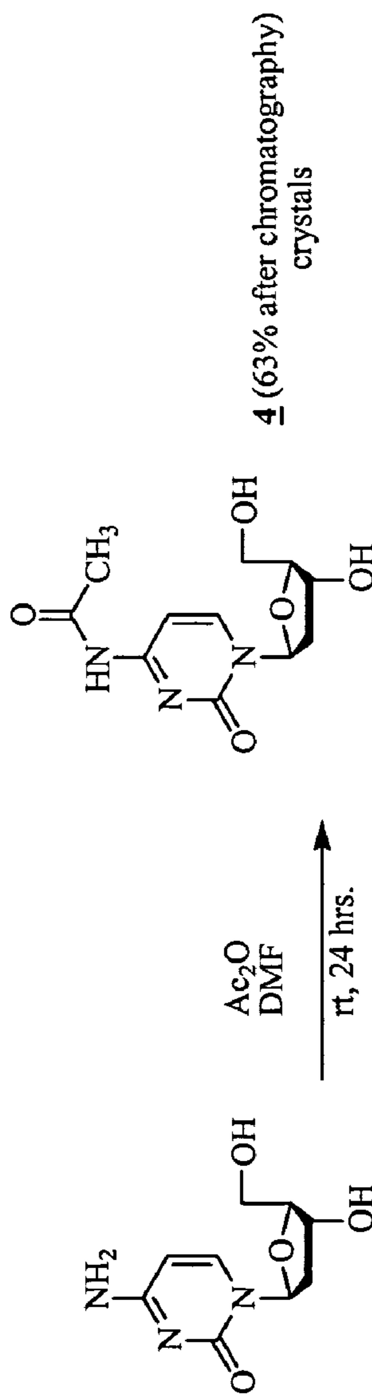
Figure 2 Synthesis of N 4 -acetyl-2'-deoxy- \beta -L-cytidine
