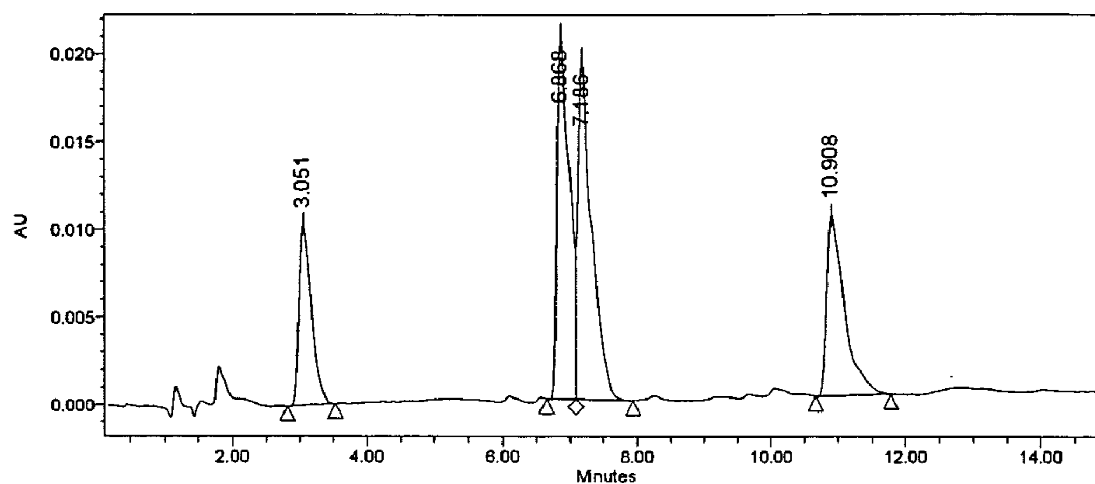
Figure 11a HPLC profile – 95.7 hours at pH of 4.51
