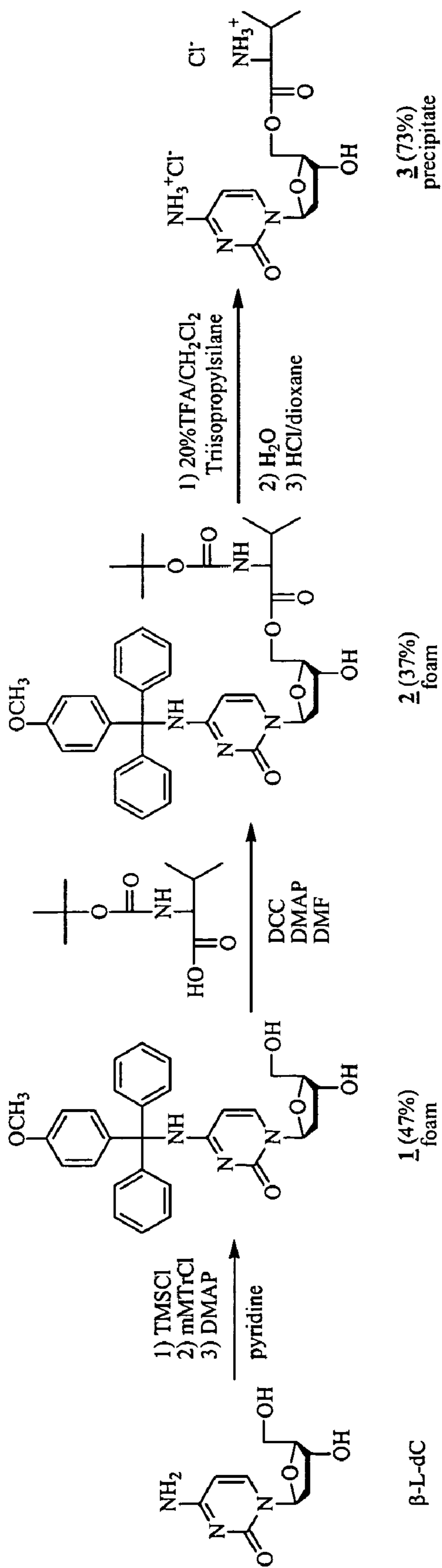
Figure 1 Synthesis of 5'-valinyl esters of 2'-deoxy- \beta -L-cytidine
