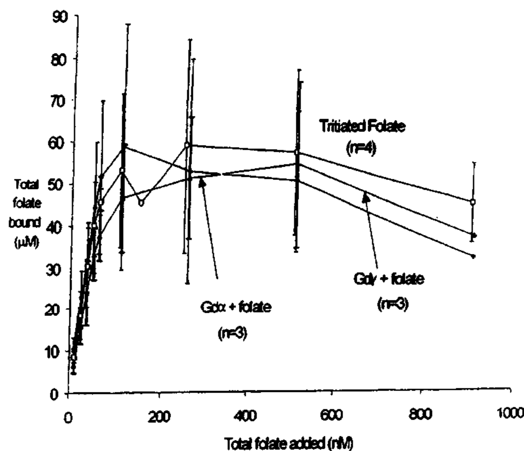
Binding of ^{153}\text{Gd-DO3A-APA-(}\alpha\text{)-folate} , ^{153}\text{Gd-DO3A-APA-(}\gamma\text{)-folate} or ^3\text{H folate} to KB cells at 37°C
