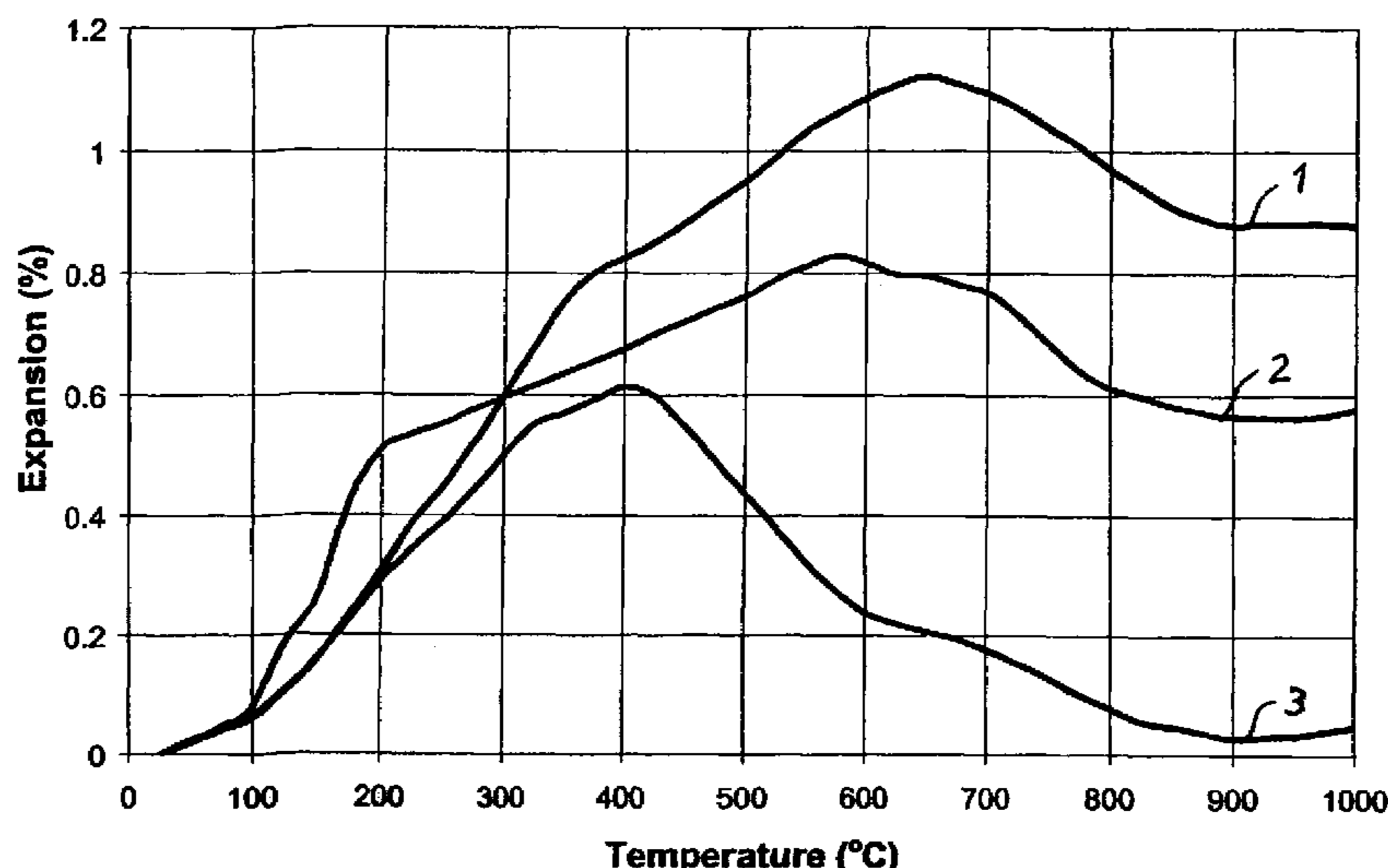
1- New Swelling Cold Paste 2- Standard Cold Paste 3- Vesuvius CP45
