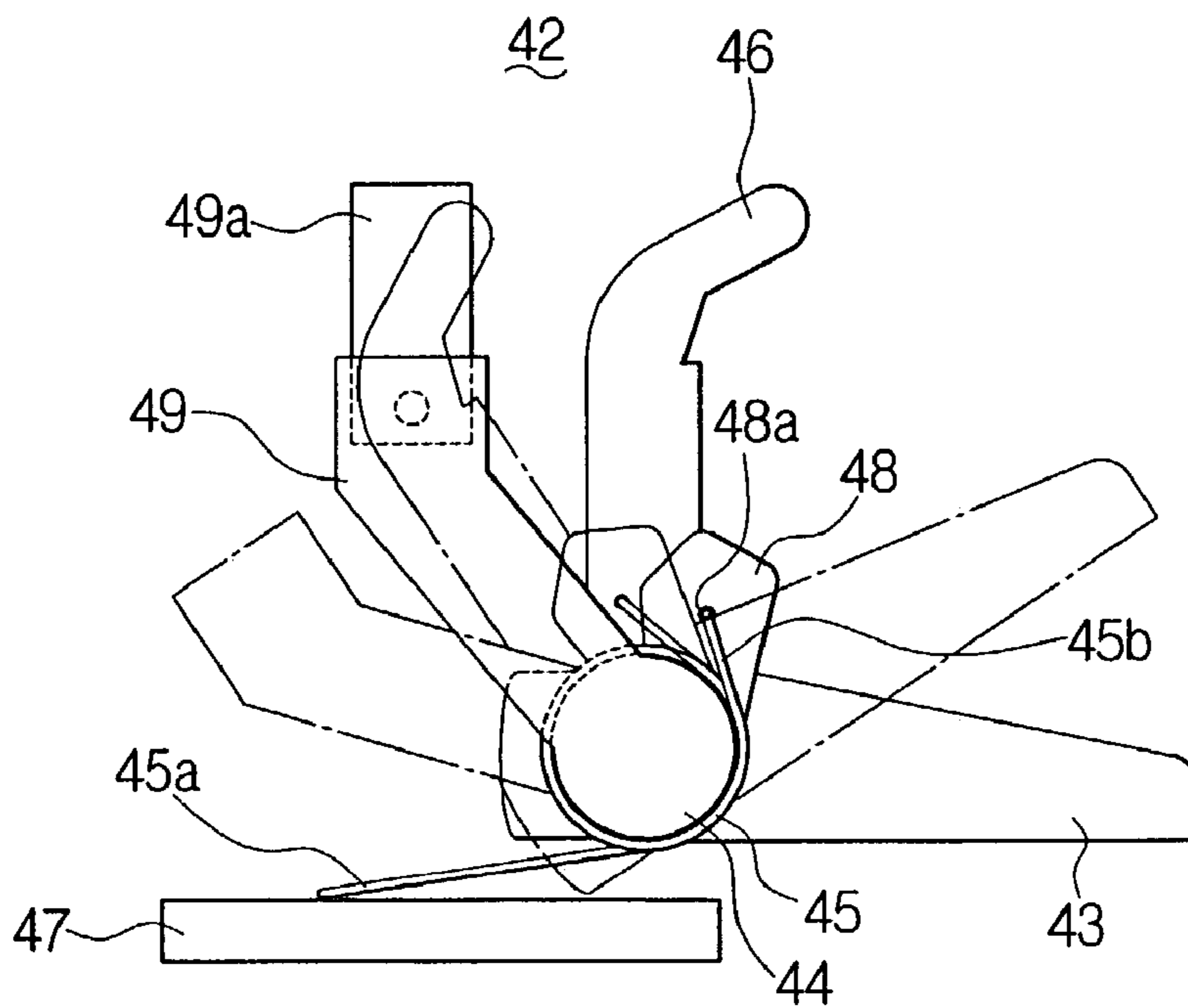
FIG. 3 (PRIOR ART)
