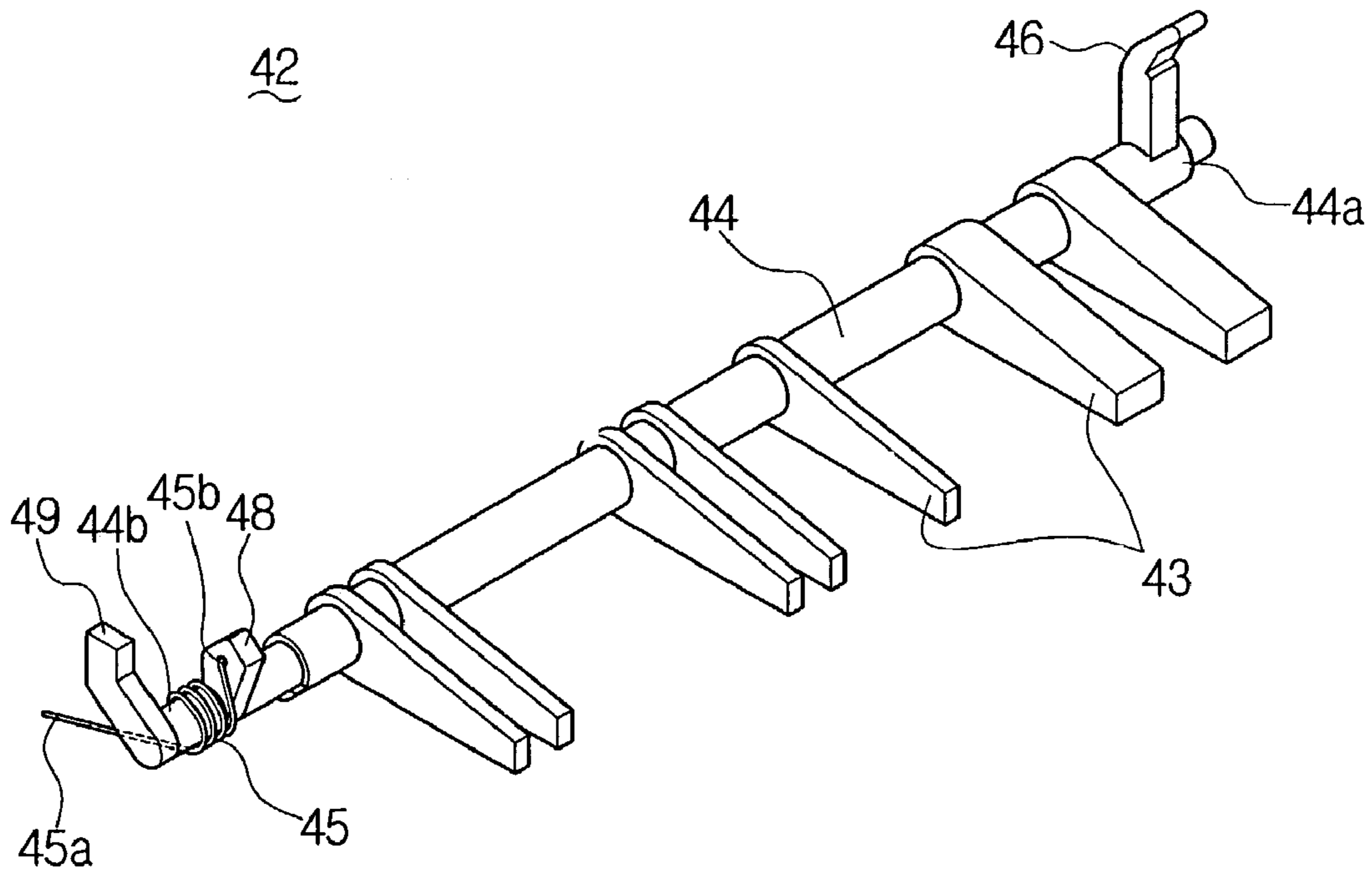
FIG. 3 (PRIOR ART)
