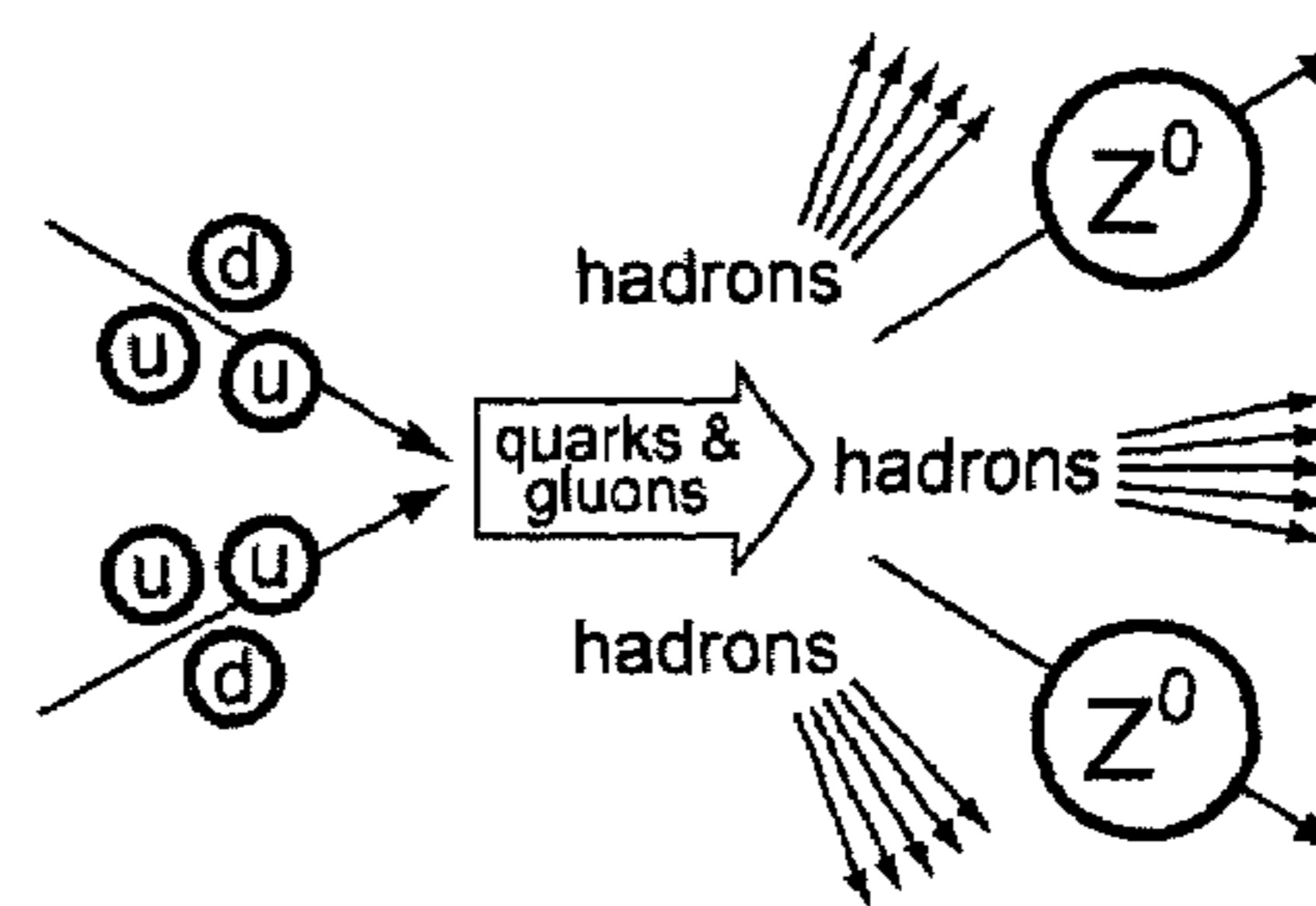
Two protons colliding at high energy can produce various hadrons plus very high mass particles such as Z bosons. Events such as this one are rare but can yield vital clues to the structure of matter.
