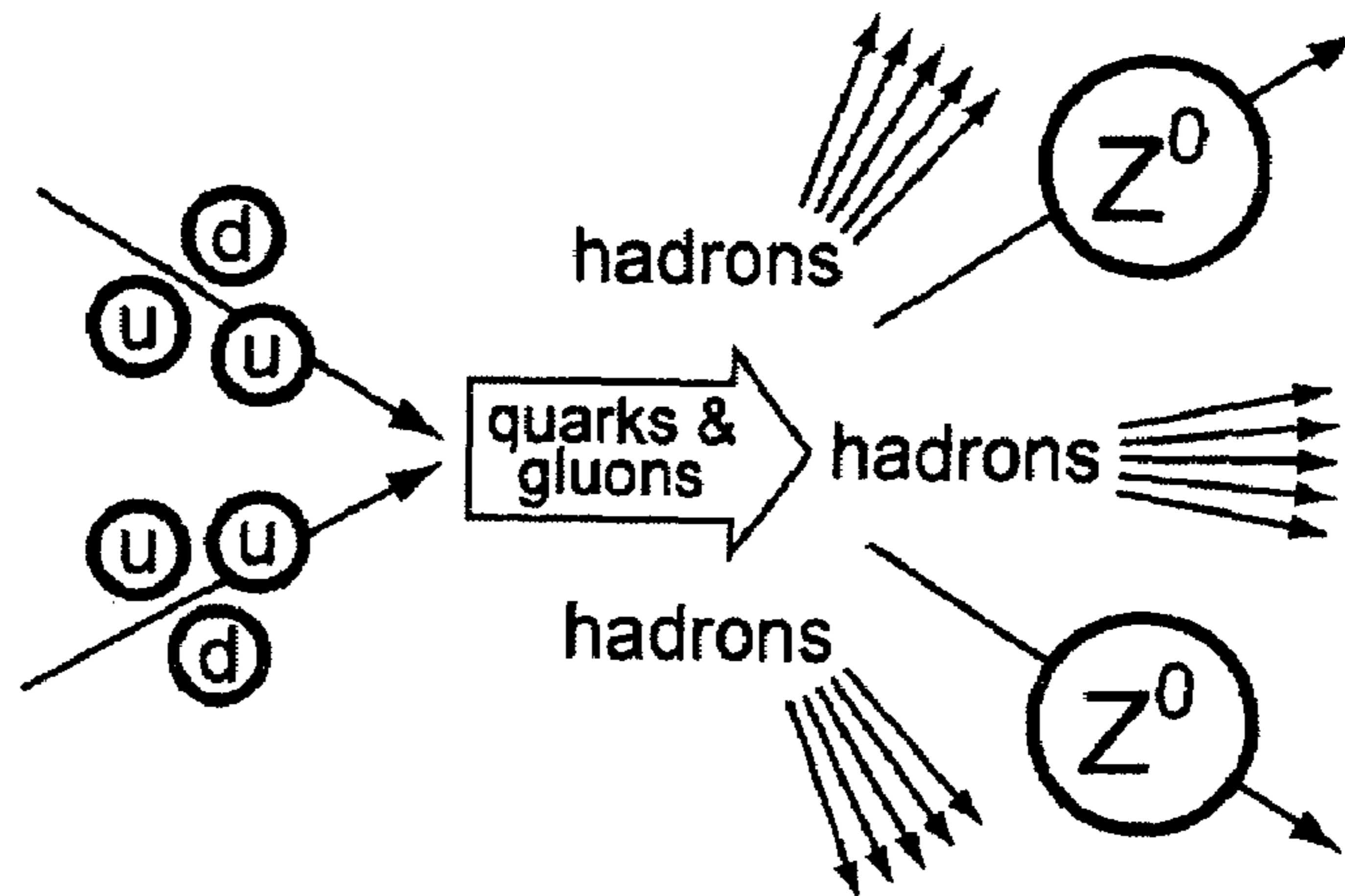
Two protons colliding at high energy can produce various hadrons plus very high mass particles such as Z bosons. Events such as this one are rare but can yield vital clues to the structure of matter.
