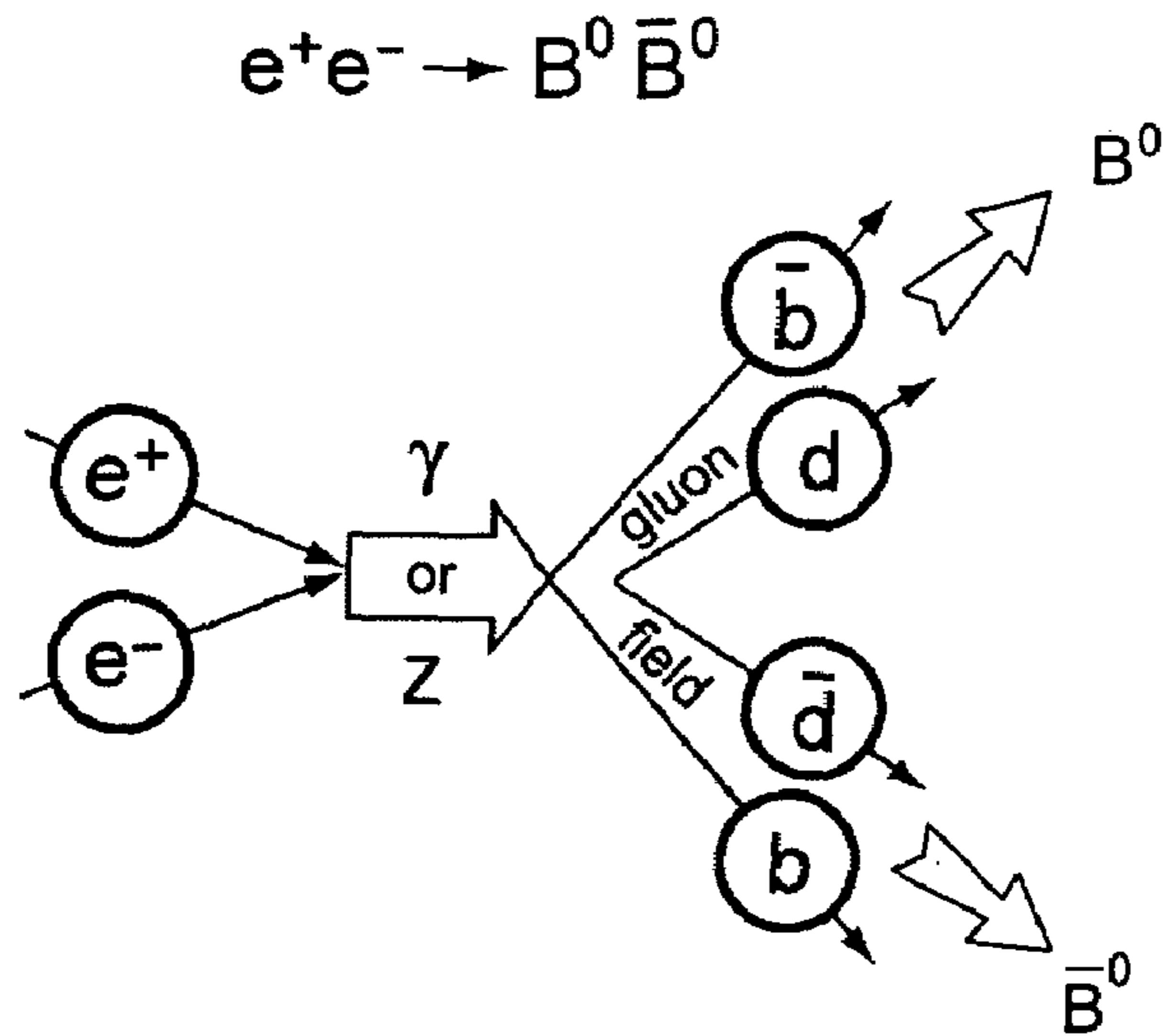
An electron and positron (antielectron) colliding at high energy, can annihilate to produce B^0 and \bar{B}^0 mesons via a virtual Z boson or a virtual photon.
