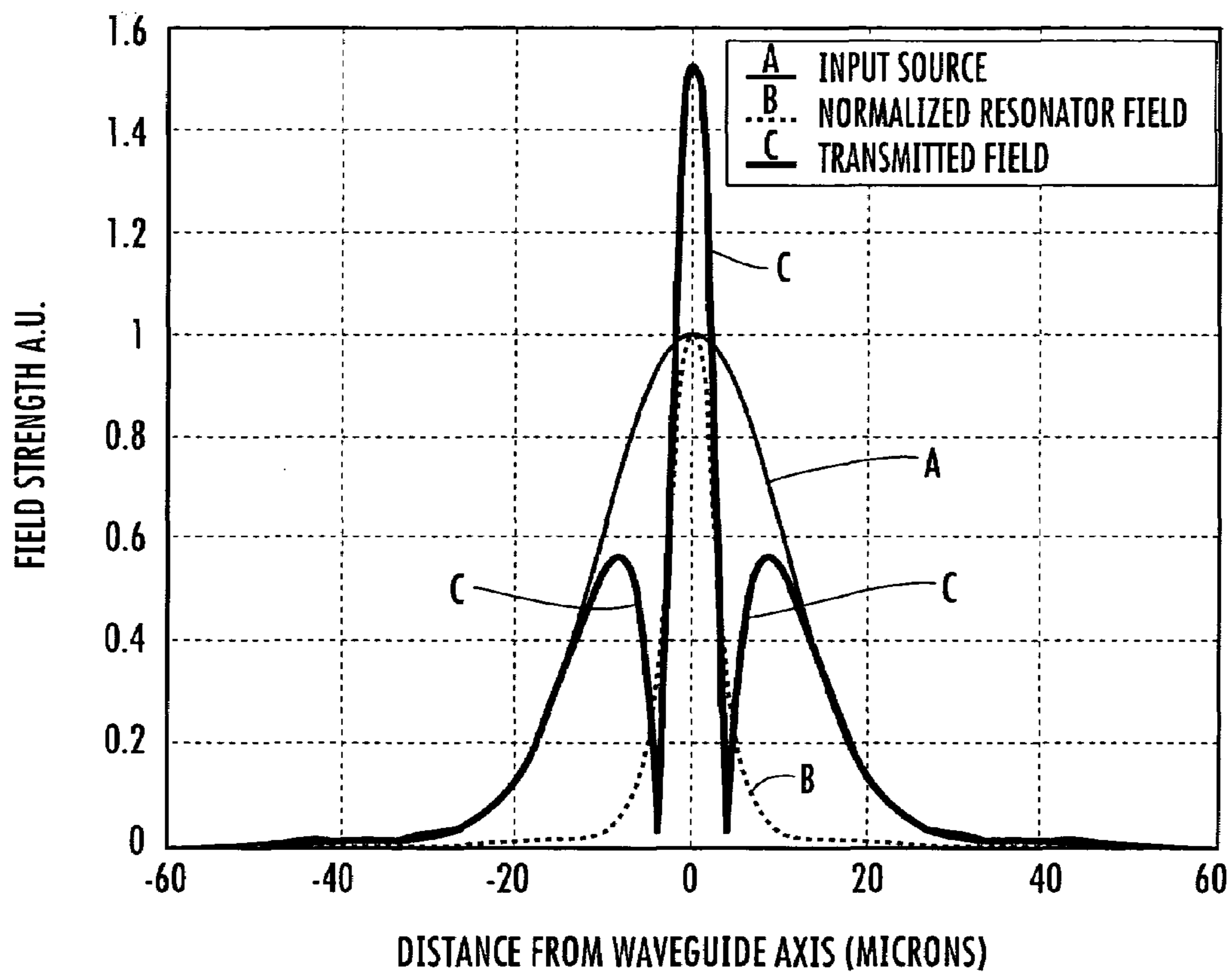
STEADY STATE FIELD PATTERNS
