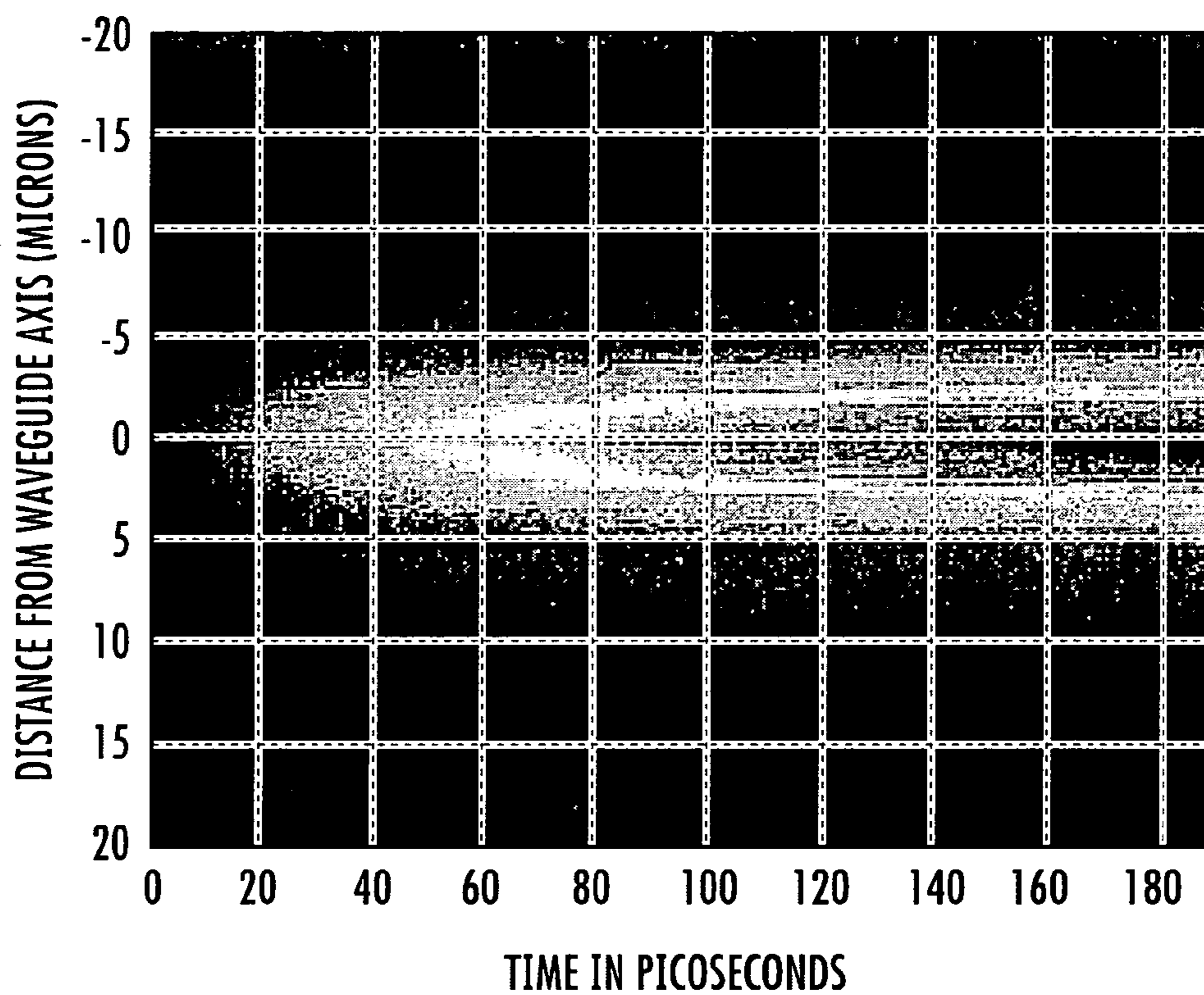
TRANSIENT FIELD PATTERNS IN RESONATOR GUIDE
