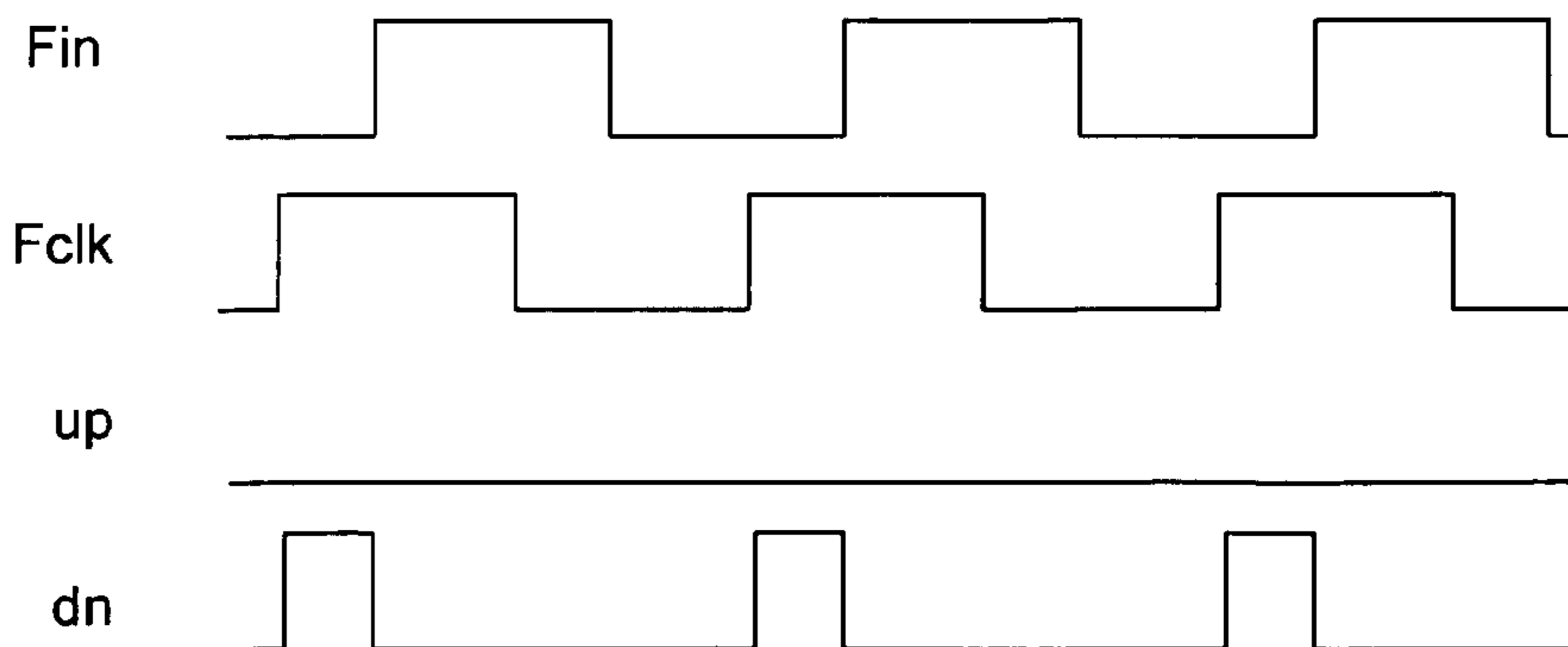
Fig. 2B (Conventional)
