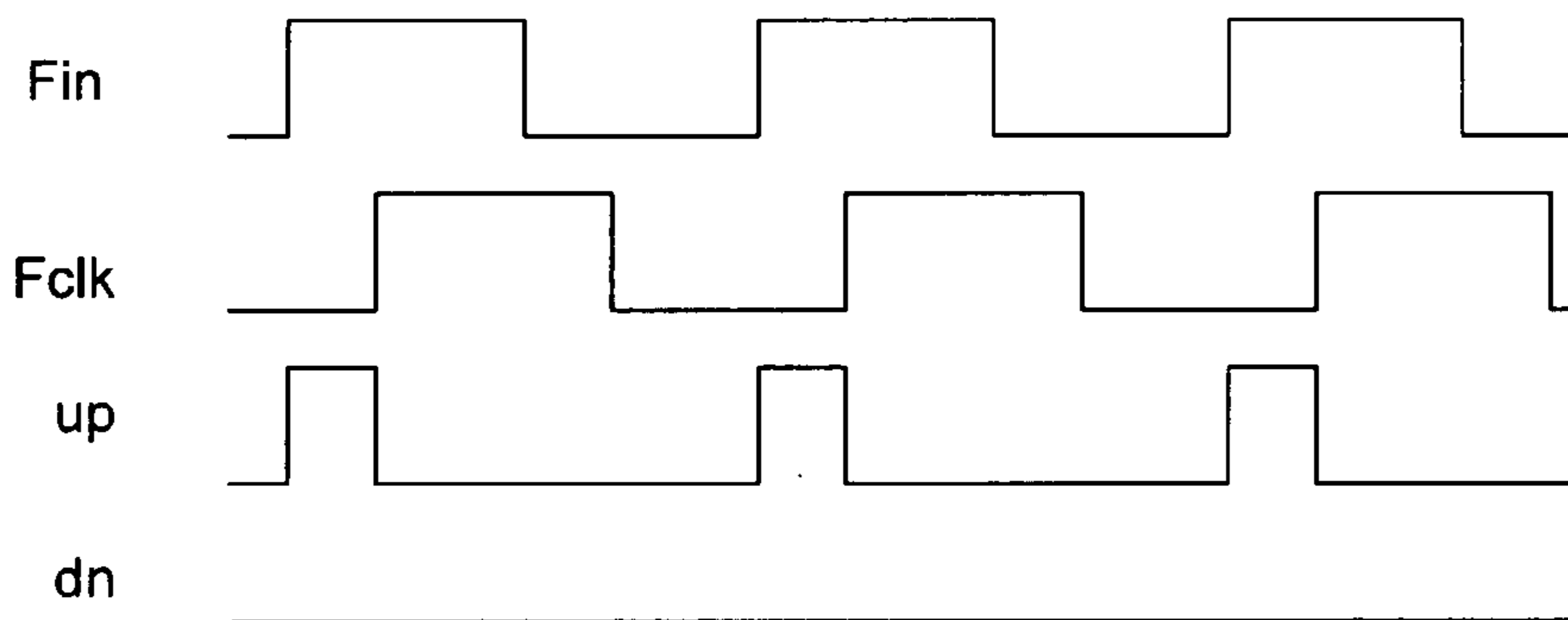
Fig. 2A (Conventional)
