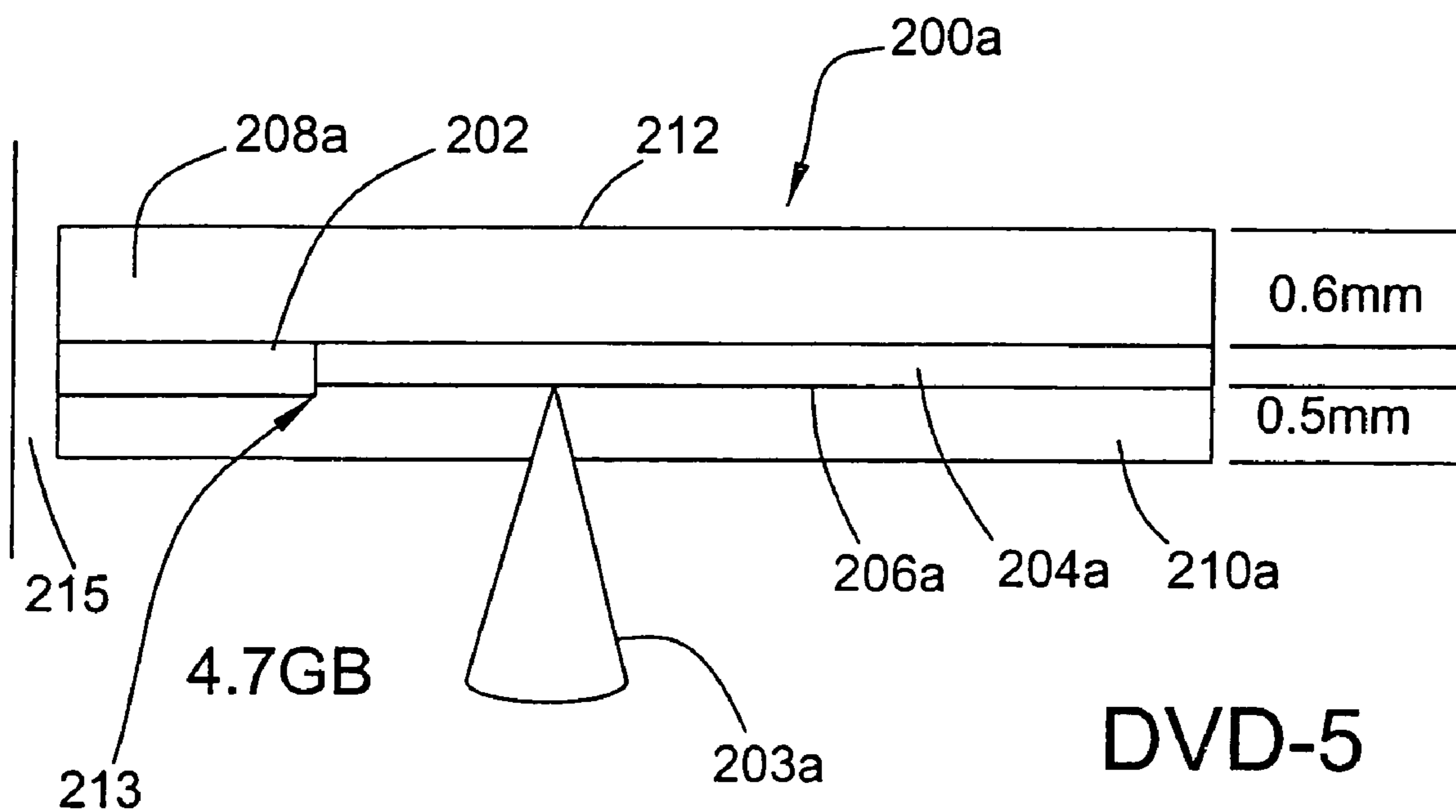
FIG. 2A Single-Sided, Single Layer Disc
