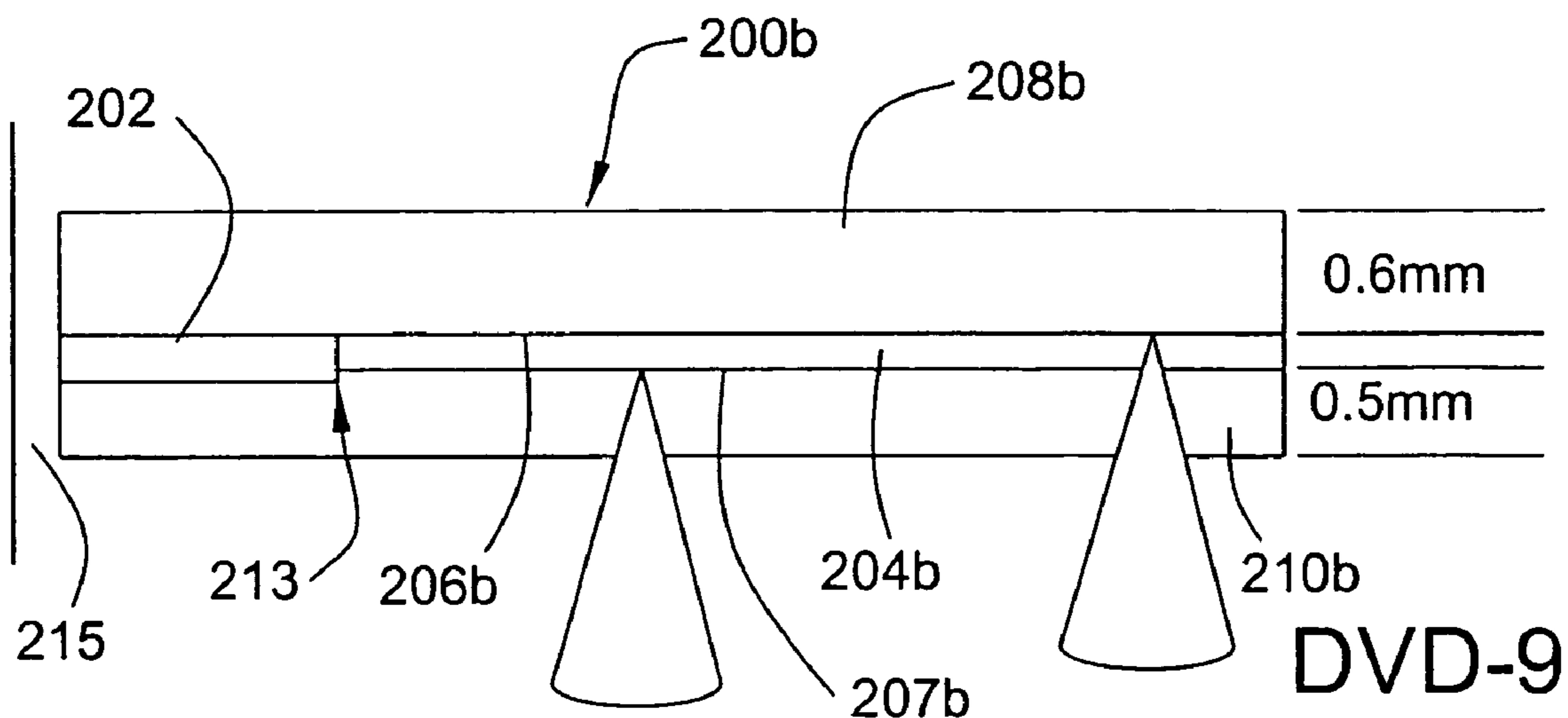
Single-Sided Double Layer Disc
