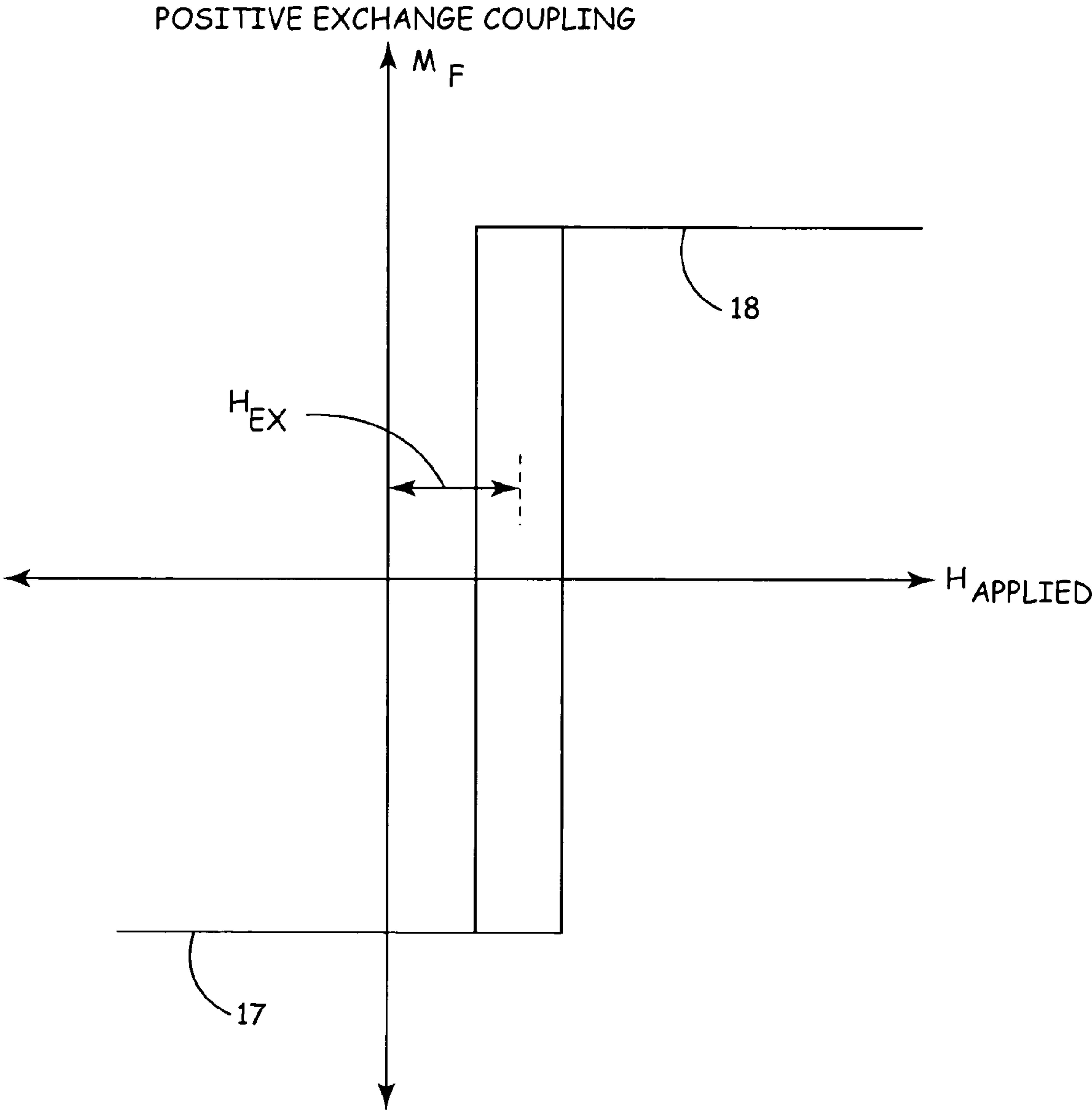
FIG. 3 PRIOR ART
