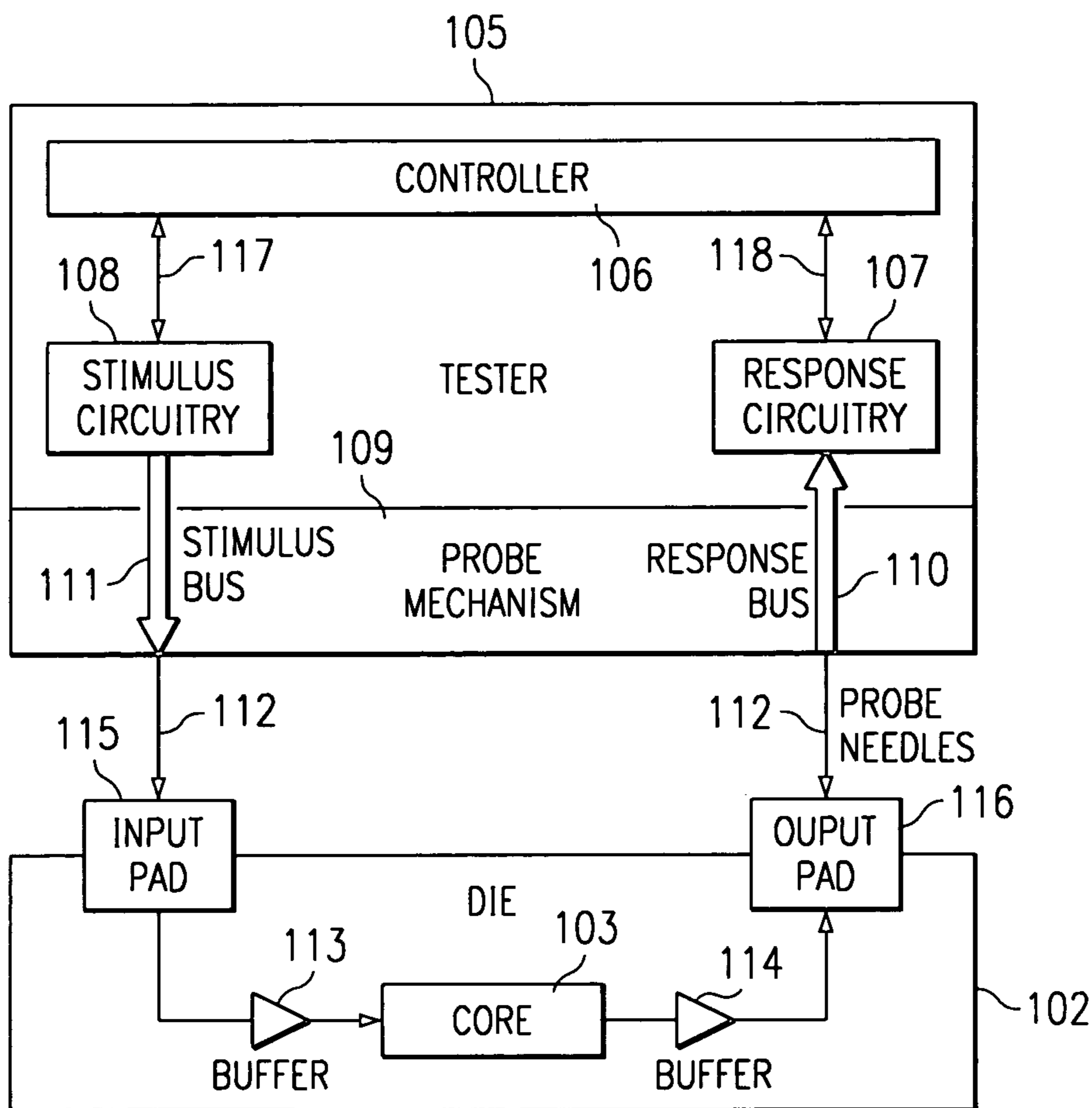
FIG. 1C (PRIOR ART)
