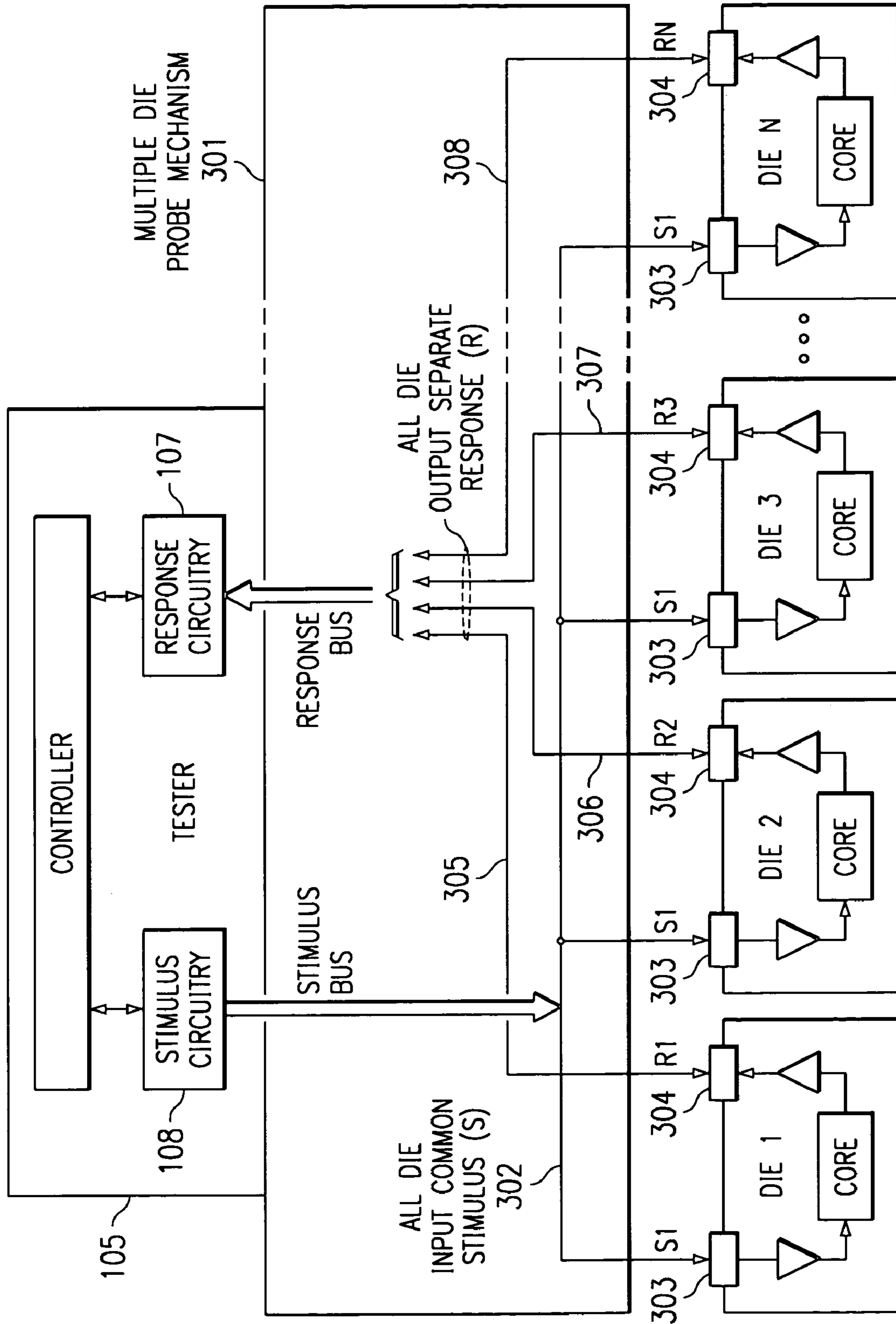
FIG. 3 (PRIOR ART)
