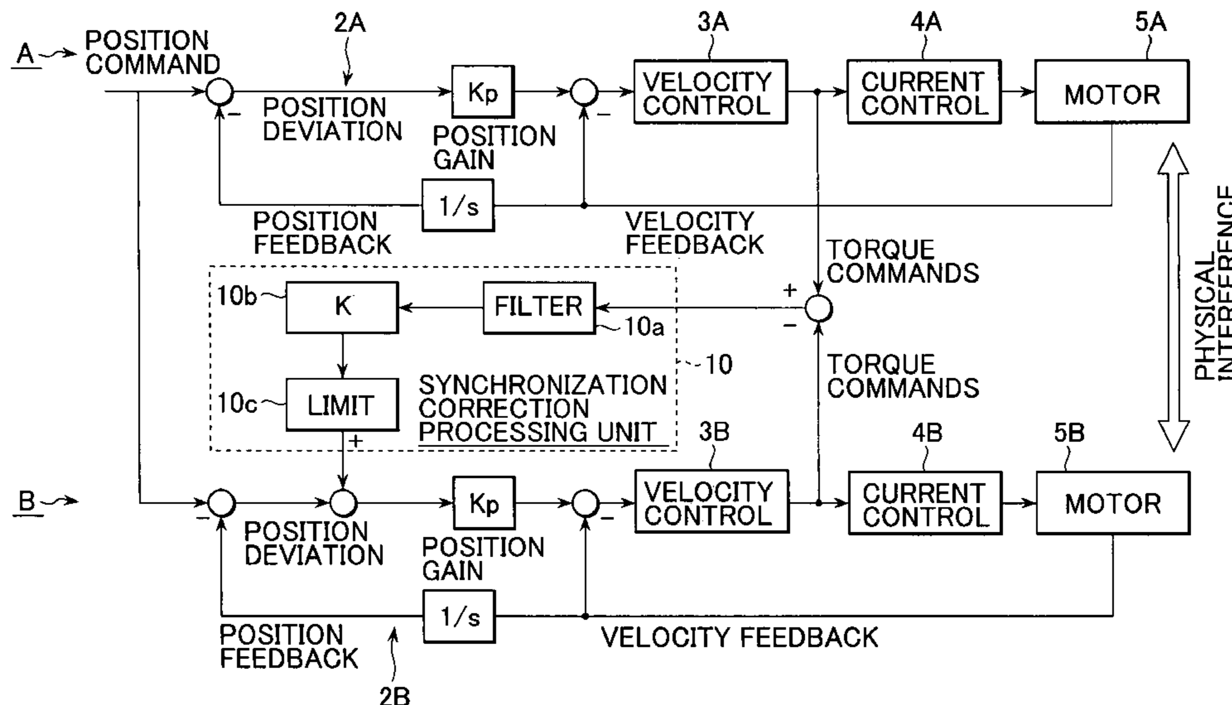
CALCULATION OF POSITION DEVIATION OFFSET FROM THE DIFFERENCE IN TORQUE COMMANDS
