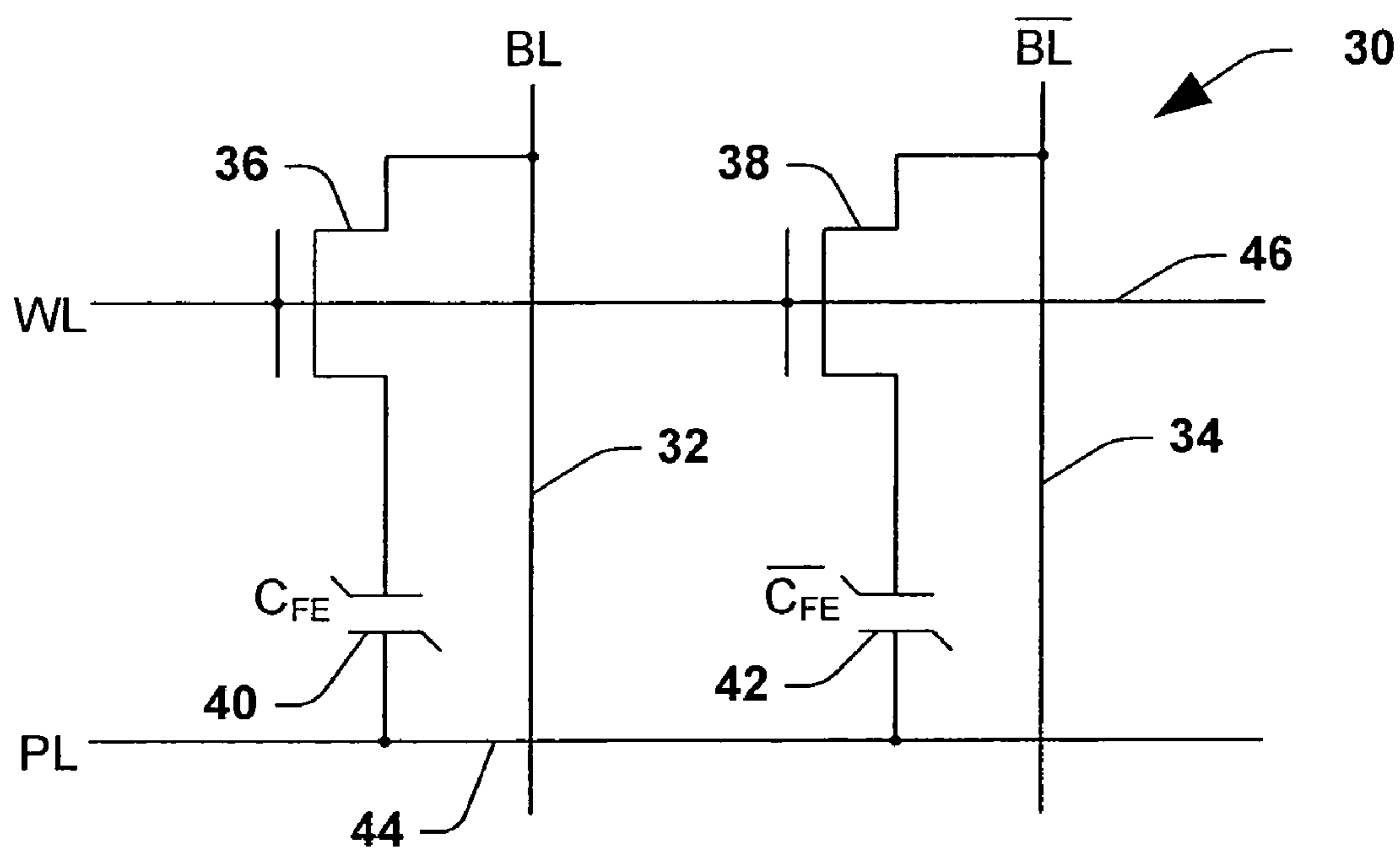
FIG. 2 (PRIOR ART)
