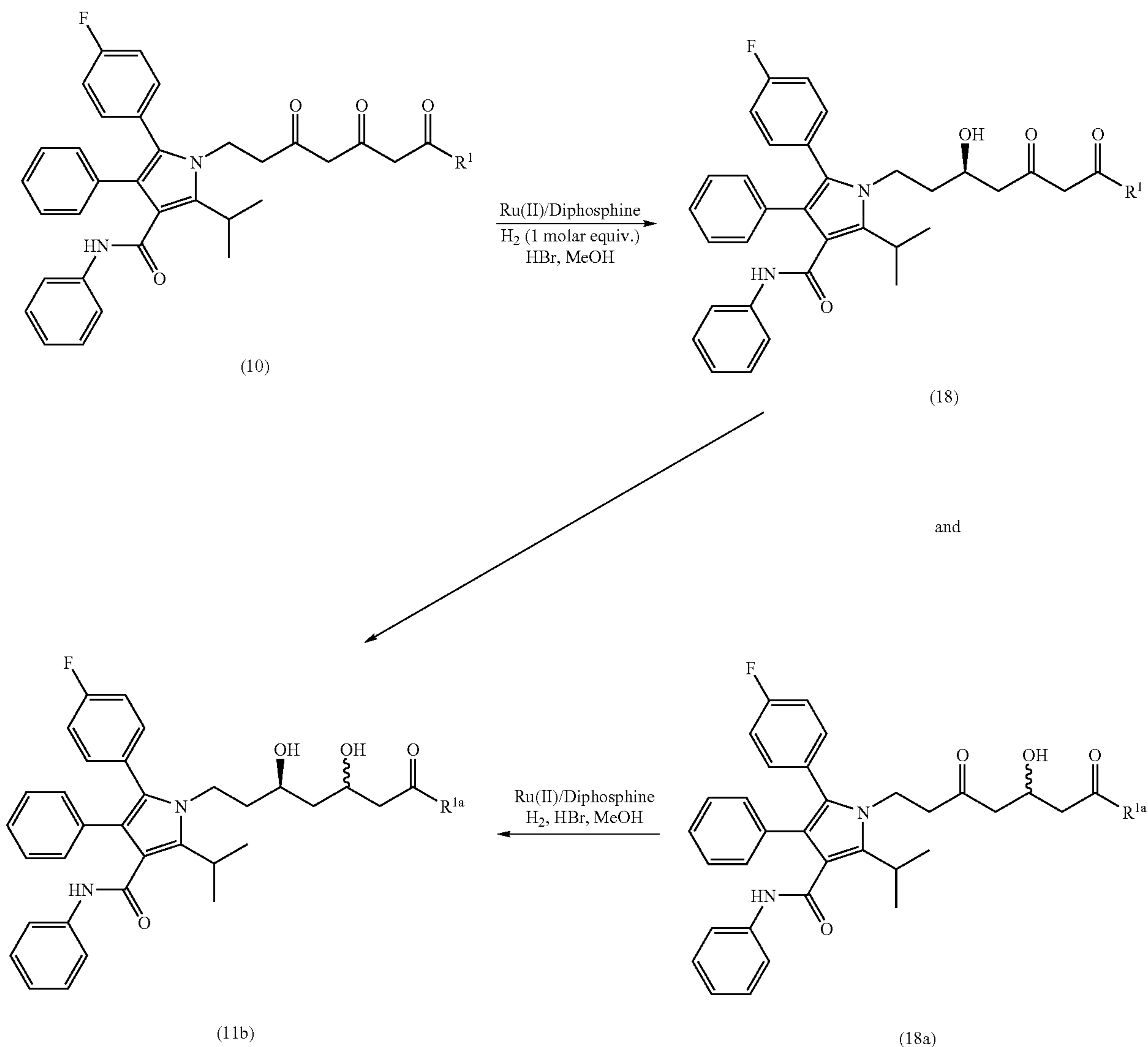
Scheme 4
