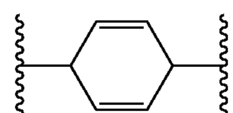
(2,5-cyclohexadien-1,4-ylene)
