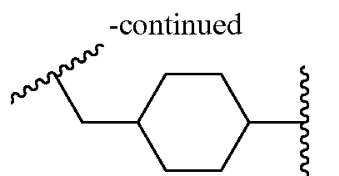
(methylene-cyclohex-1,4-ylene)
