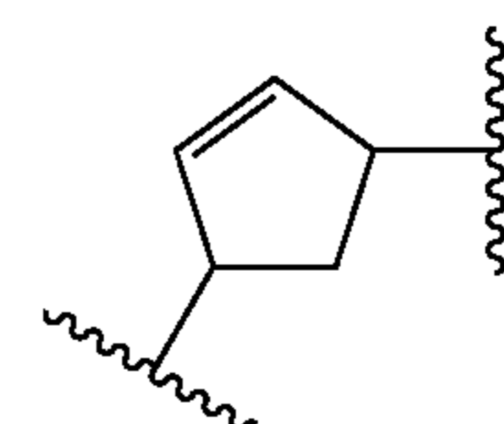
(4-cyclopenten-1,3-ylene)
