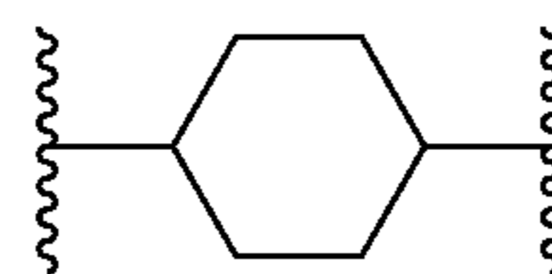
(cyclohex-1,4-ylene)
