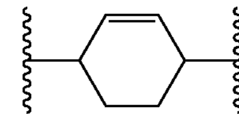
(2-cyclohexen-1,4-ylene)
