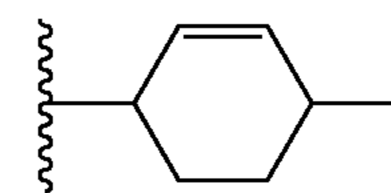
(2-cyclohexen-1,4-ylene)
