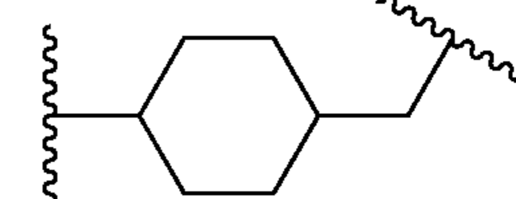
(cyclohex-1,4-ylene-methylene)
