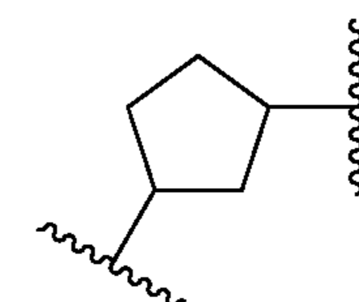
(cyclopent-1,3-ylene)
