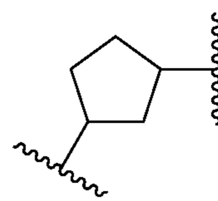
(cyclopent-1,3-ylene)
