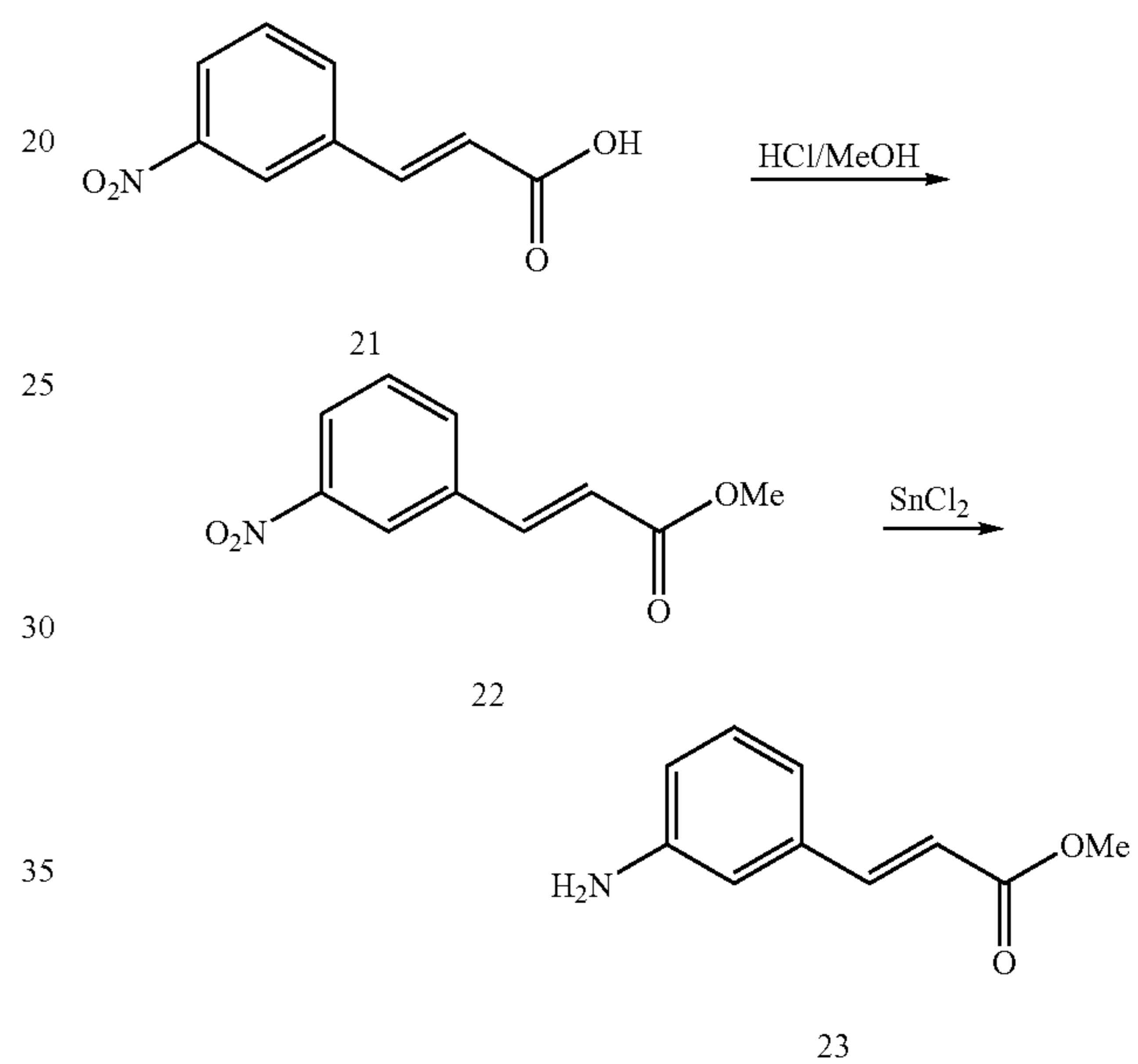
Scheme 3A
