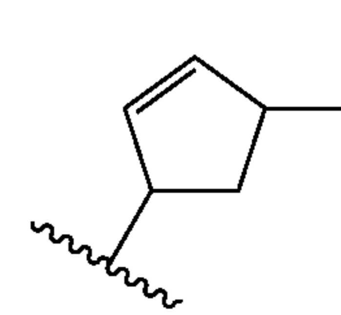
(4-cyclopenten-1,3-ylene)
