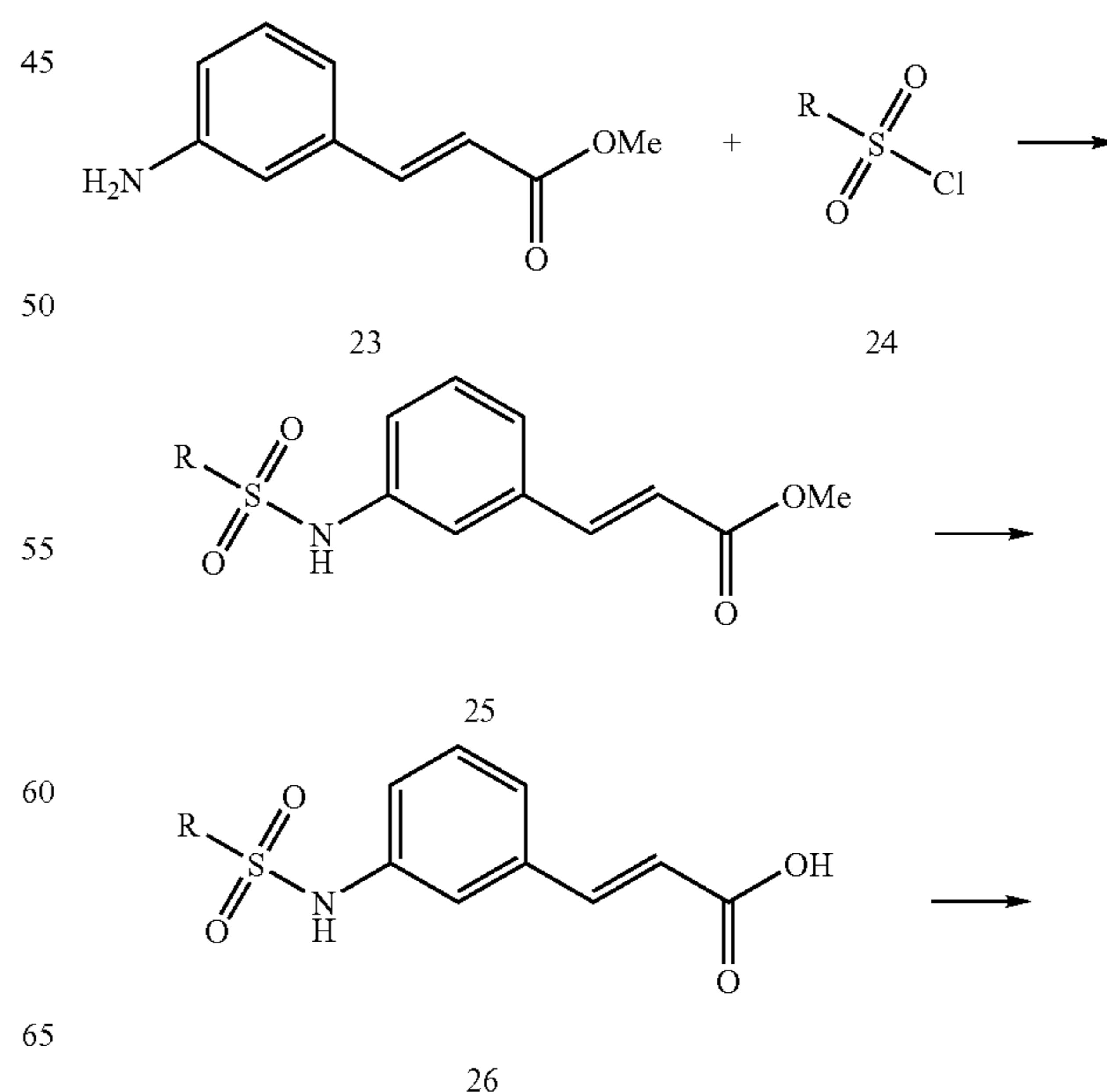
Scheme 3B
