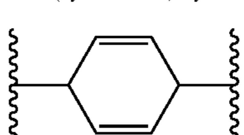
(cyclohex-1,4-ylene)
