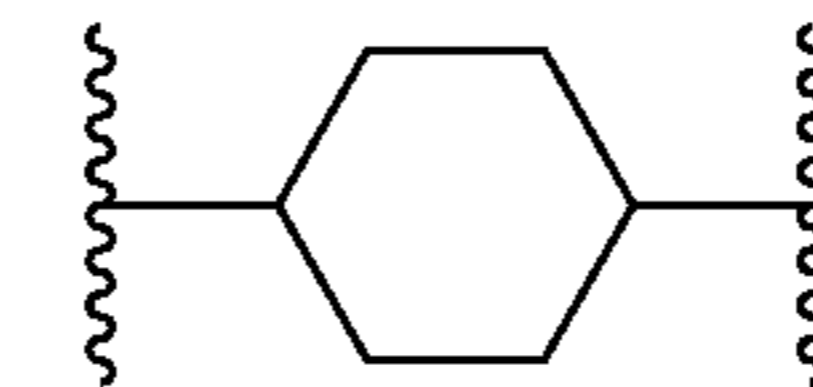
(cyclohex-1,4-ylene)
