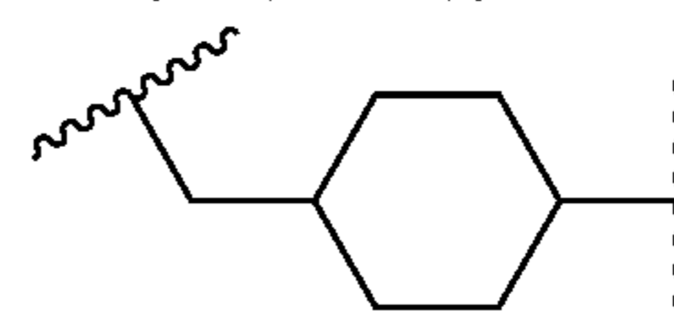
(methylene-cyclohex-1,4-ylene)
