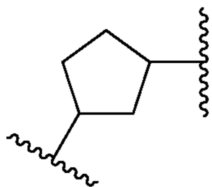
(cyclopent-1,3-ylene)
