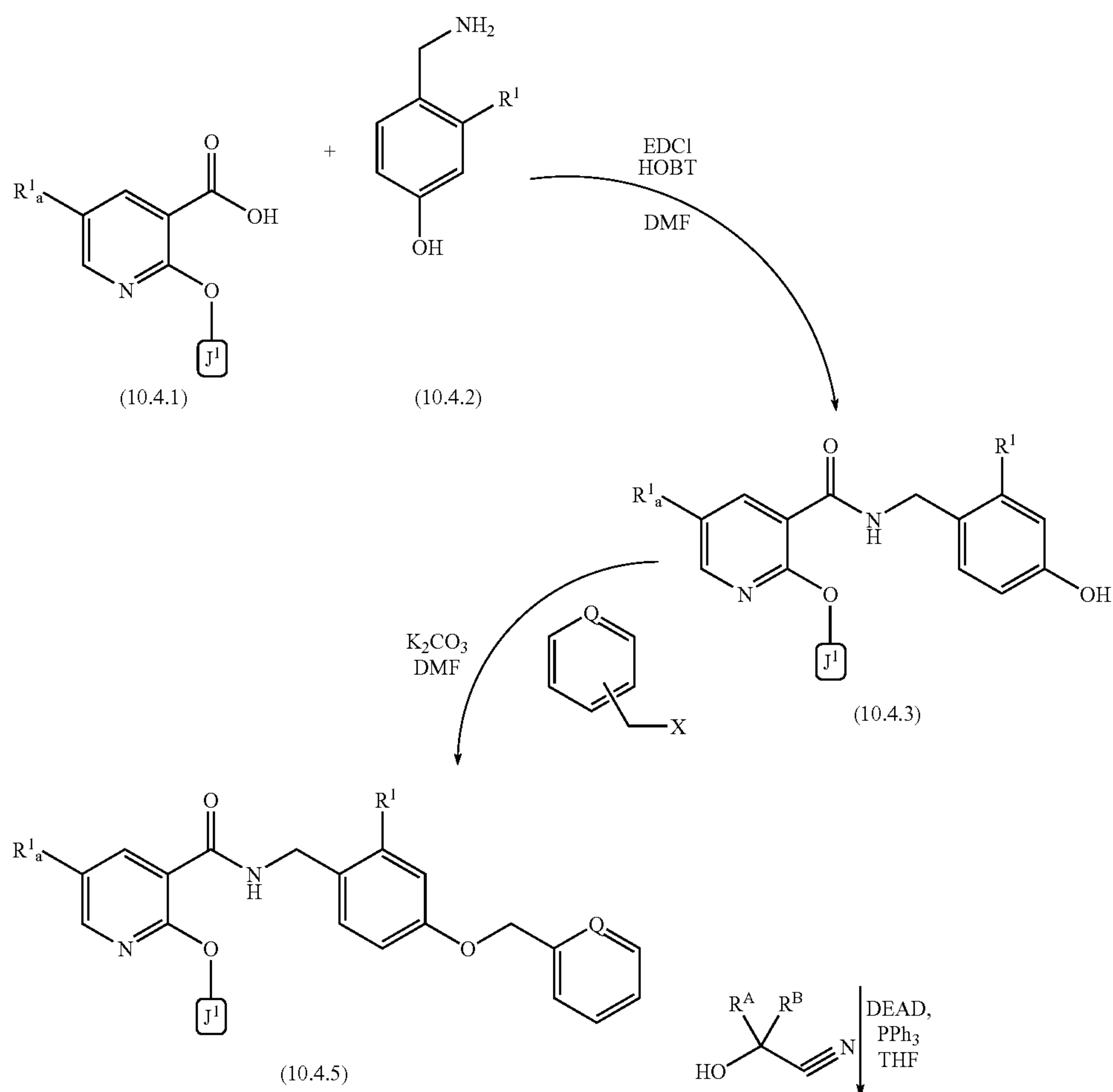
SYNTHESIS SCHEME (10.4.0)
