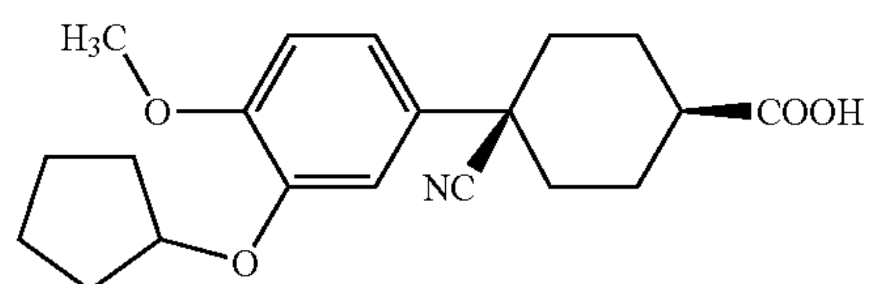
ARIFLO® cis-[4-cyano-4-(3-cyclopentyl-oxy-4-methoxyphenyl)cyclo-hexane-1-carboxylic acid]
