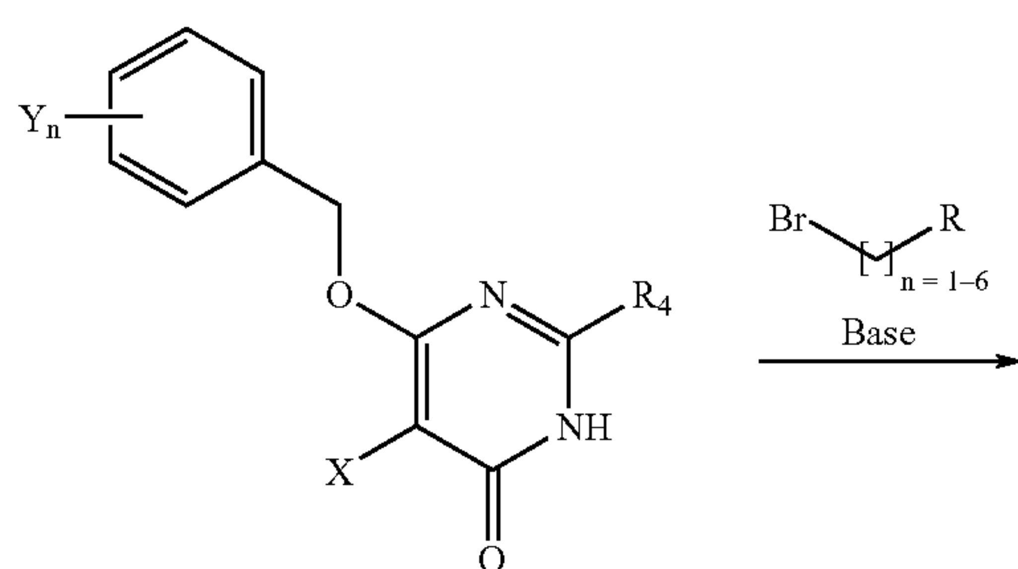
Scheme 9
