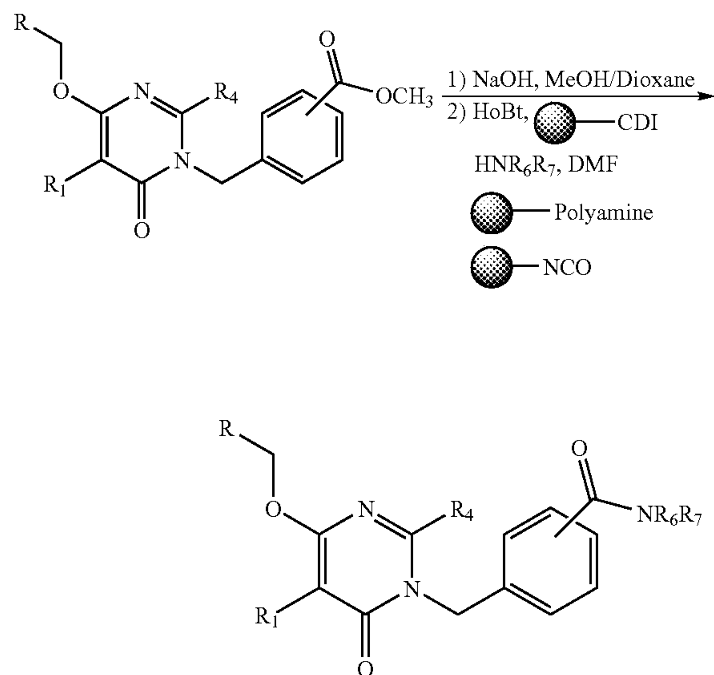
Scheme 13
