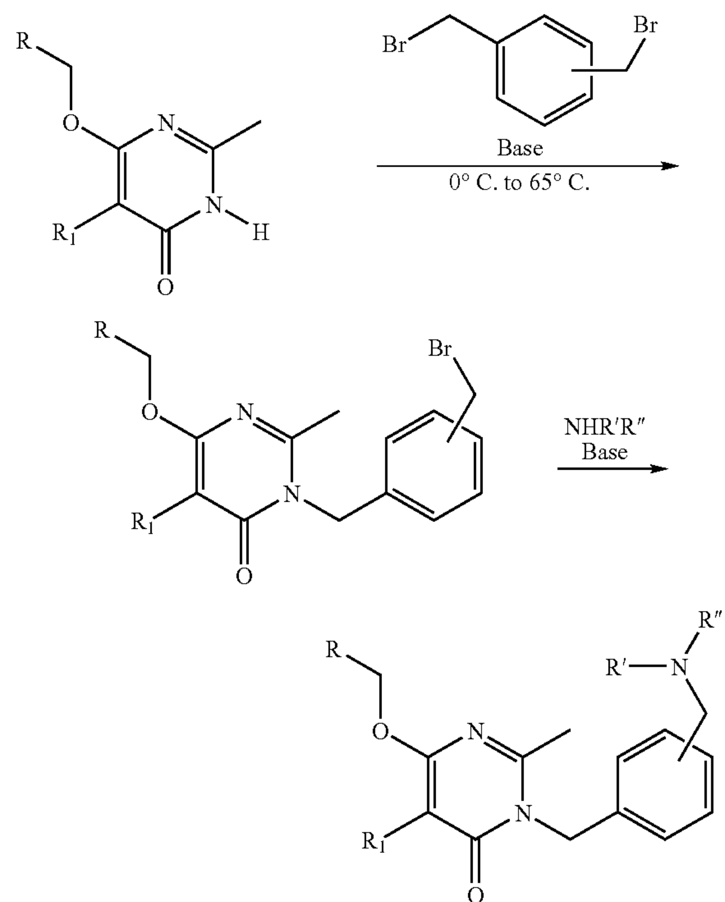
Scheme 20
