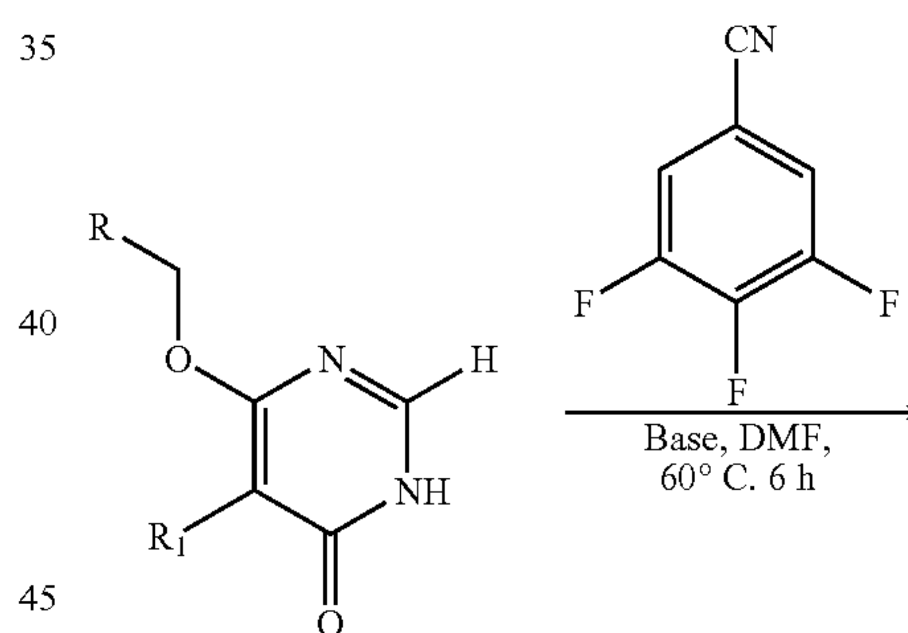
Scheme 12
