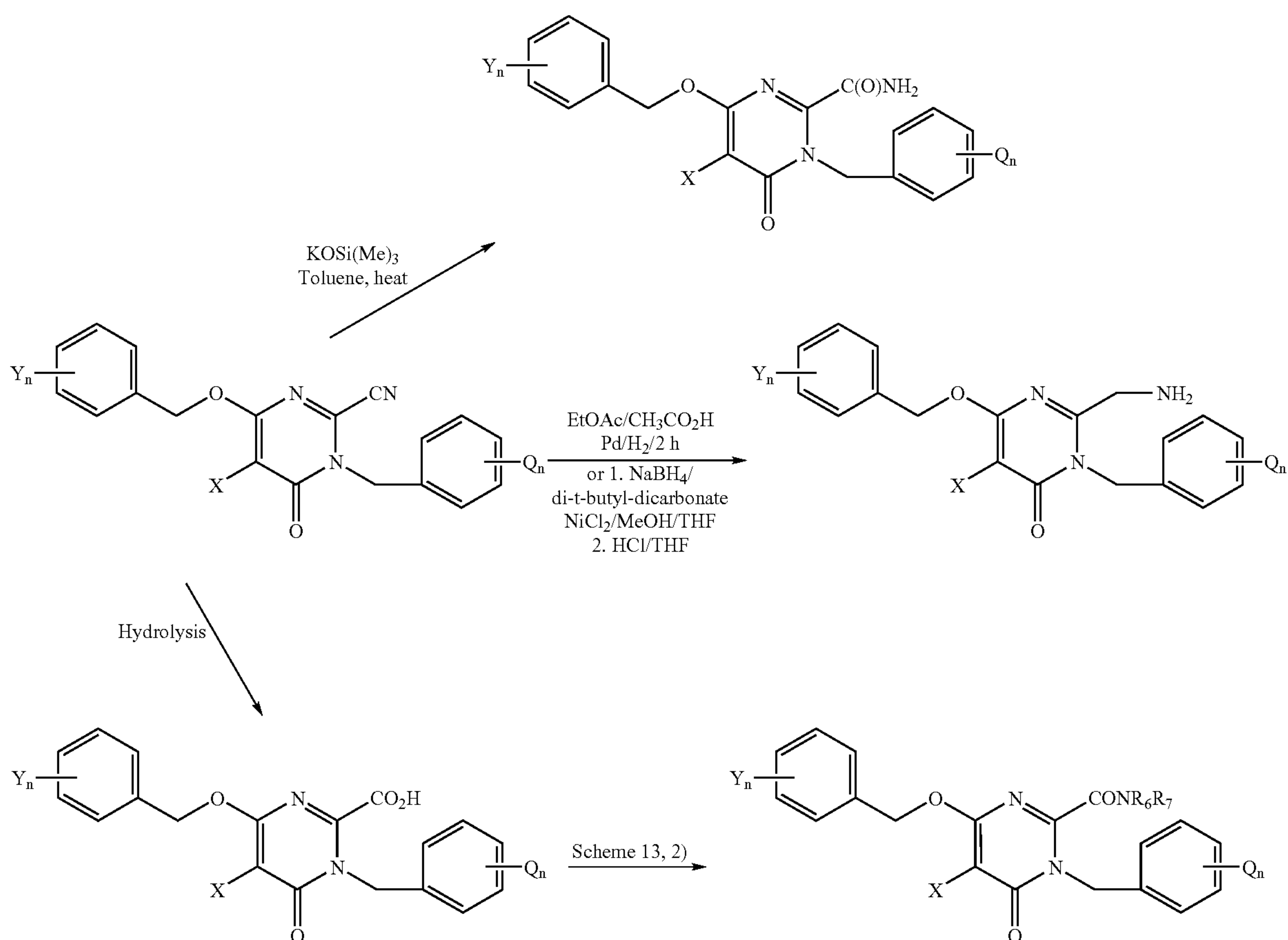
Scheme 8
