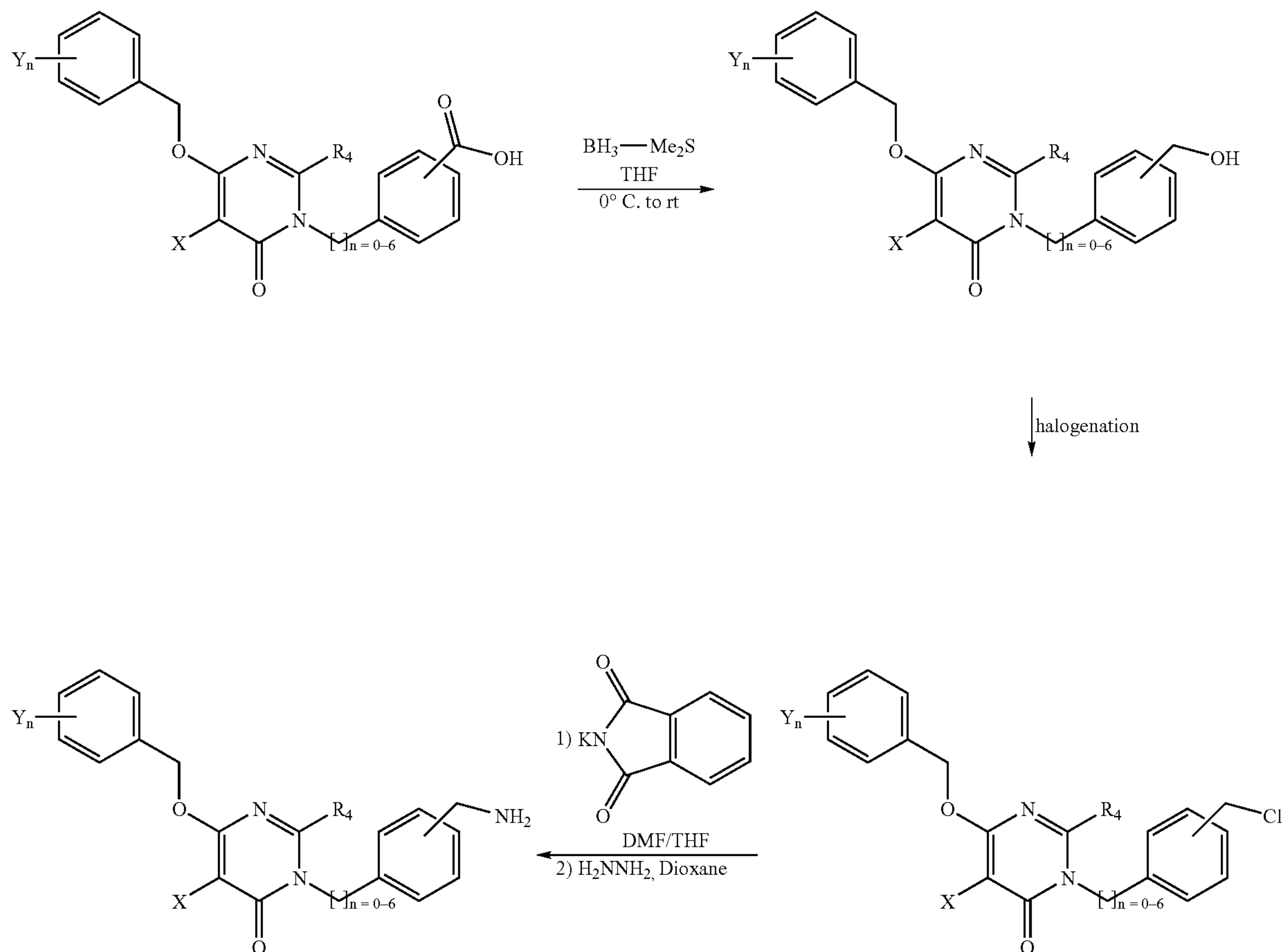
Scheme 14
