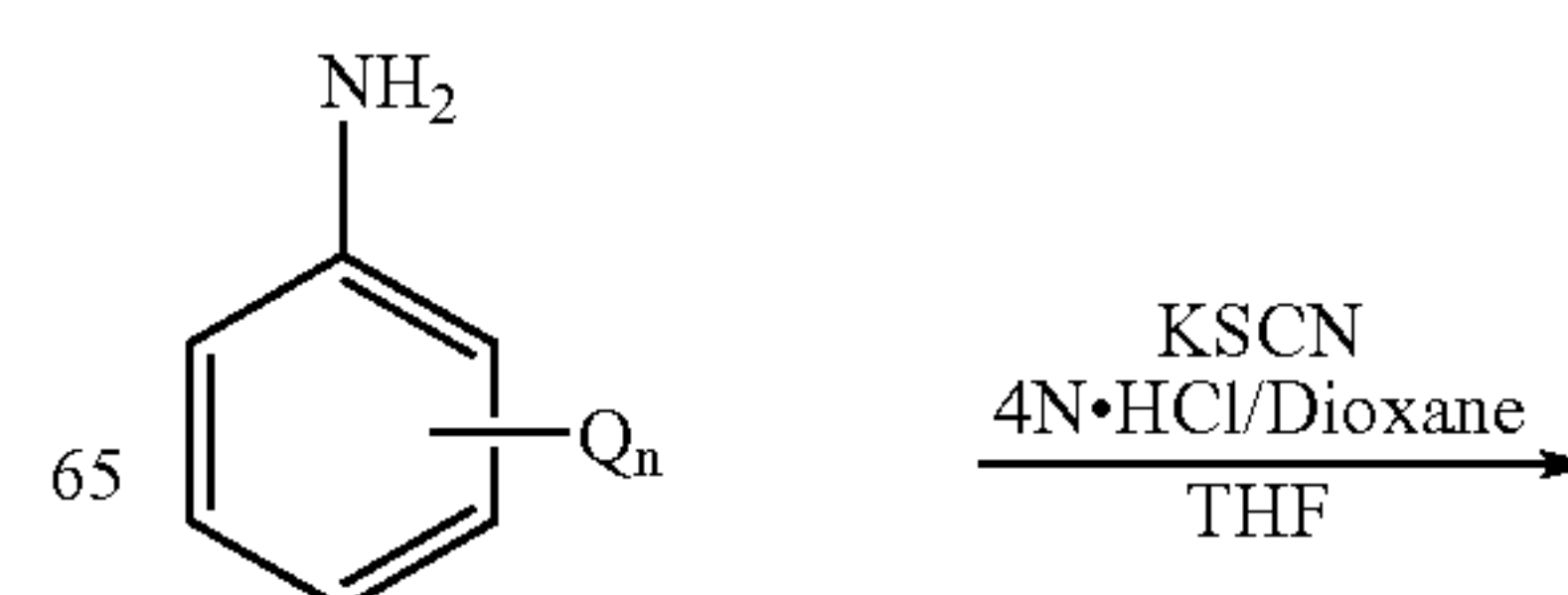
Scheme 23
