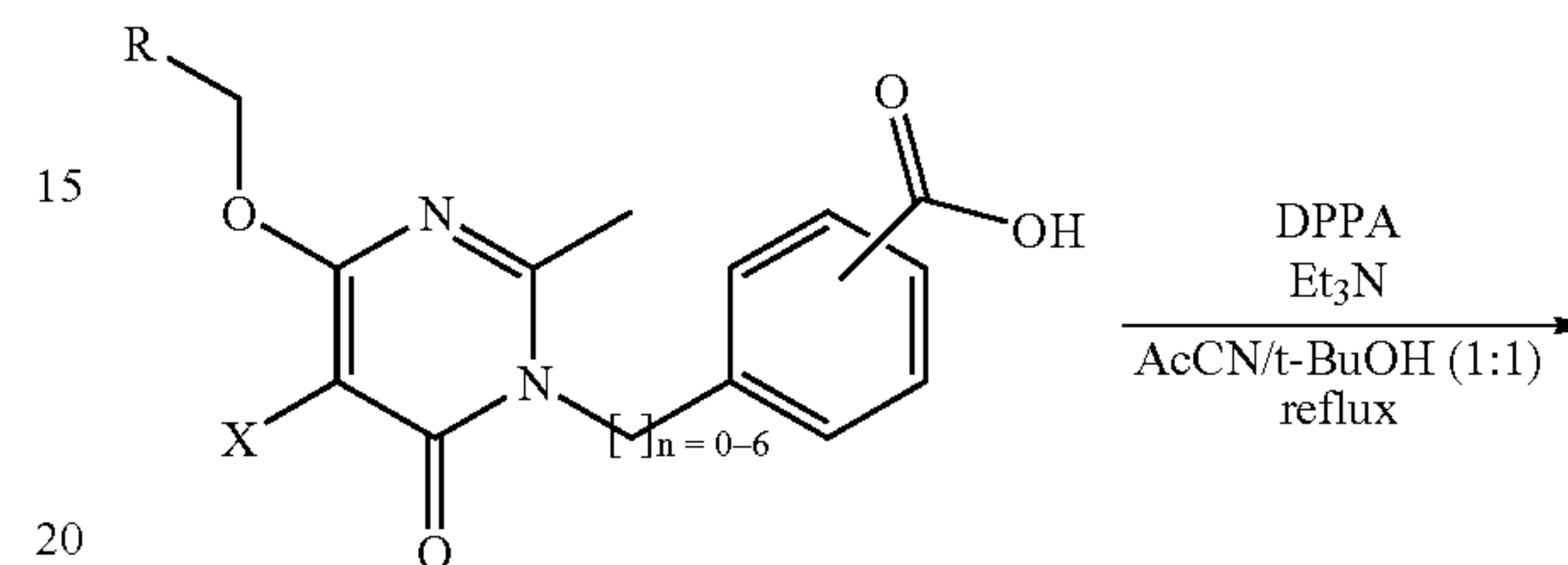
Scheme 15
