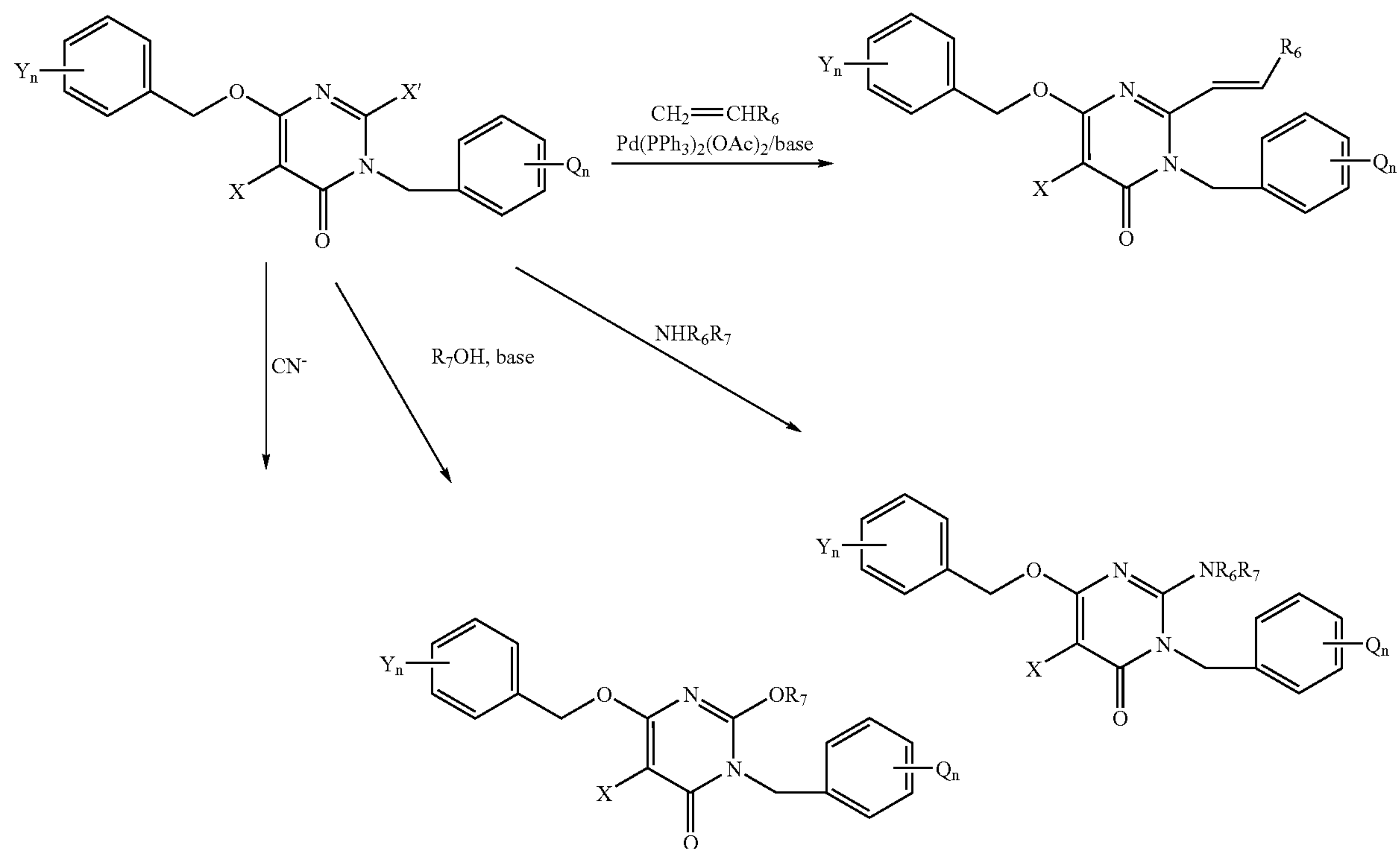
Scheme 7
