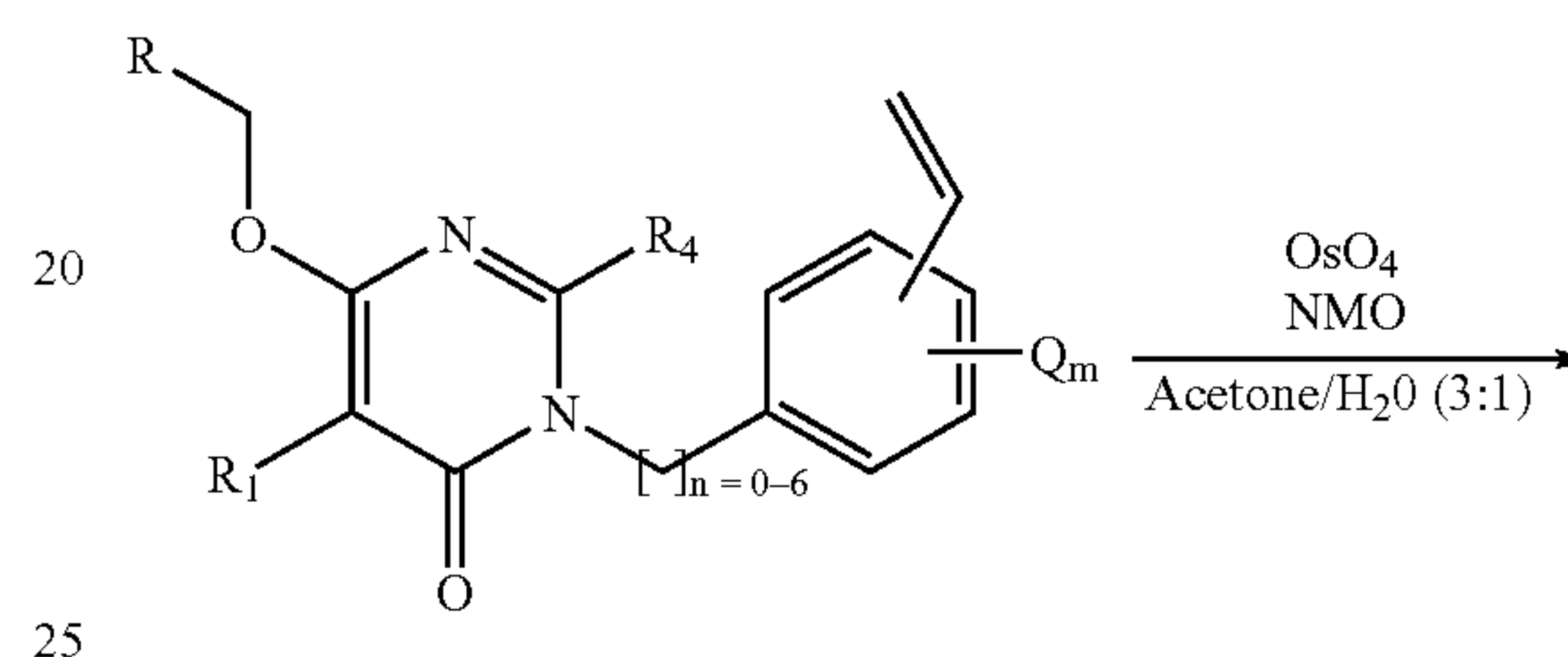
Scheme 17
