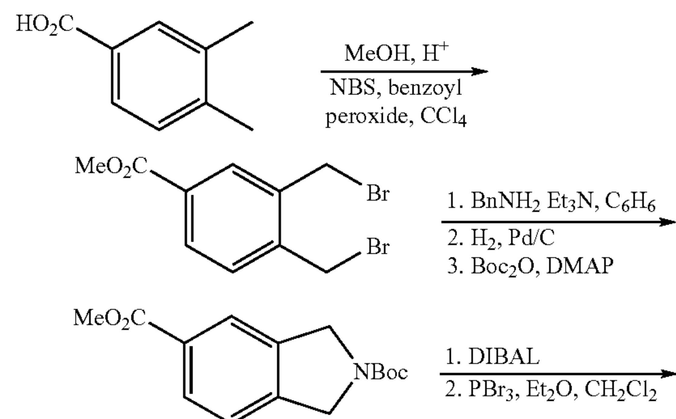
Scheme 21
