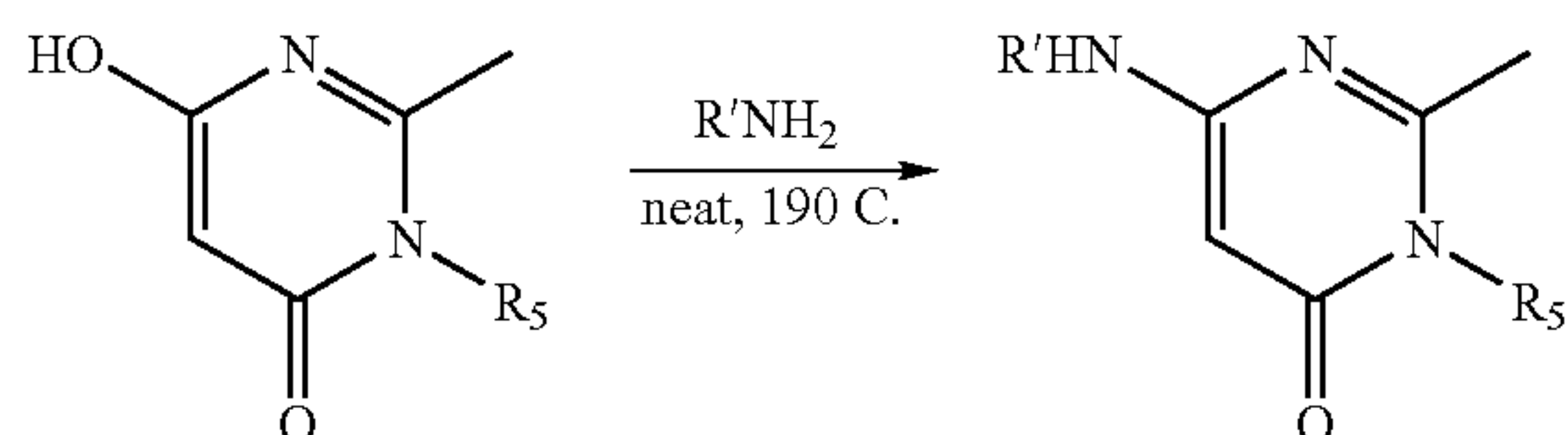
Scheme 19
