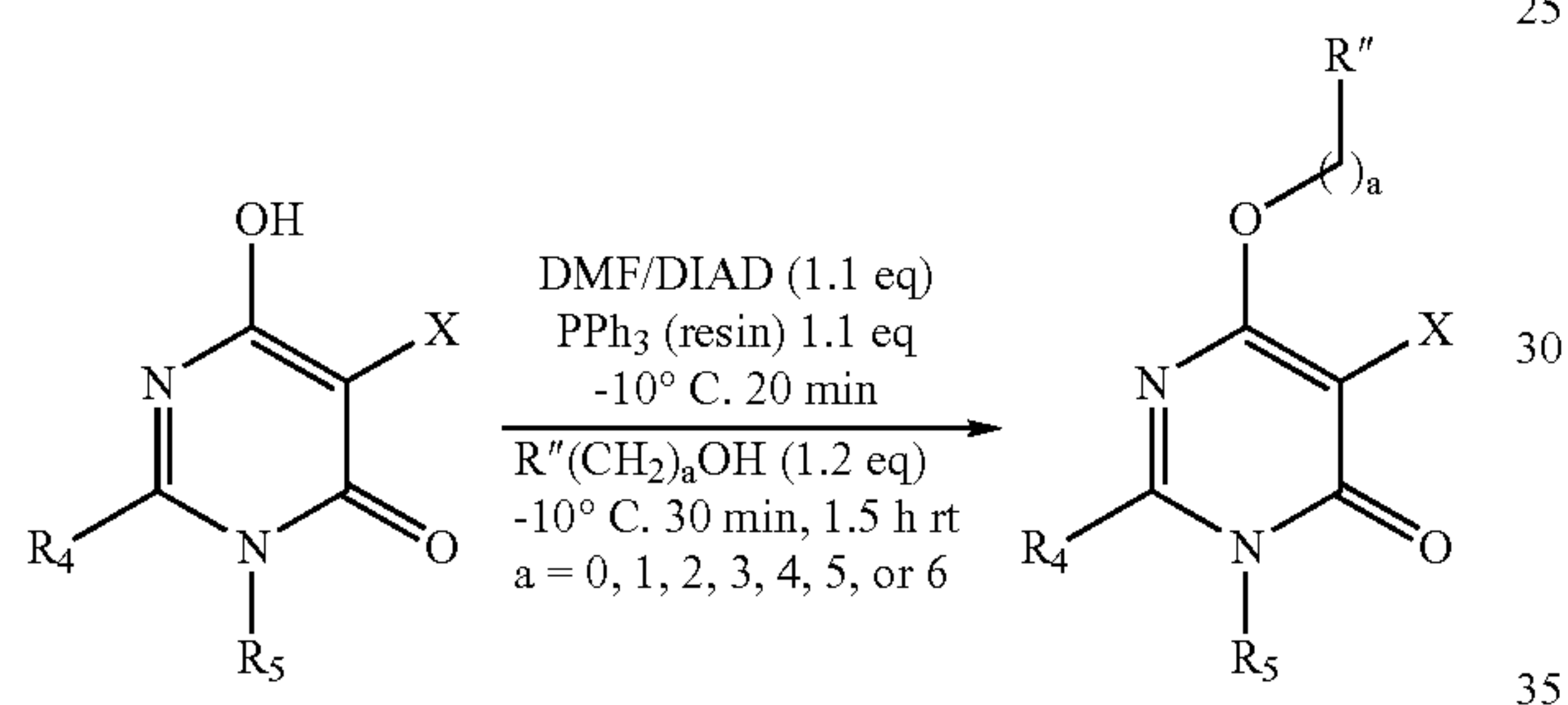
Scheme 10
