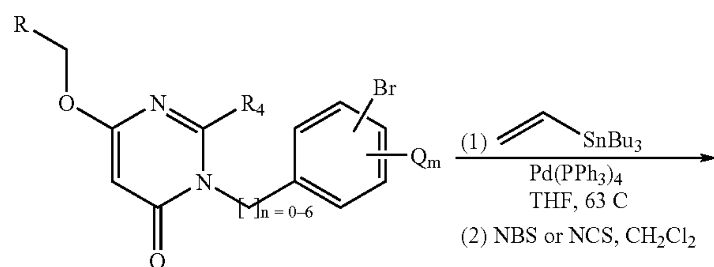
Scheme 16
