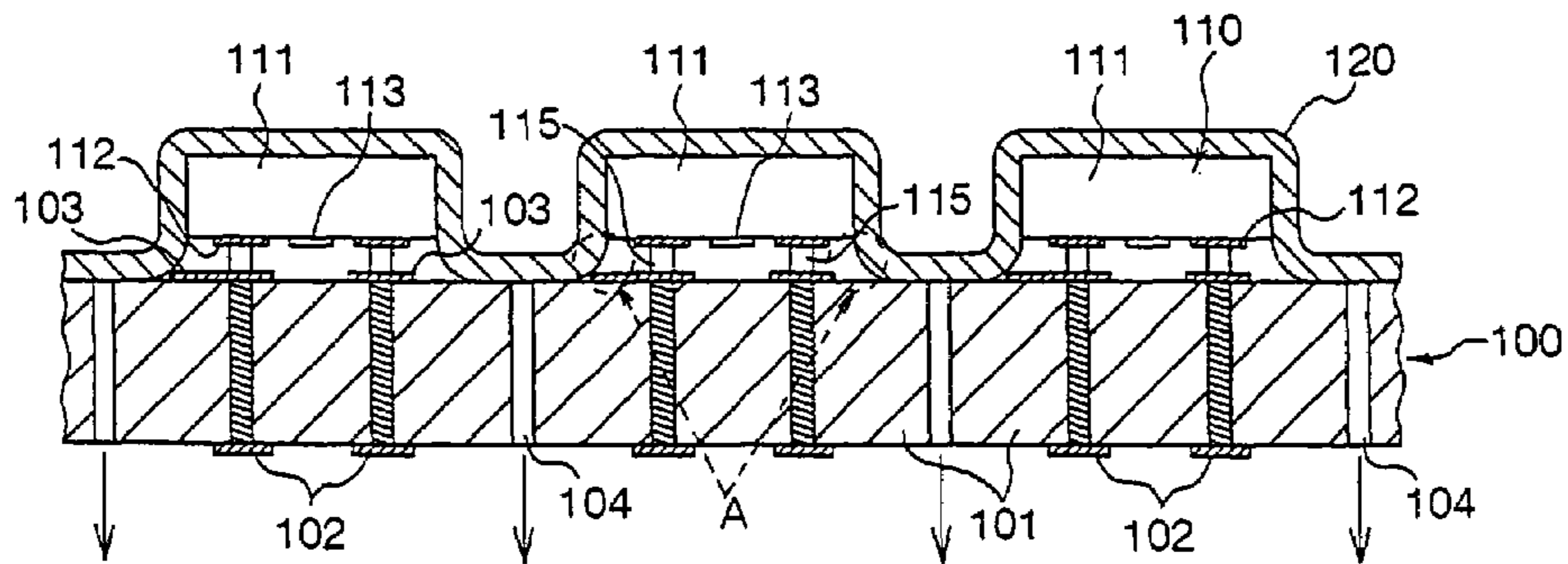
Fig. 10 PRIOR ART
