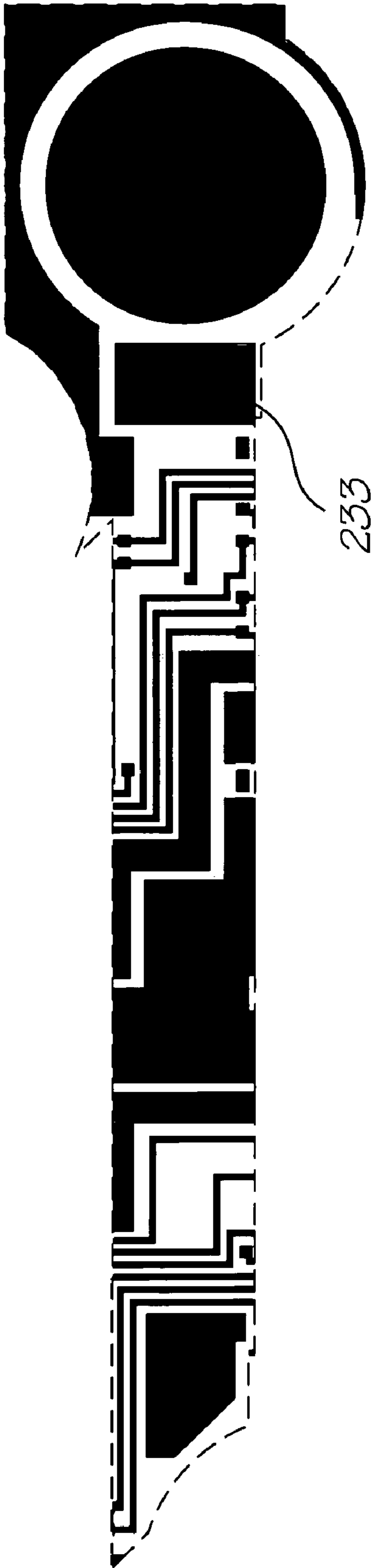
Metal 2 mask
