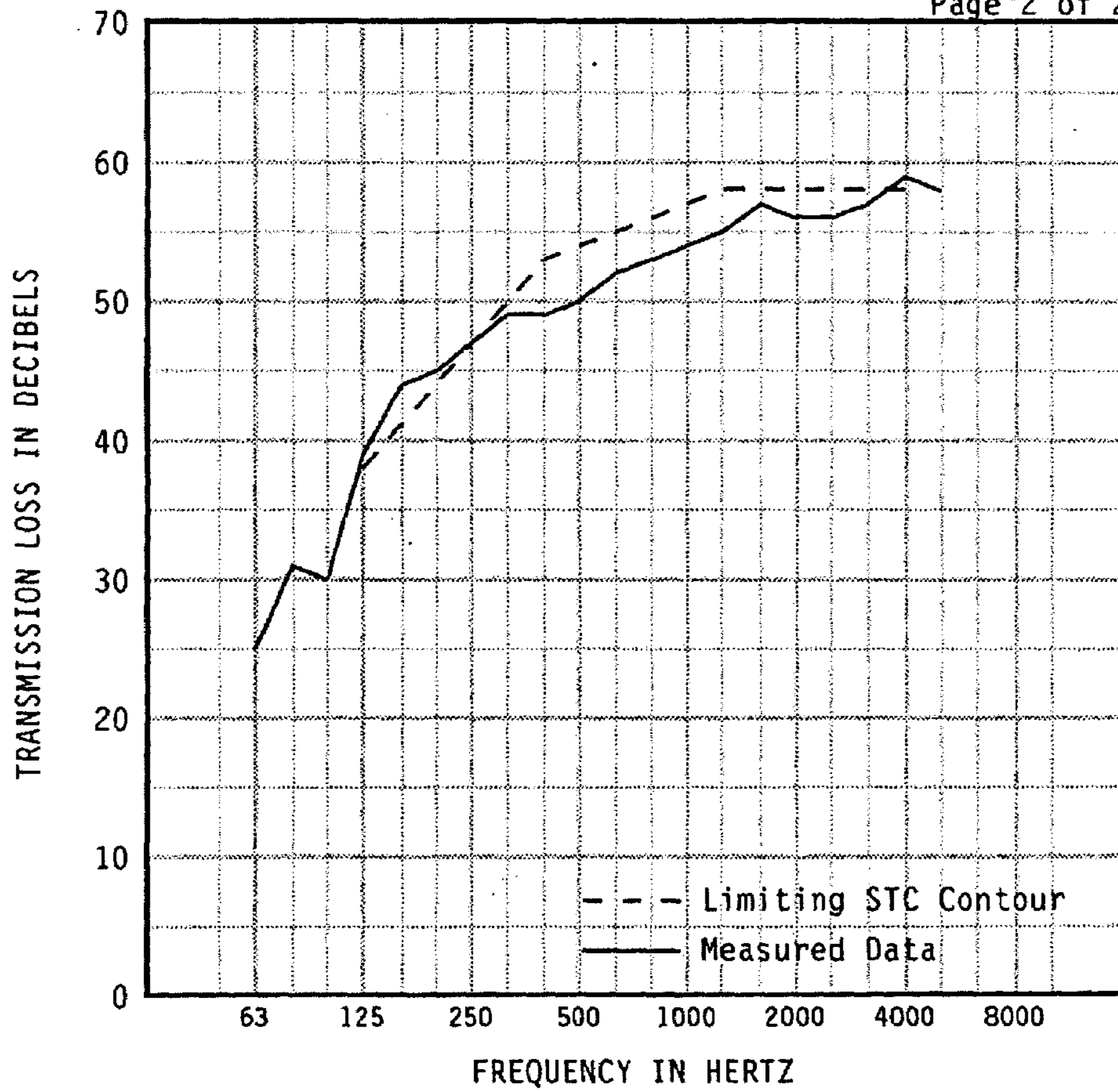
Standard 2x4 Construction with QuietRock Ultra both sides no insulation
