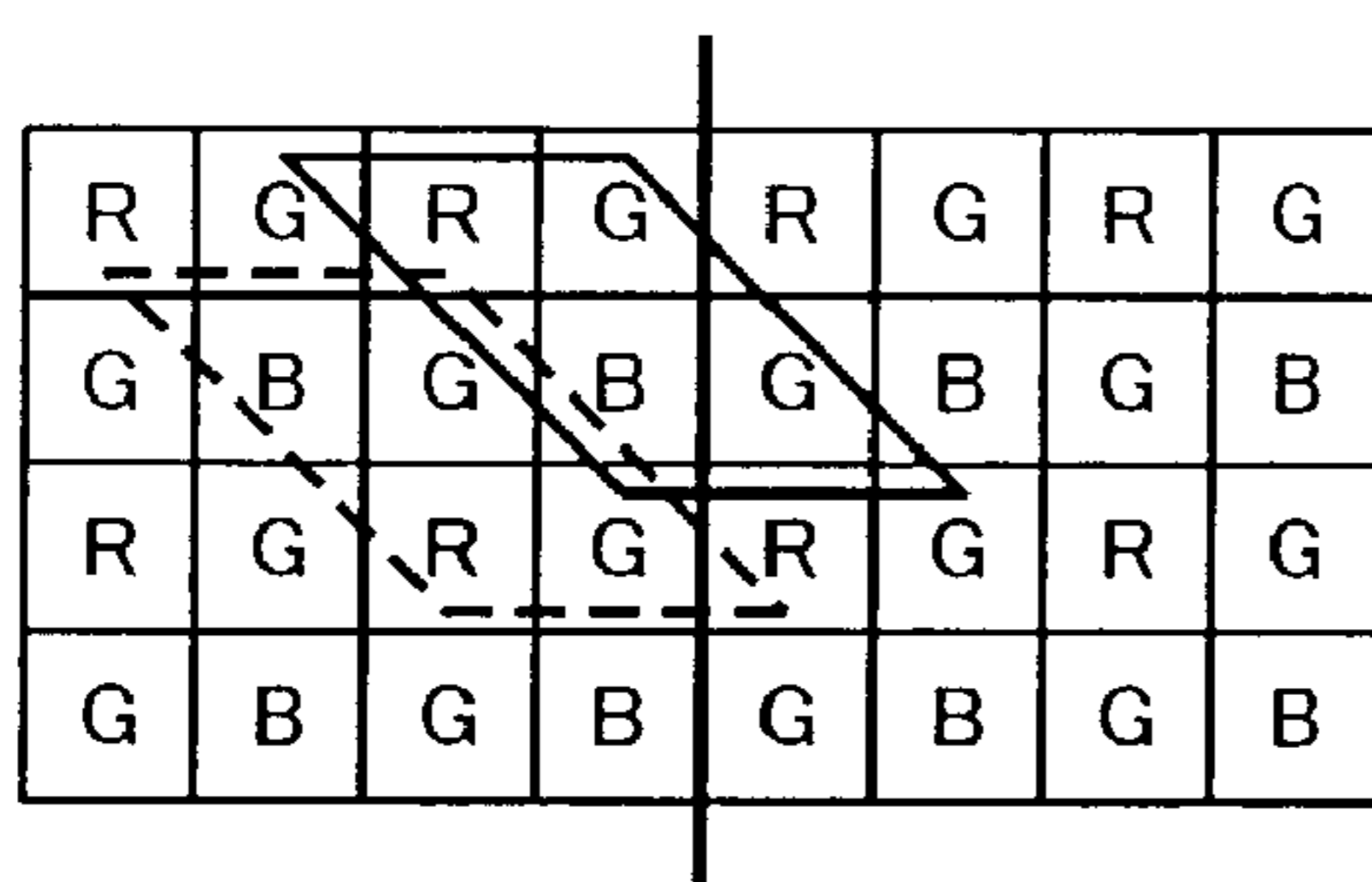
READOUT TYPE I
