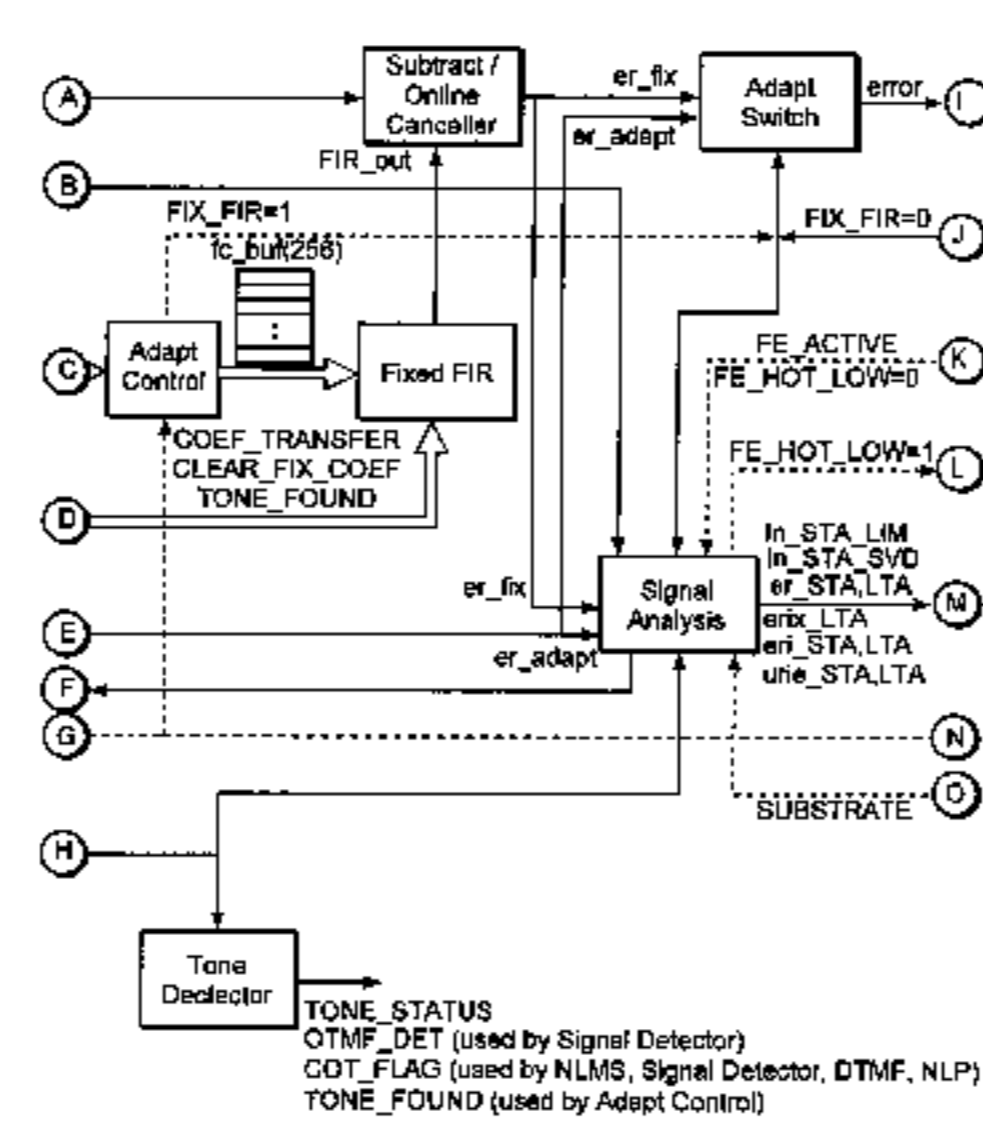
Voice Echo Canceller Block Diagram
