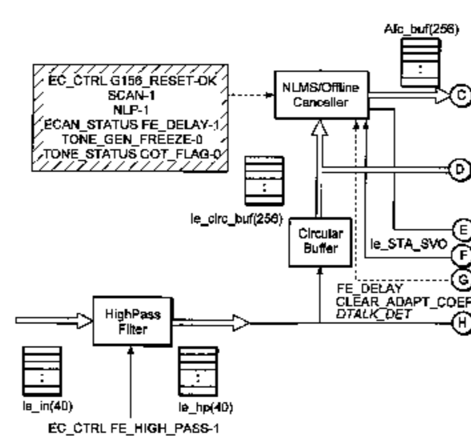
Voice Echo Canceller Block Diagram
