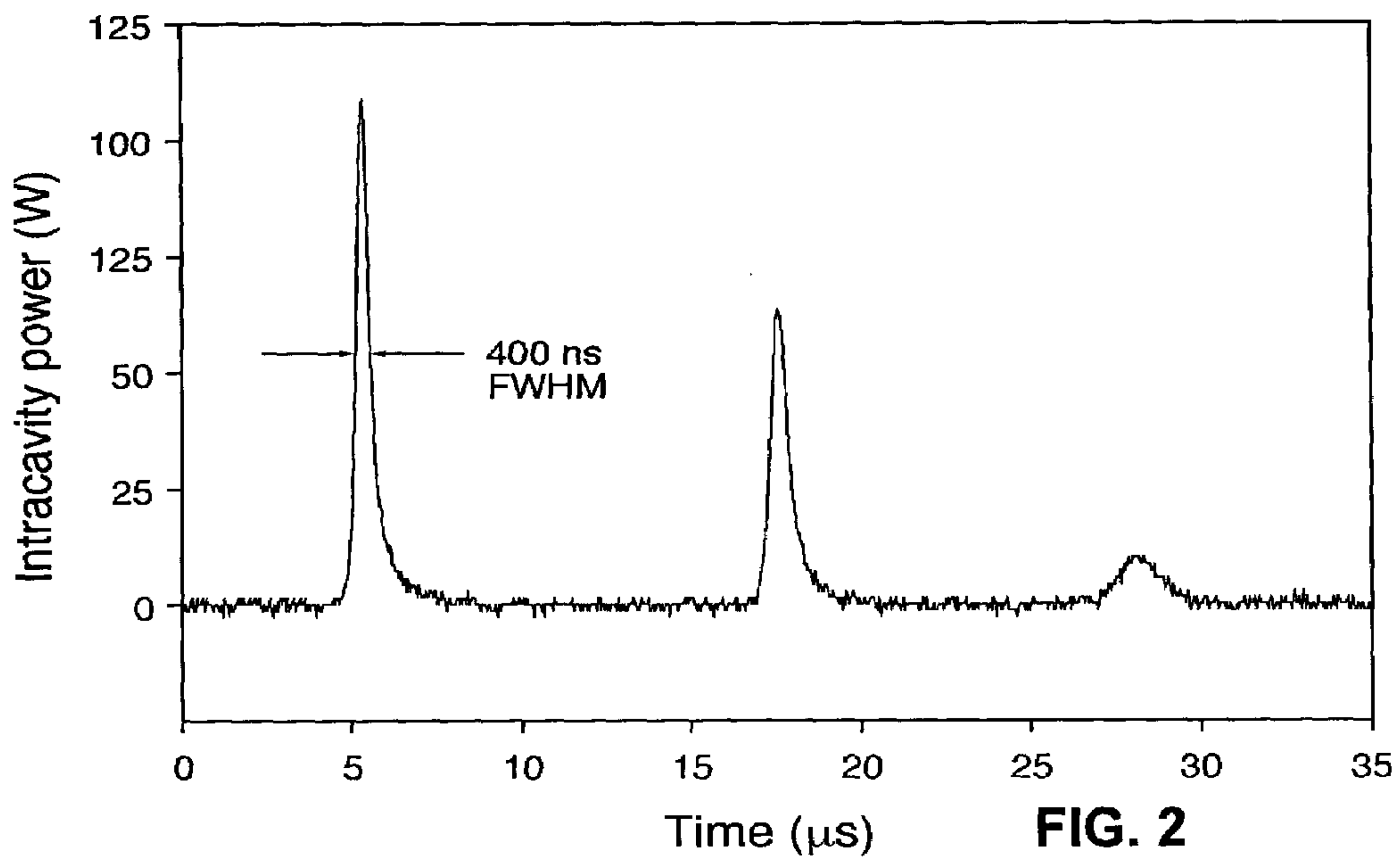
Typical relaxation-oscillation pulse-train near threshold
