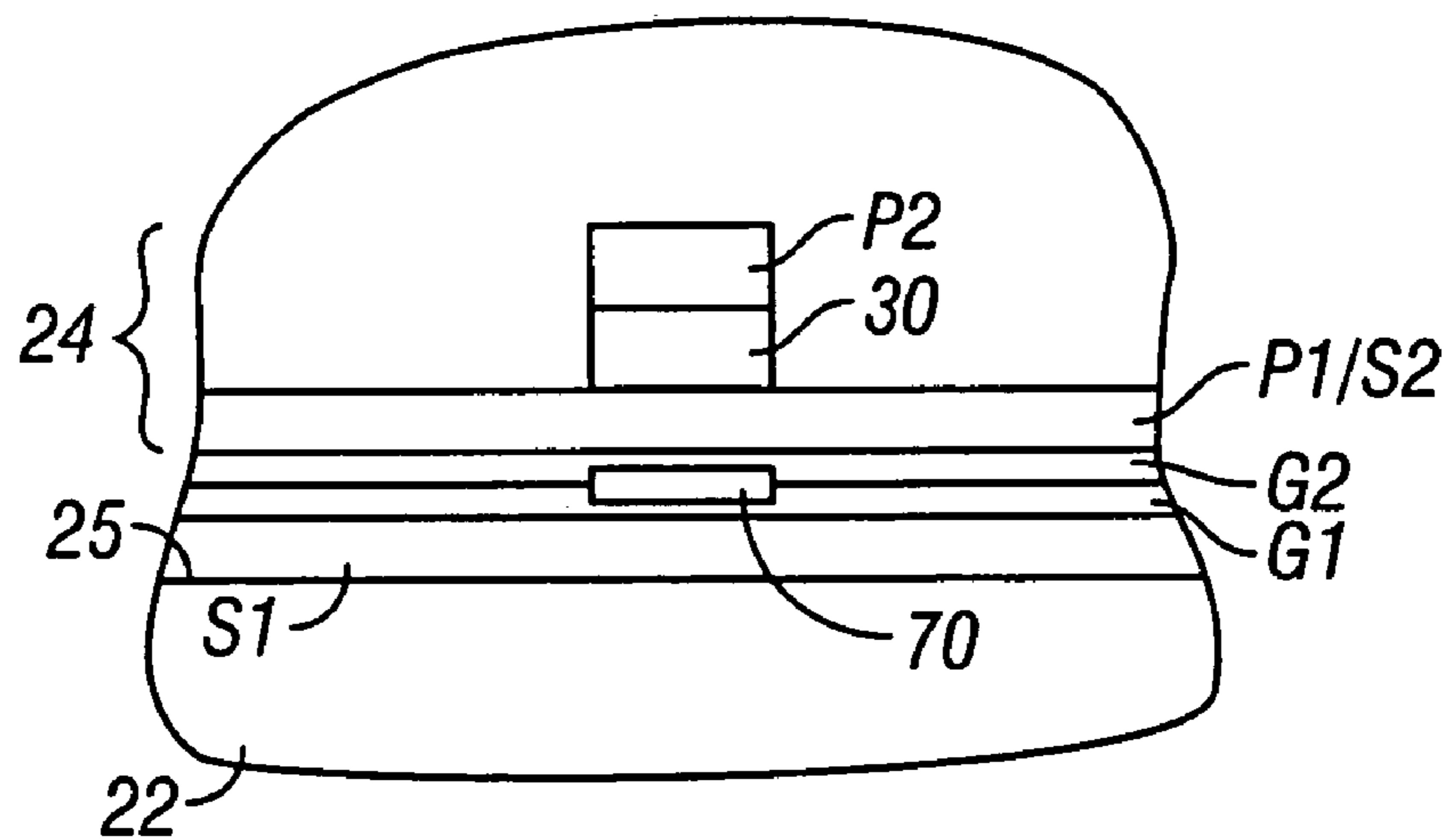
FIG. 3 (Prior Art)
