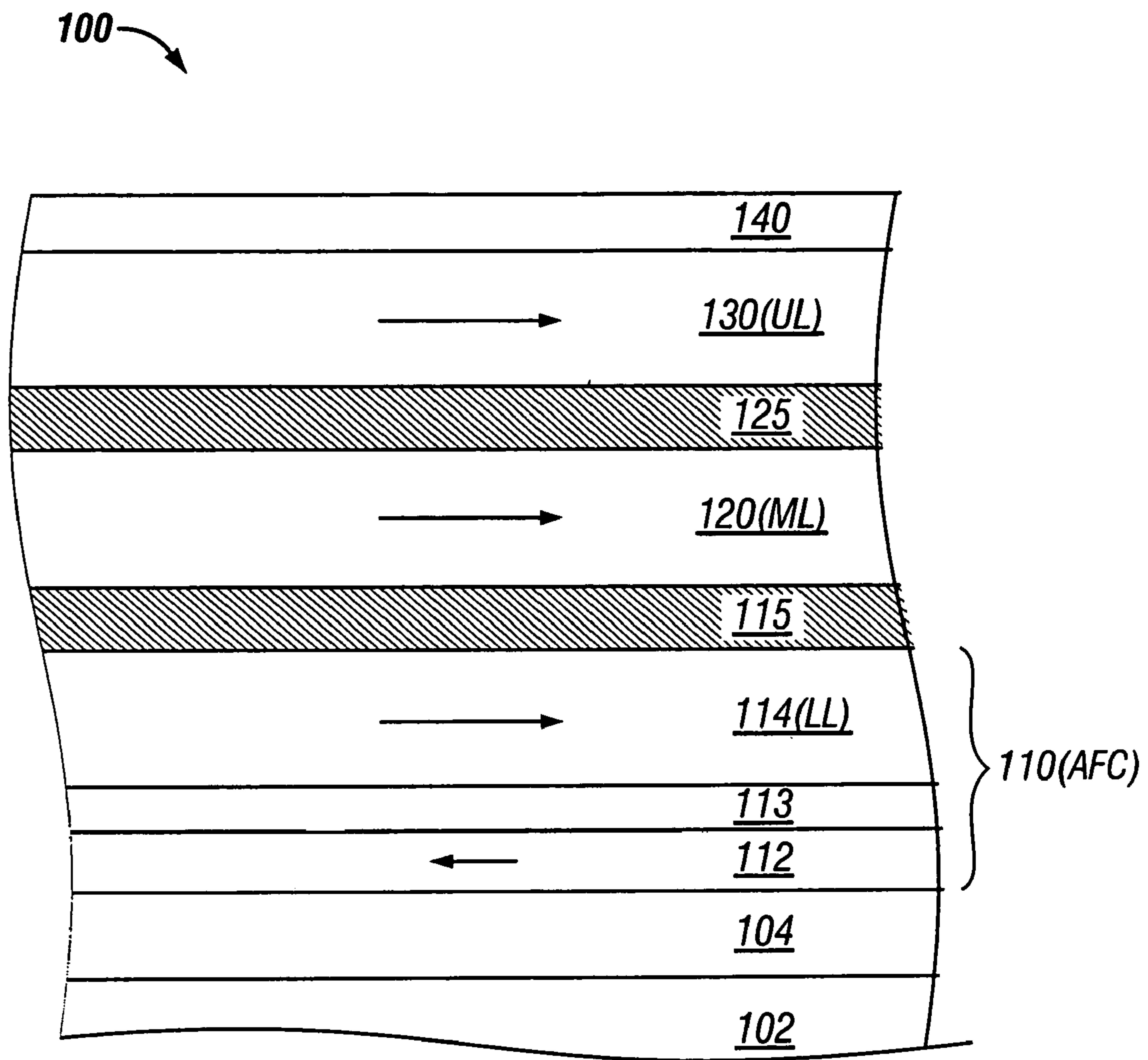
FIG. 4 (Prior Art)
