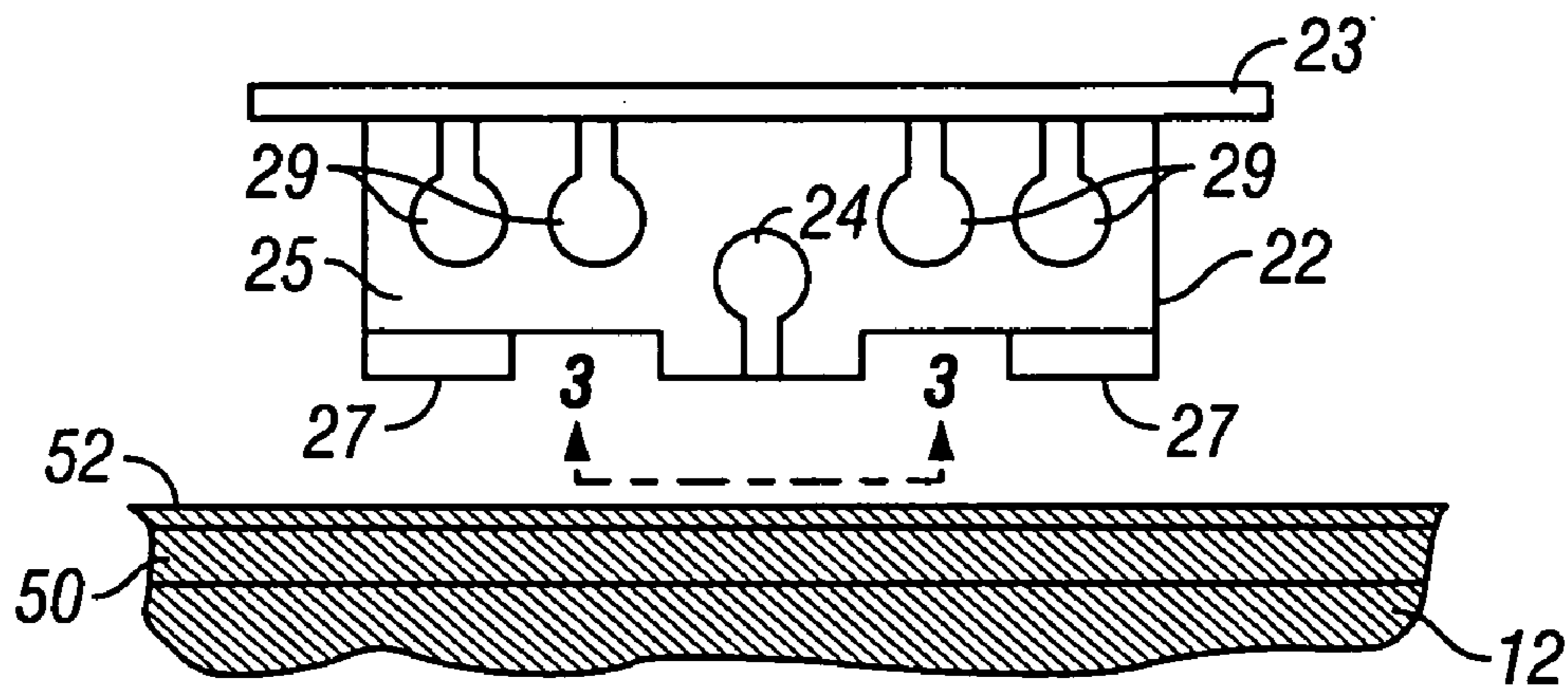
FIG. 2 (Prior Art)
