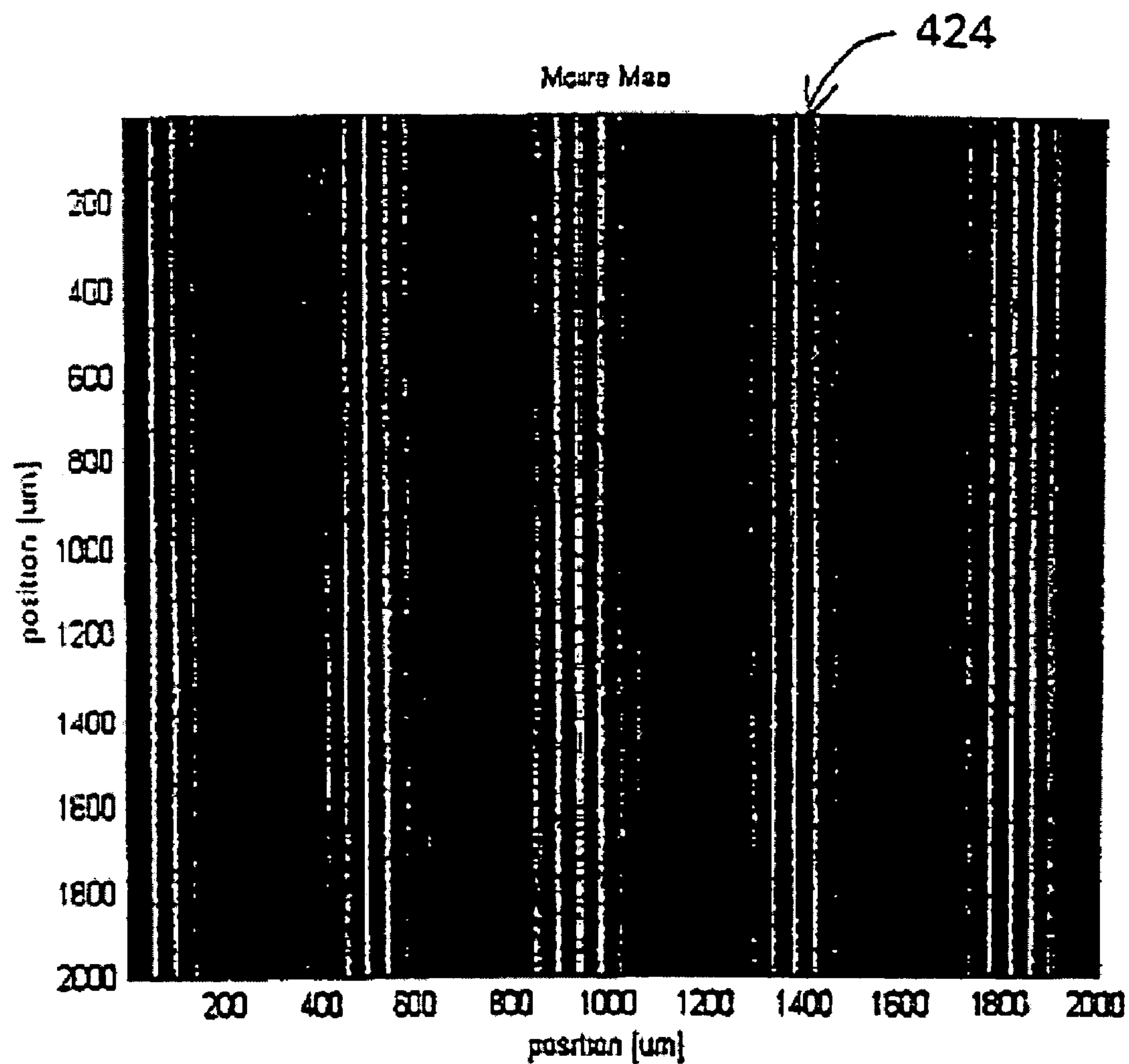
Moire Map of the 40 \mu\text{m} Pitch Prism Array Against A 44 \mu\text{m} Pitch Reference Prism Array
