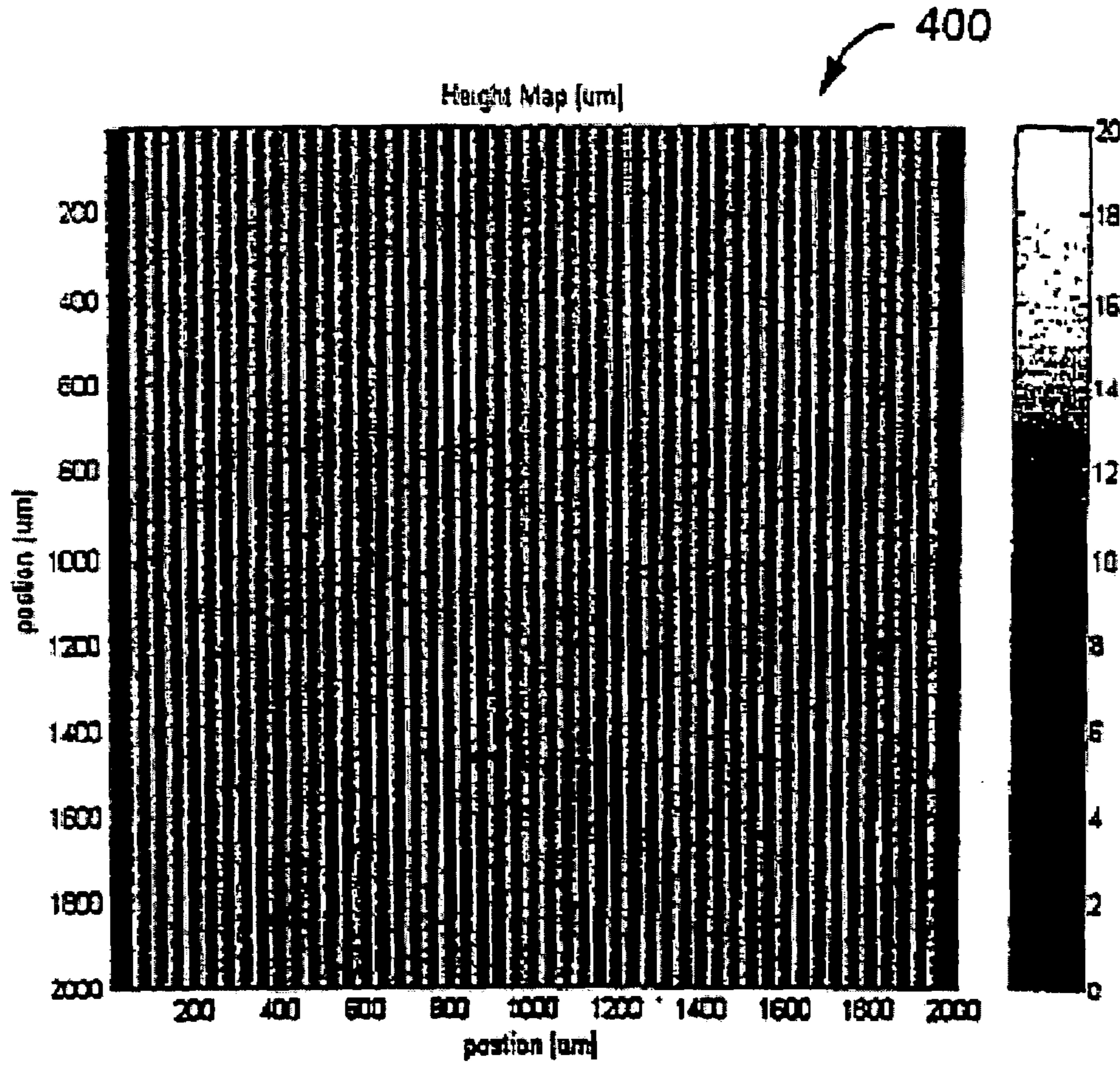
40 \mu\text{m} Pitch Prism Array
