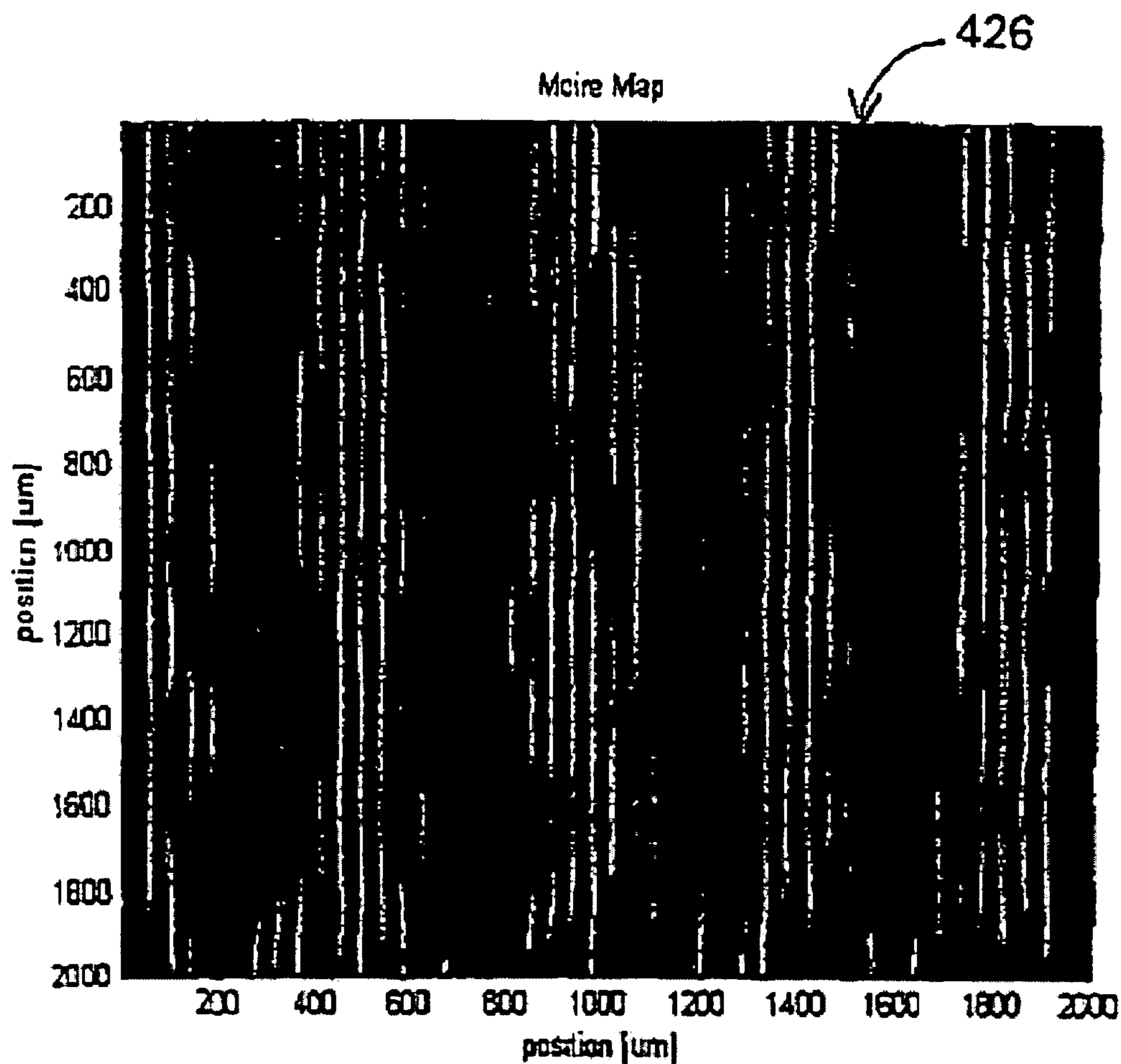
Moire Map of the 40 μm Pitch Prism Array of FIG.22 Against A 44 μm Pitch Reference Prism Array
