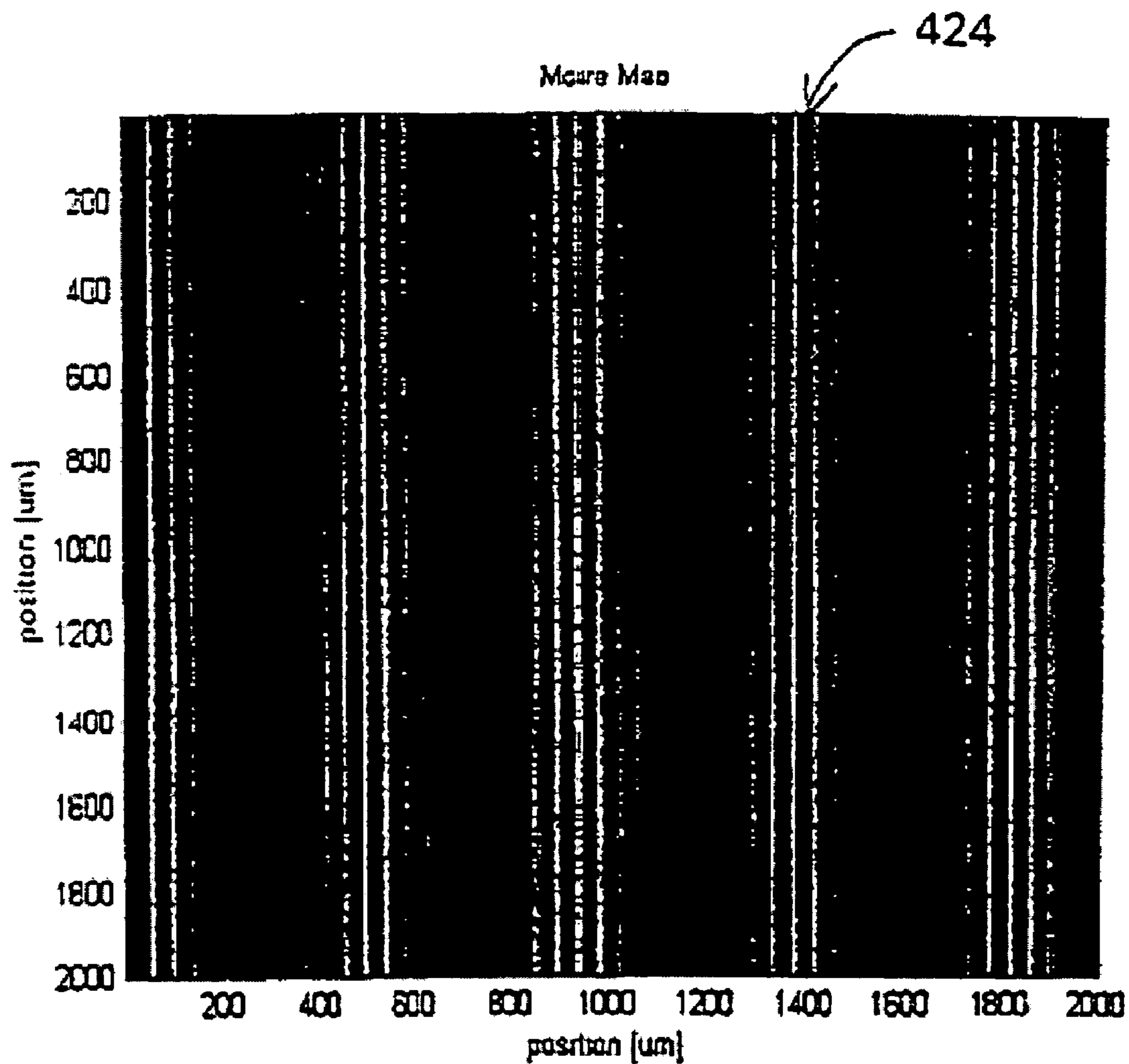
Moire Map of the 40 μm Pitch Prism Array Against A 44 μm Pitch Reference Prism Array
