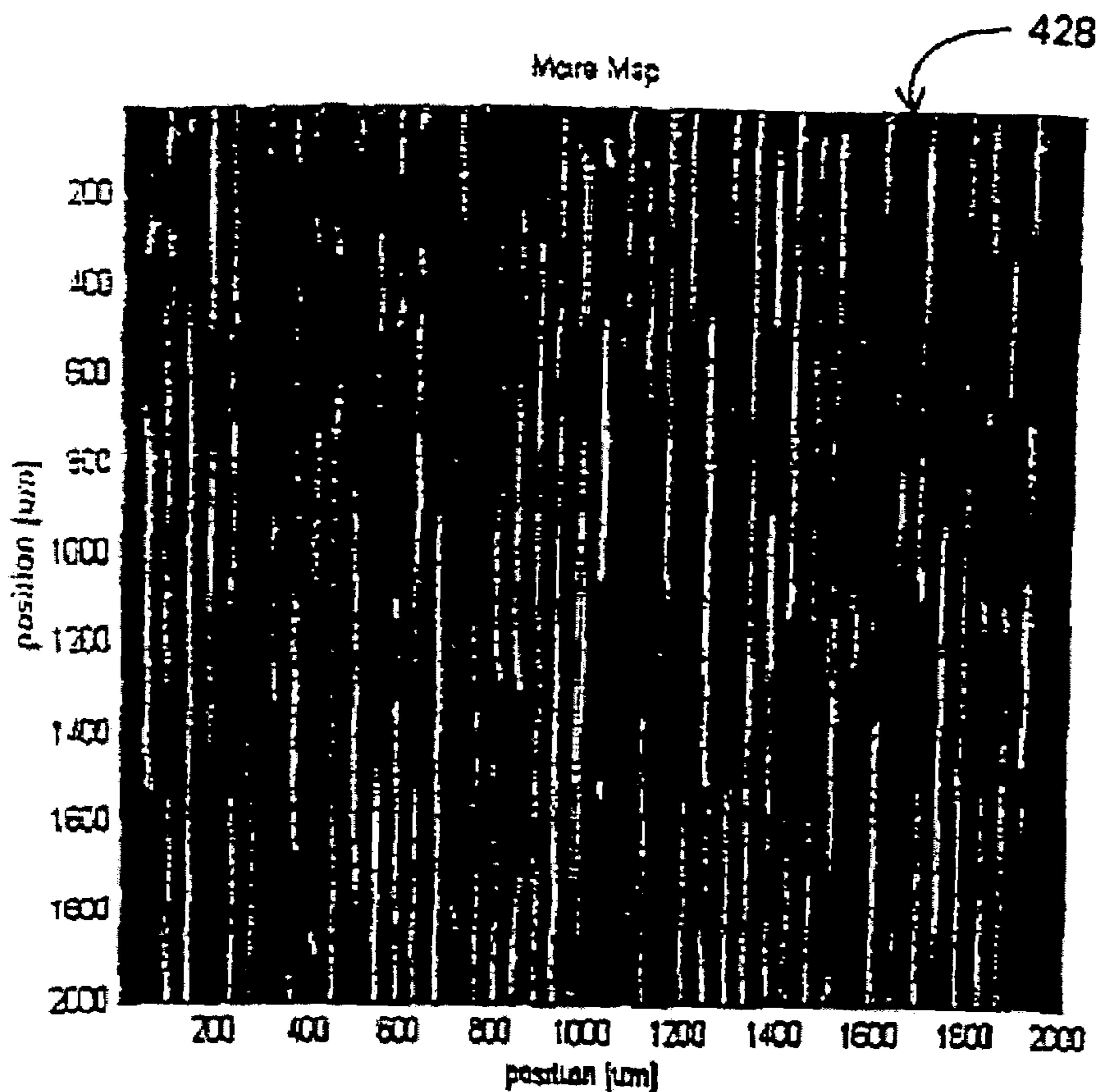
Moire Map of FIG.26 Against a 44 \mu\text{m} Pitch Reference Prism Array
