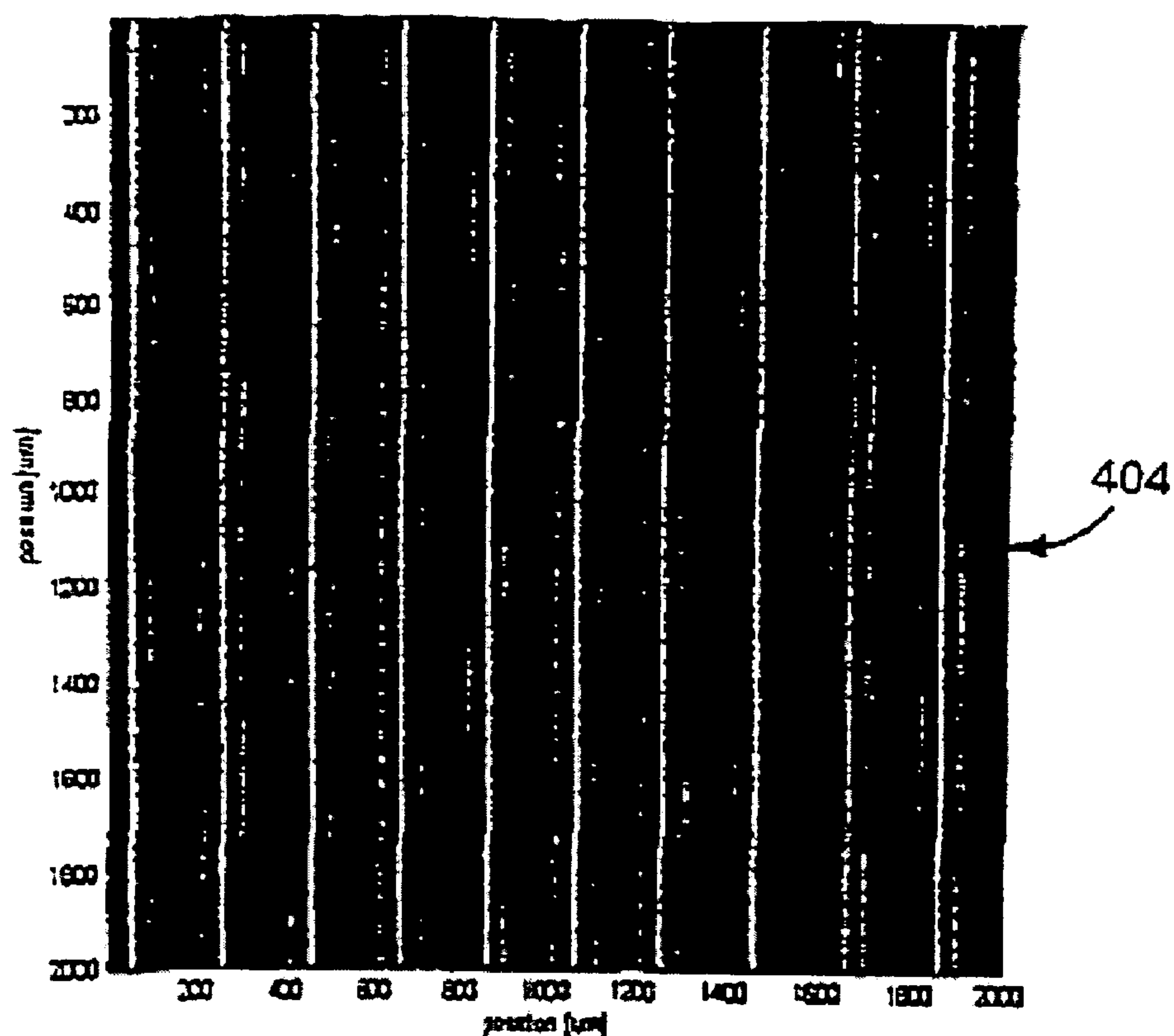
Moire Map of the 40 \mu\text{m} Pitch Prism Array of FIG. 18 with a 50 \mu\text{m} Reference Prism Array
