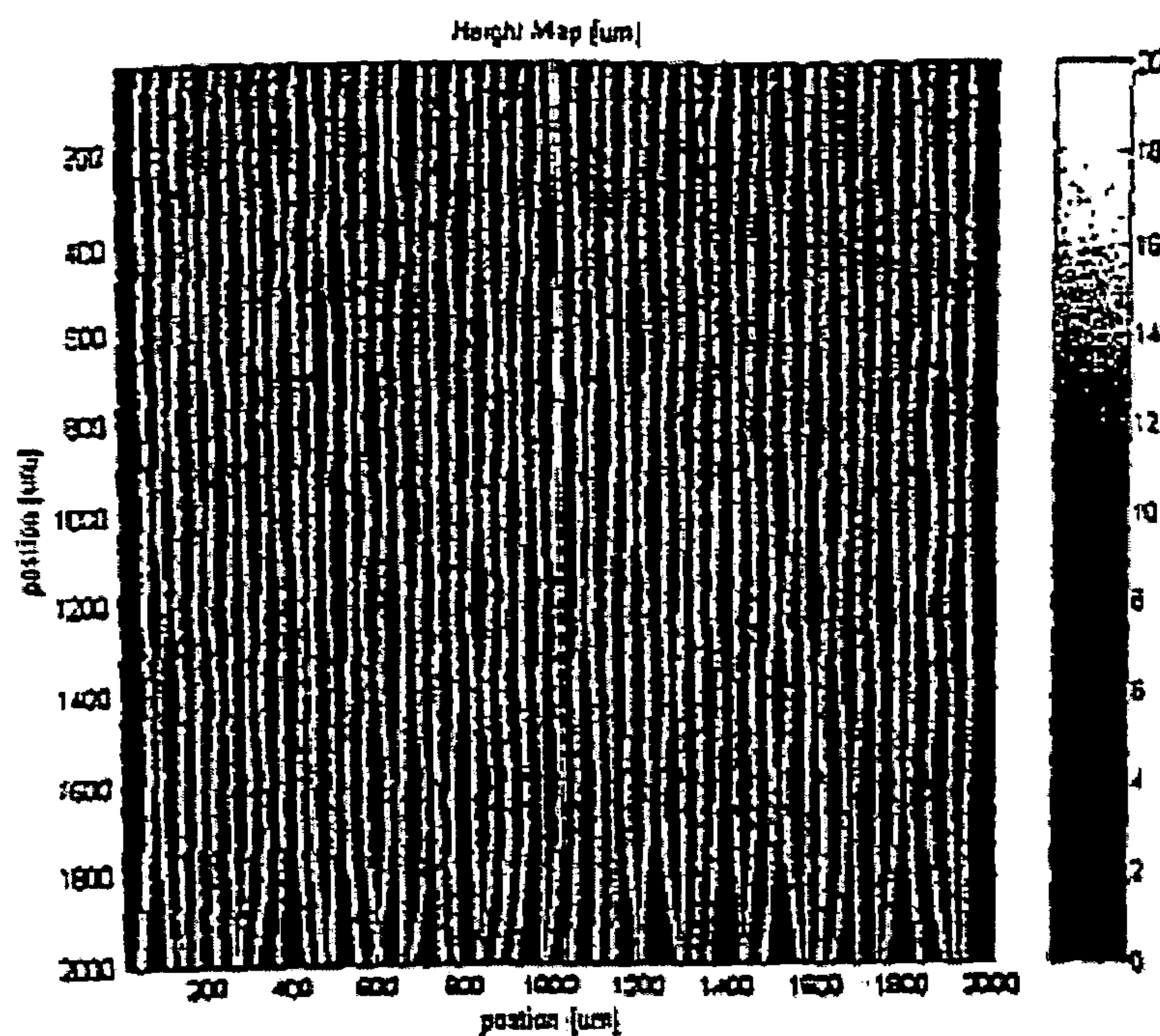
The Prism Array of FIG.18 with \pm 20\% Randomness Introduced Into The Horizontal Position of the Prism Centers
