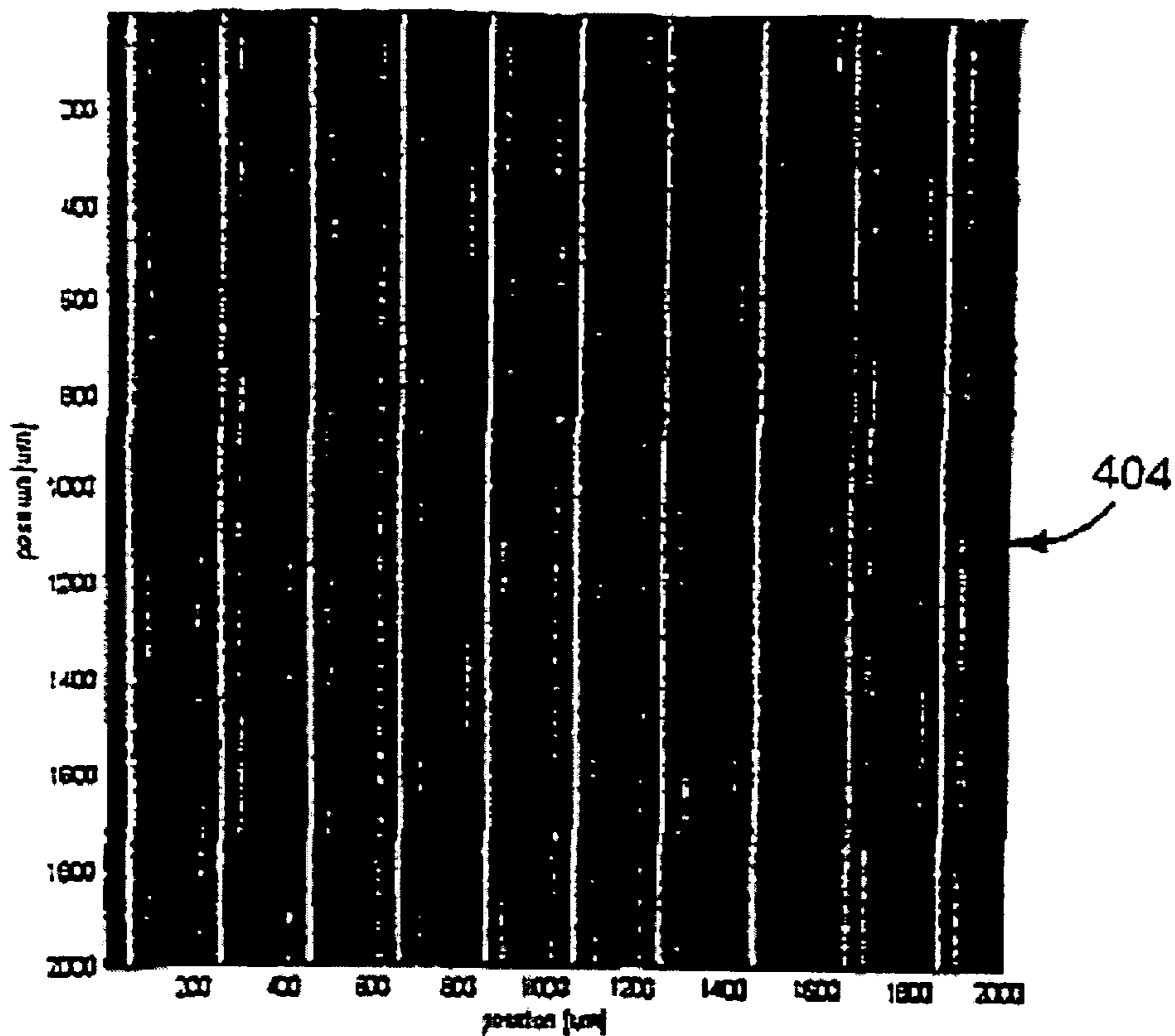
Moire Map of the 40 \mu\text{m} Pitch Prism Array of FIG. 18 with a 50 \mu\text{m} Reference Prism Array
