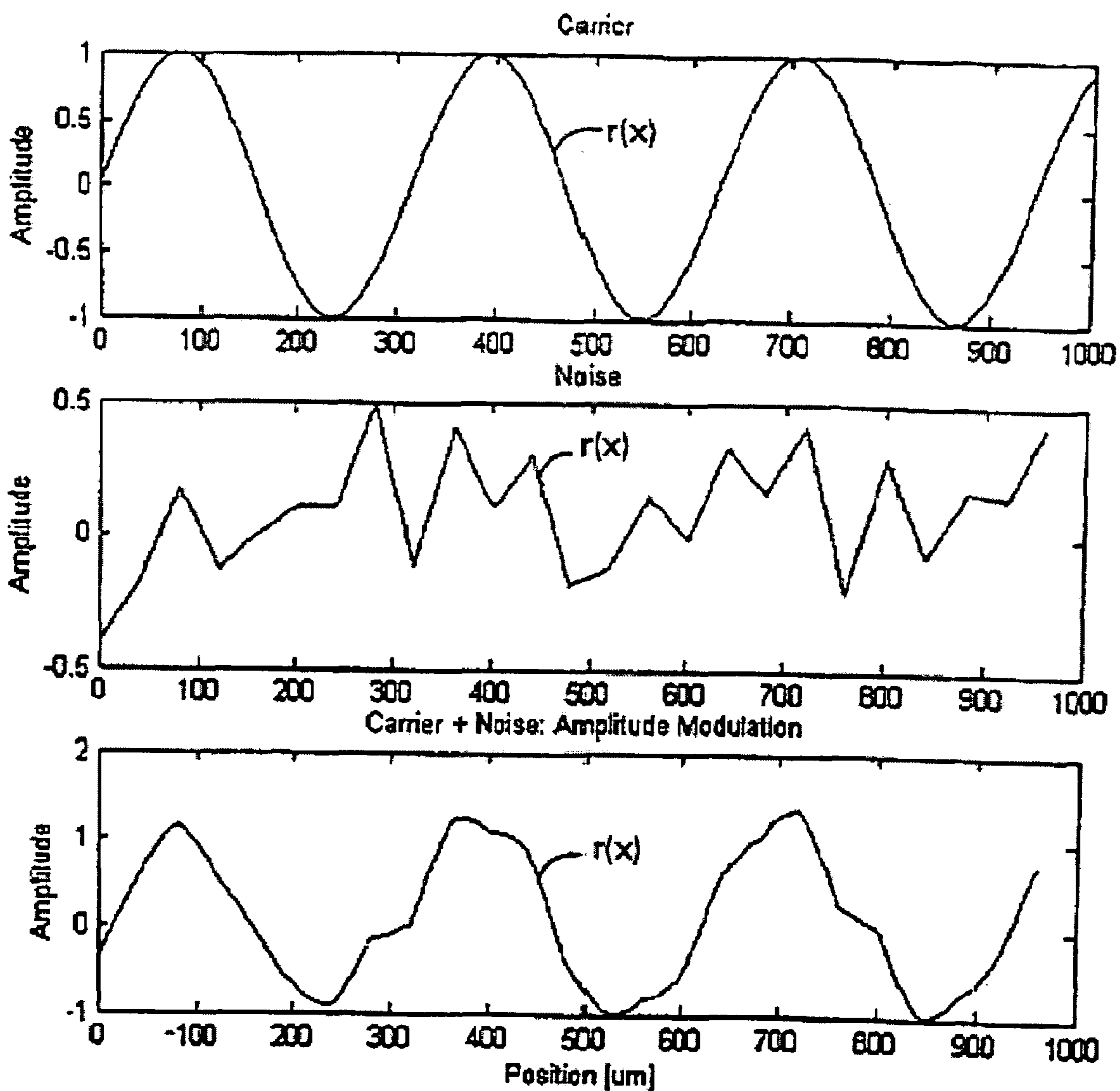
Amplitude modulation example r(x) + \sin(x/50)
