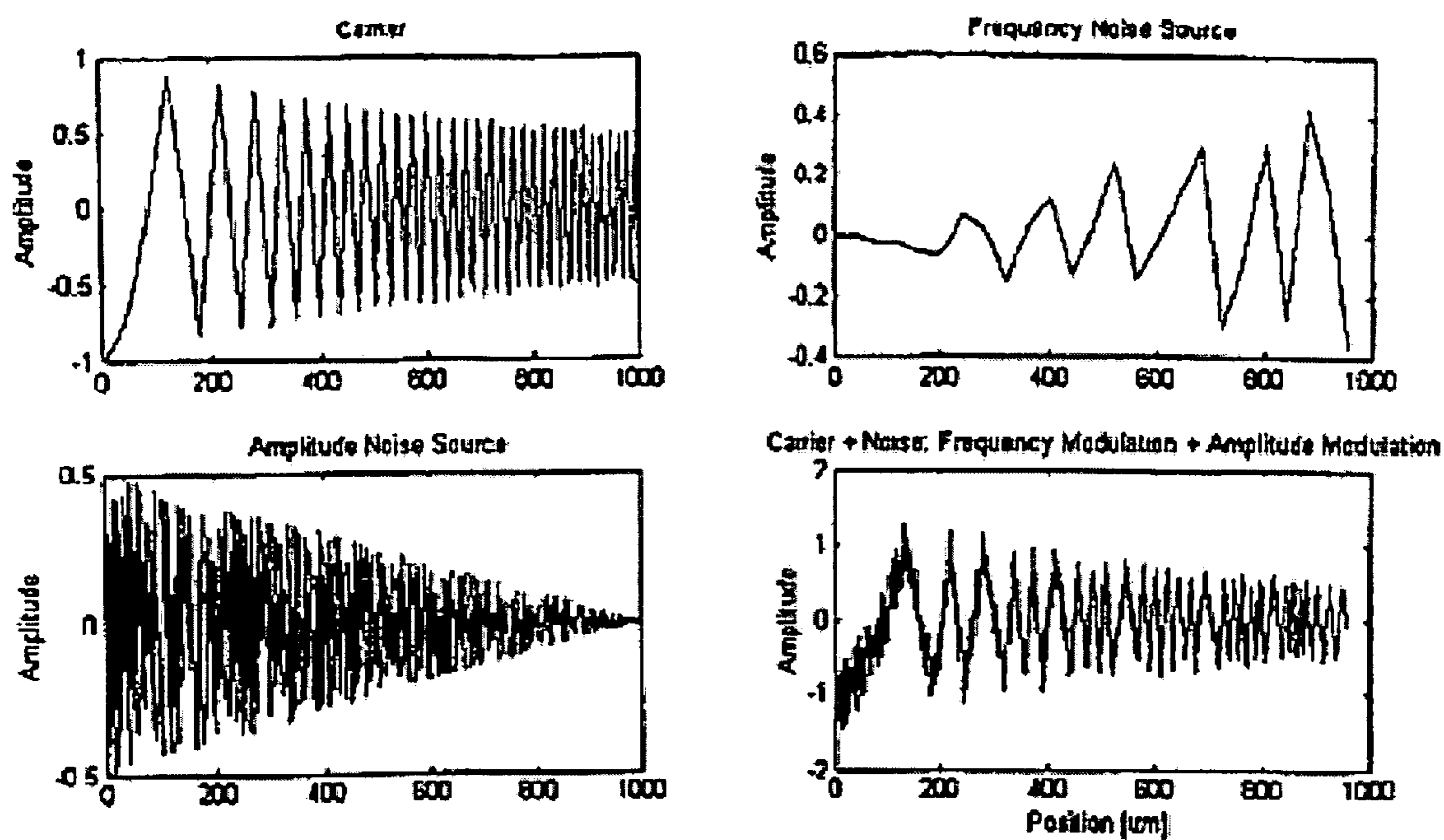
Frequency and Amplitude modulation example with spatially varying carrier and noise functions: r'(z) + \text{sawtooth}(z^2 / (5000 + 10r(z))) * (1000) / (z + 1000)
