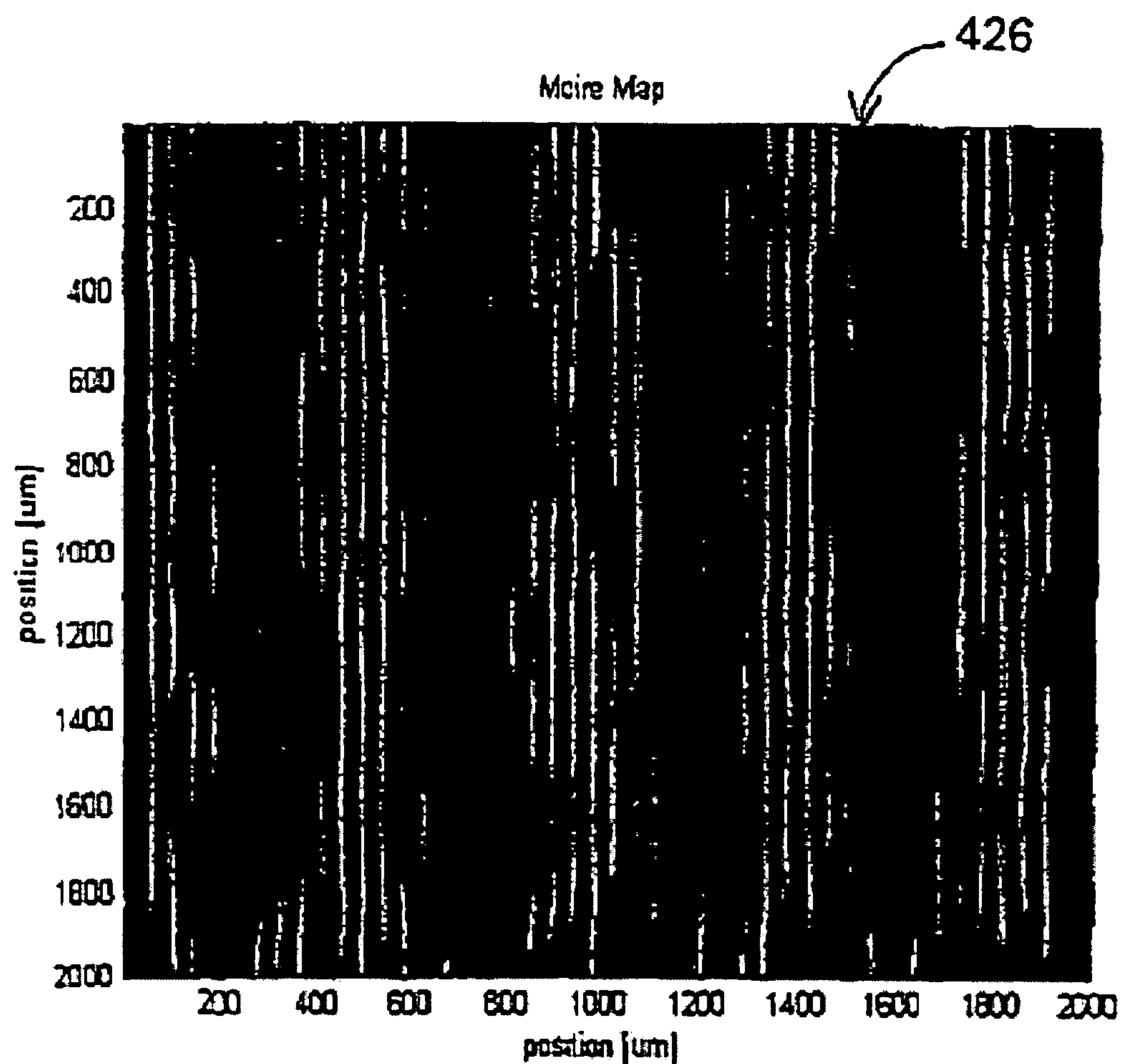
Moire Map of the 40 \mu\text{m} Pitch Prism Array of FIG.22 Against A 44 \mu\text{m} Pitch Reference Prism Array
