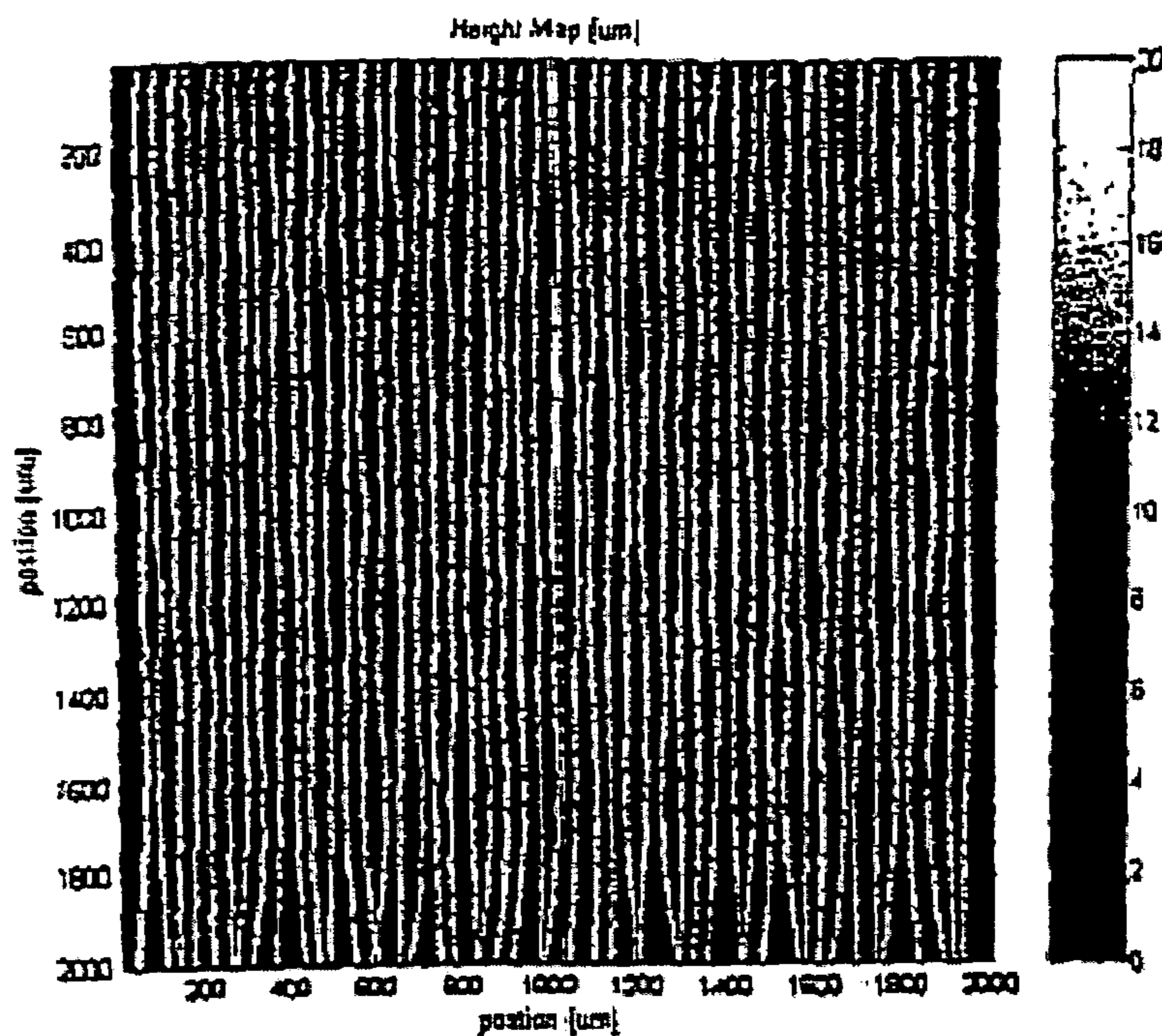
The Prism Array of FIG.18 with +/- 20% Randomness Introduced Into The Horizontal Position of the Prism Centers
