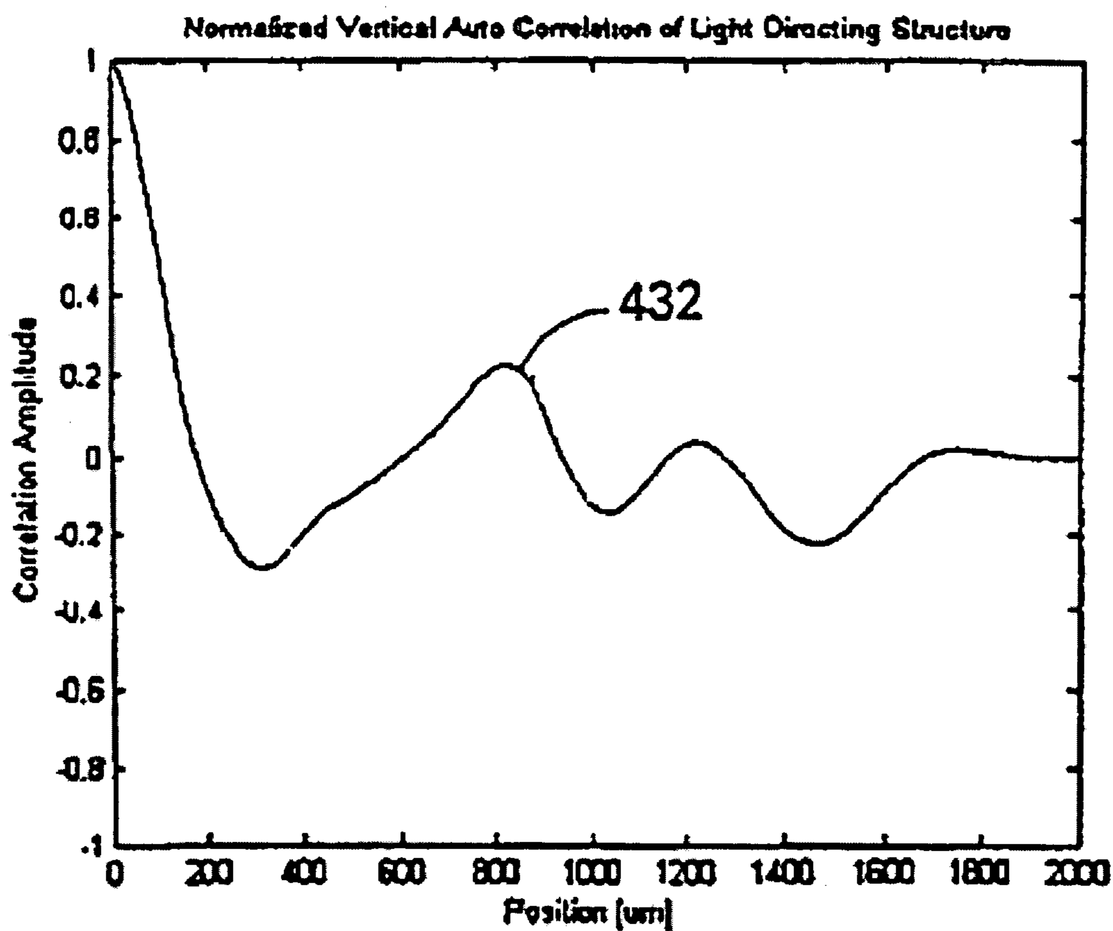
Auto Correlation of FIG.22 along "z"
