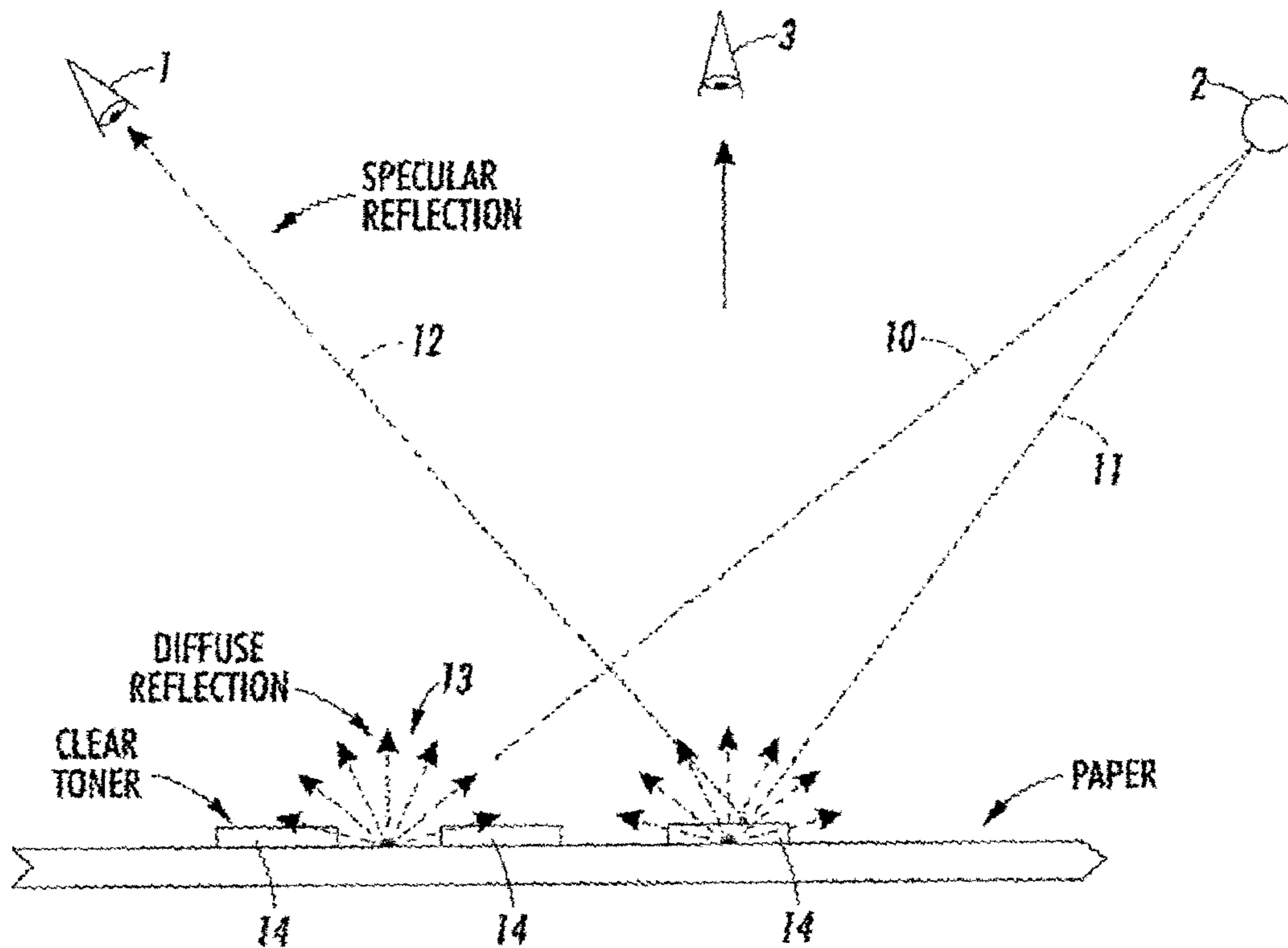
FIG. 1 (PRIOR ART)
