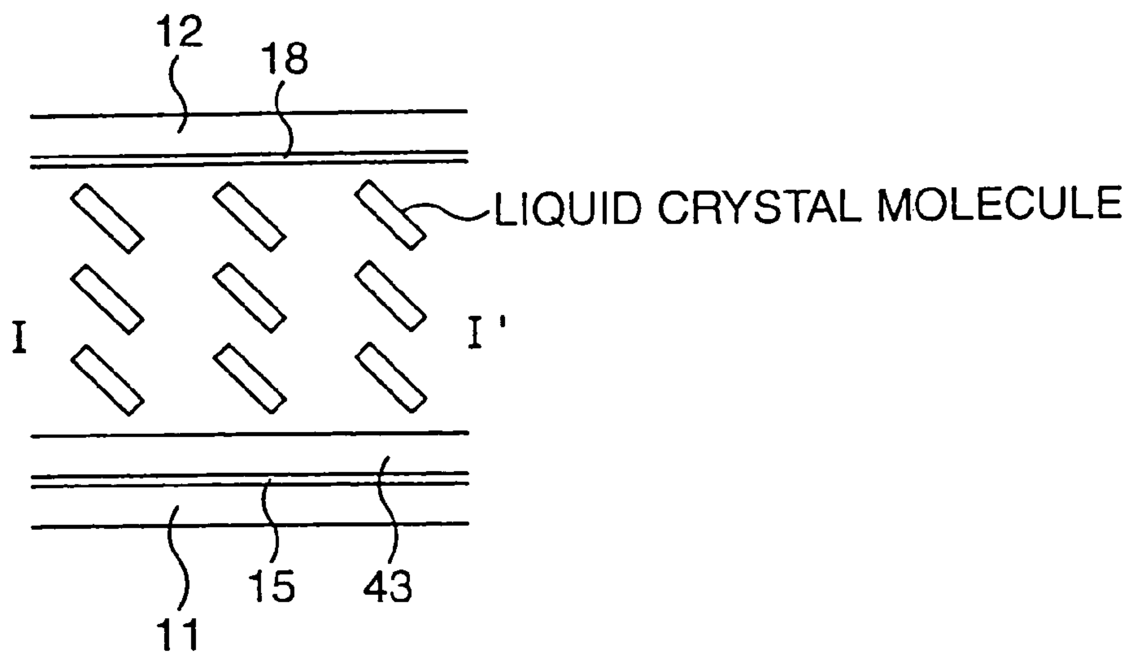
SECTIONAL VIEW
