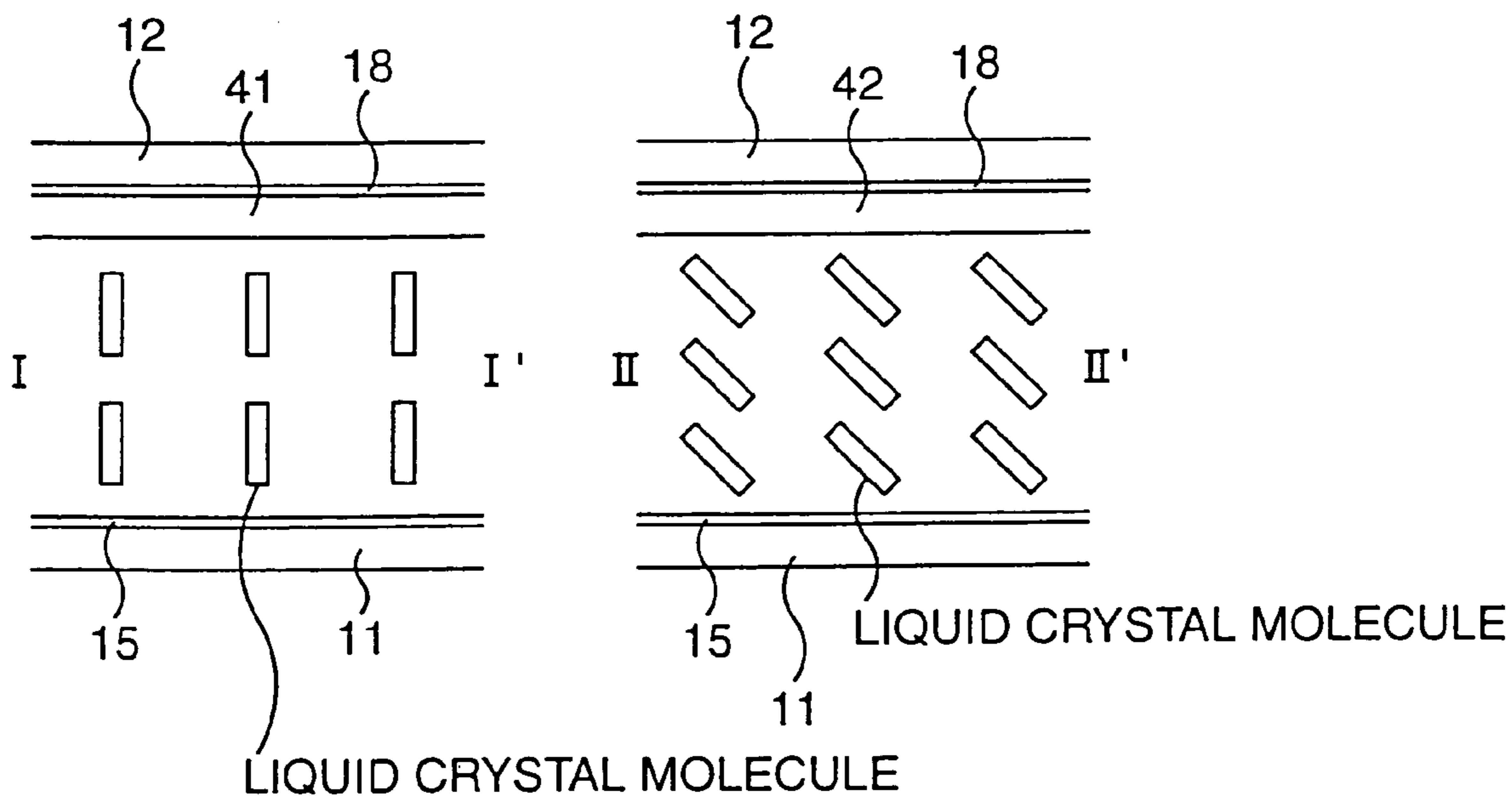
SECTIONAL VIEW
