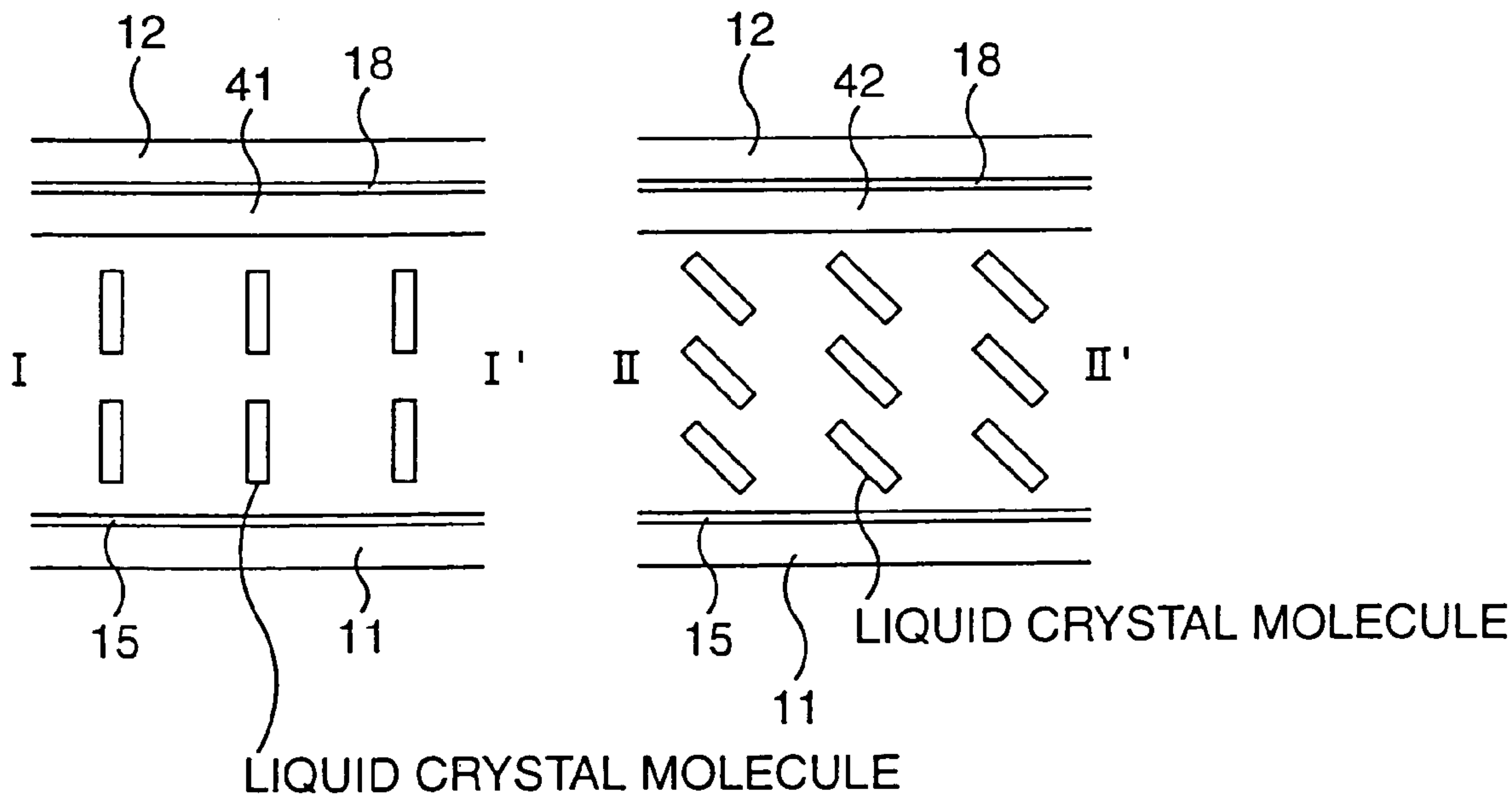
SECTIONAL VIEW
