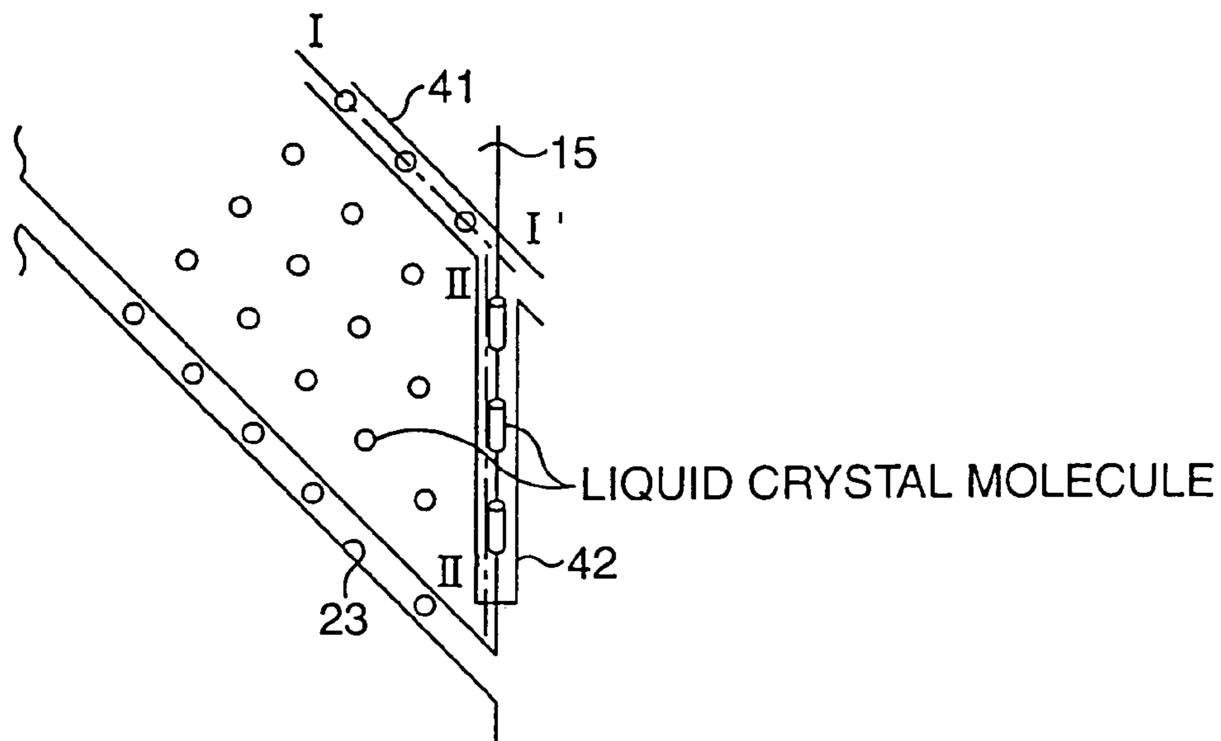
PLANE VIEW
