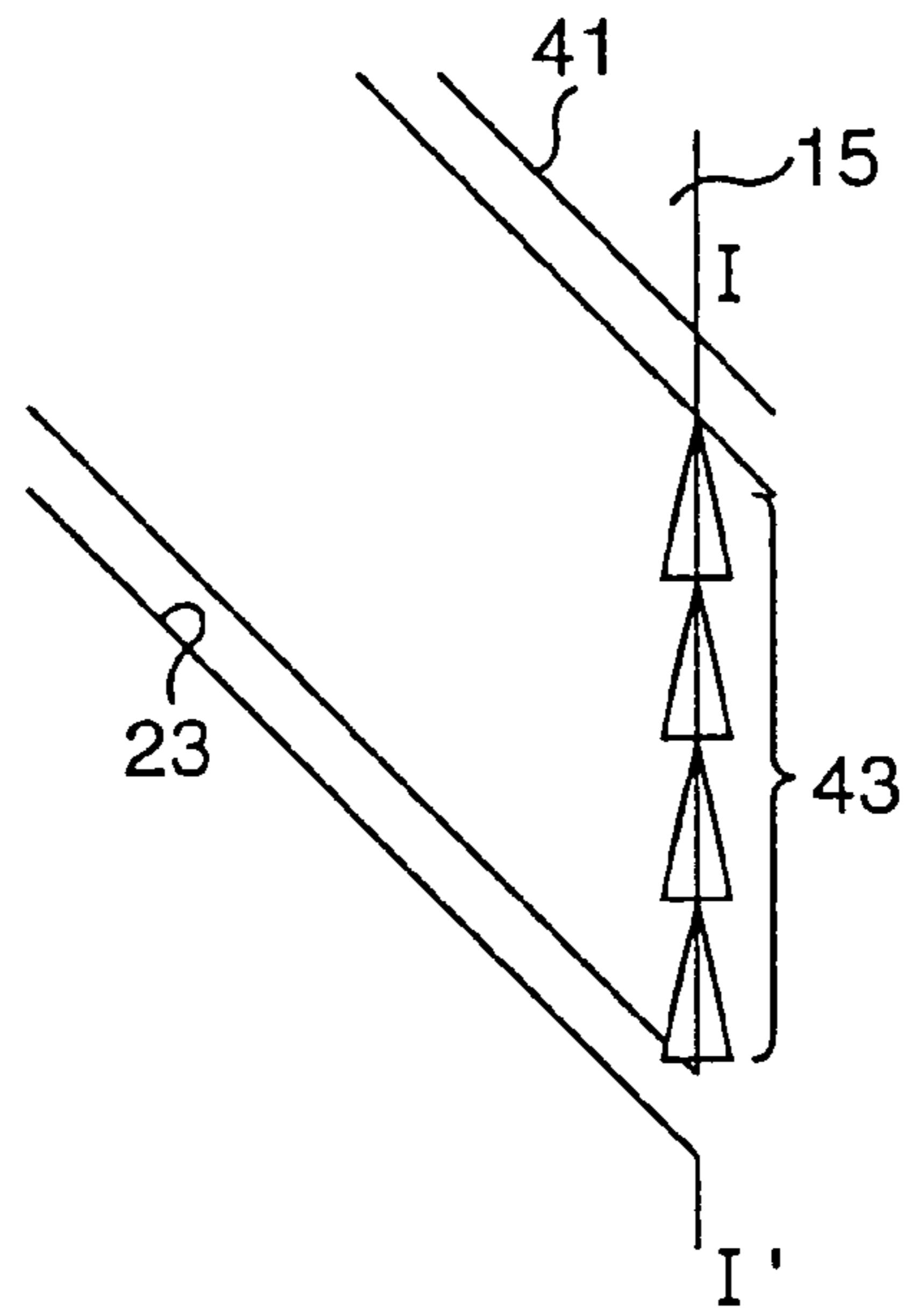
PLANE VIEW
