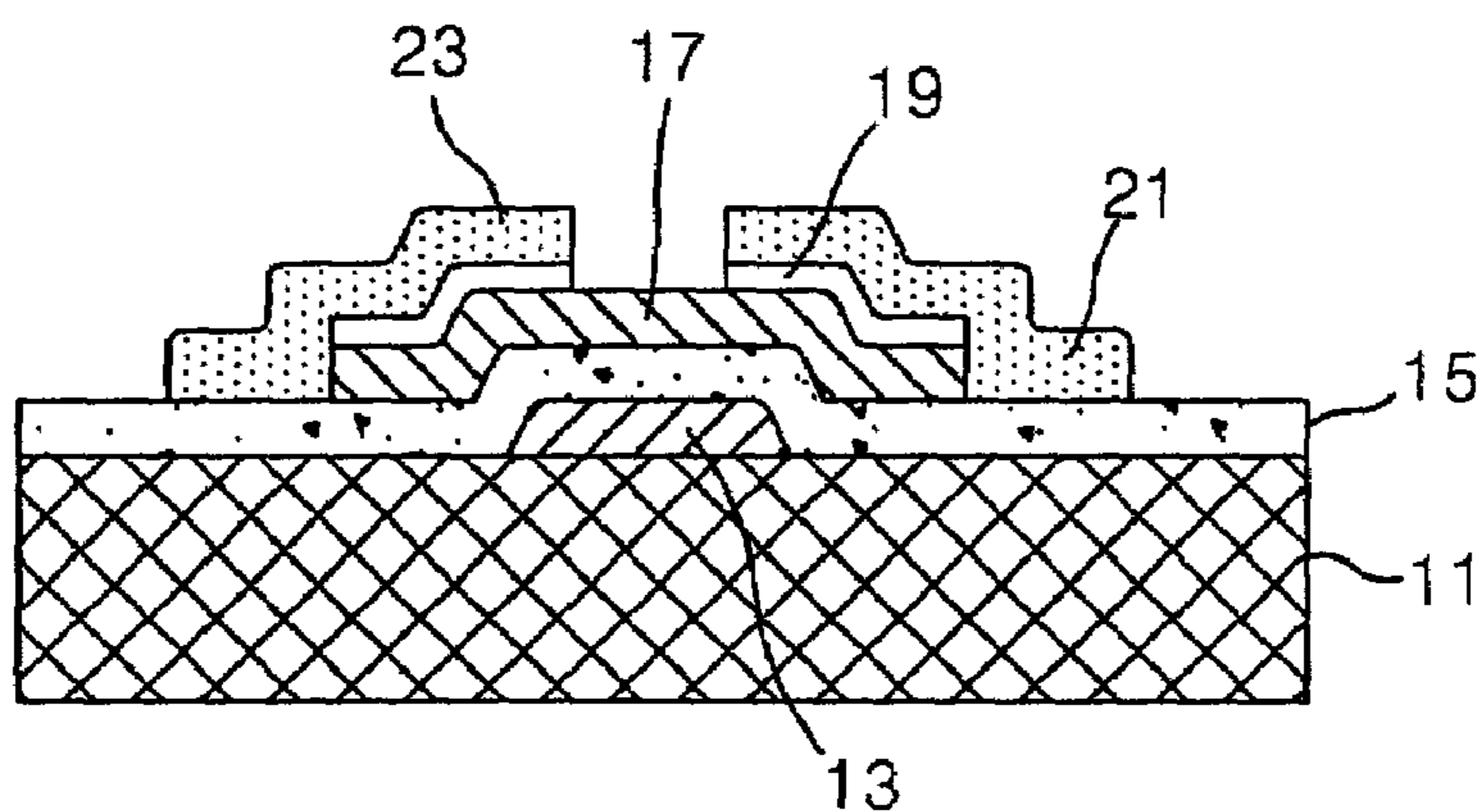
FIG. 1C CONVENTIONAL ART
