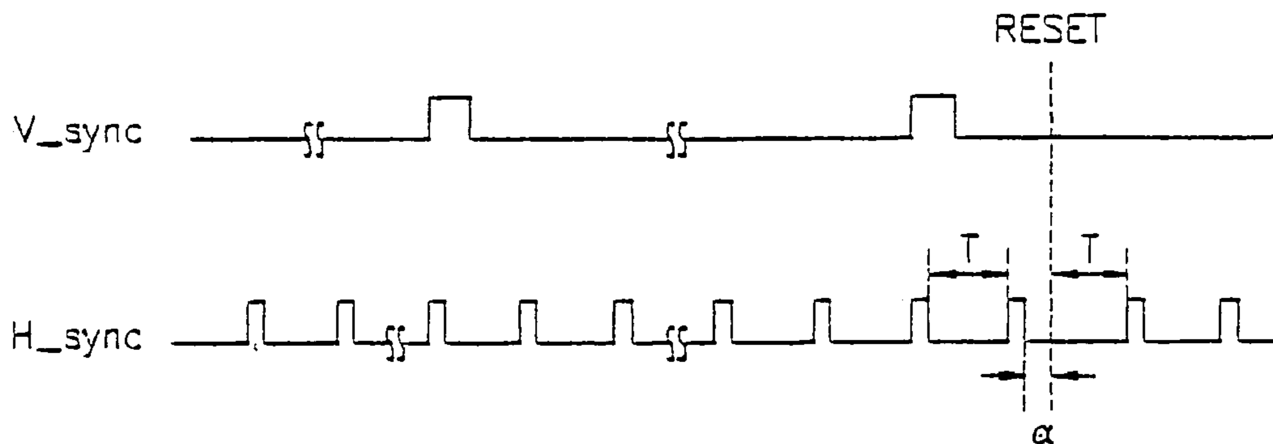
FIG. 2 (PRIOR ART)
