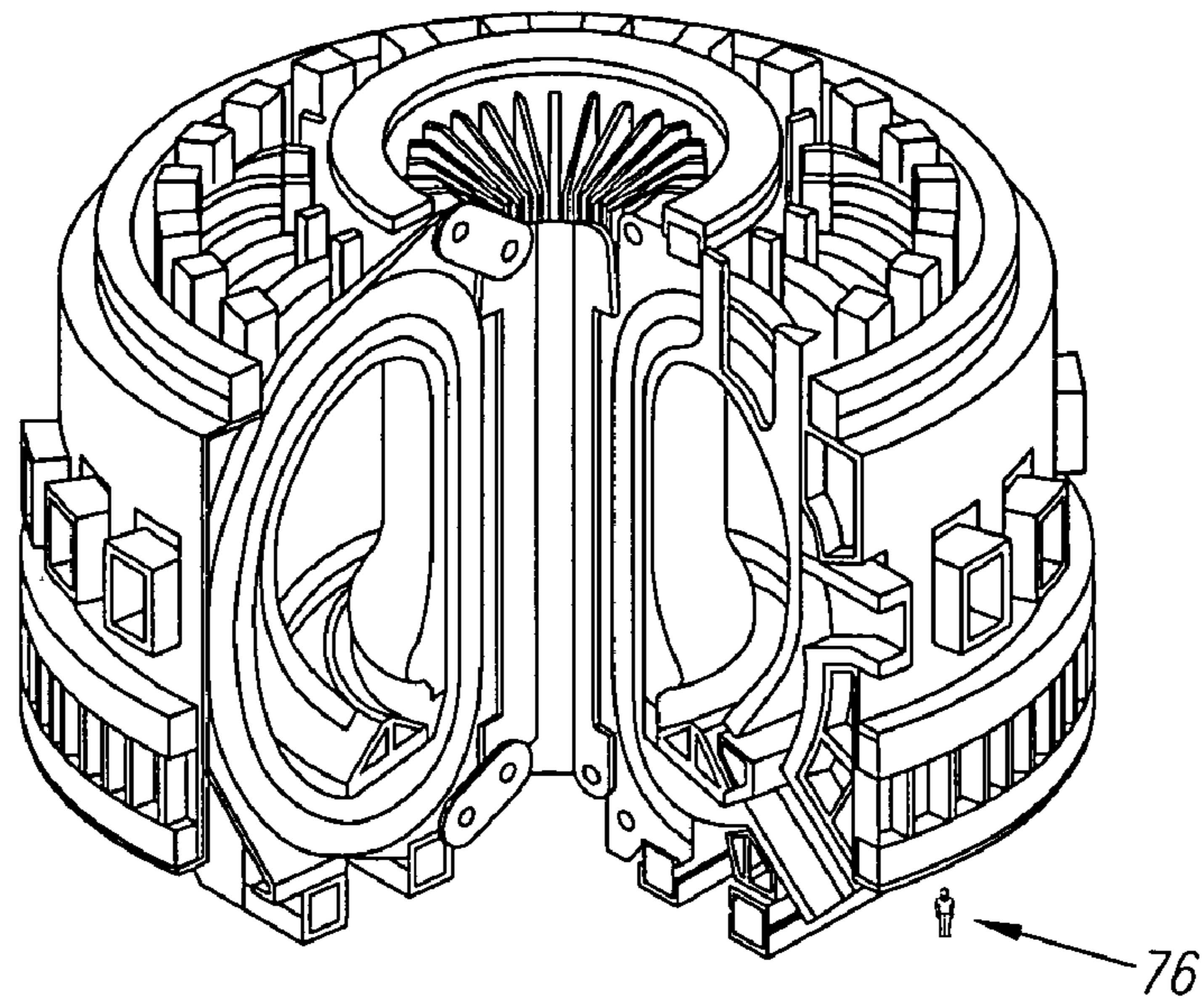
FIG. 7 (PRIOR ART)
