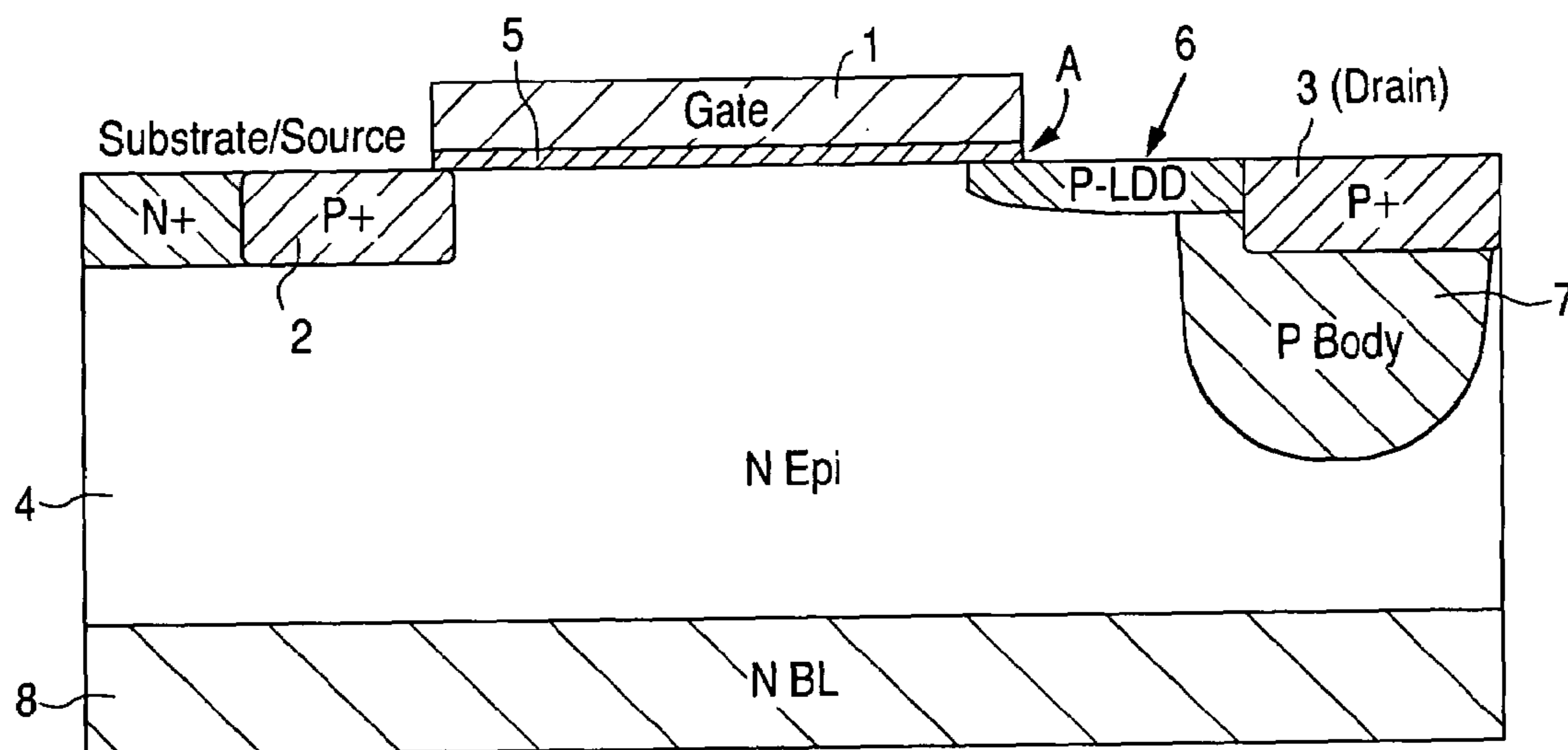
FIG. 1 (PRIOR ART)
