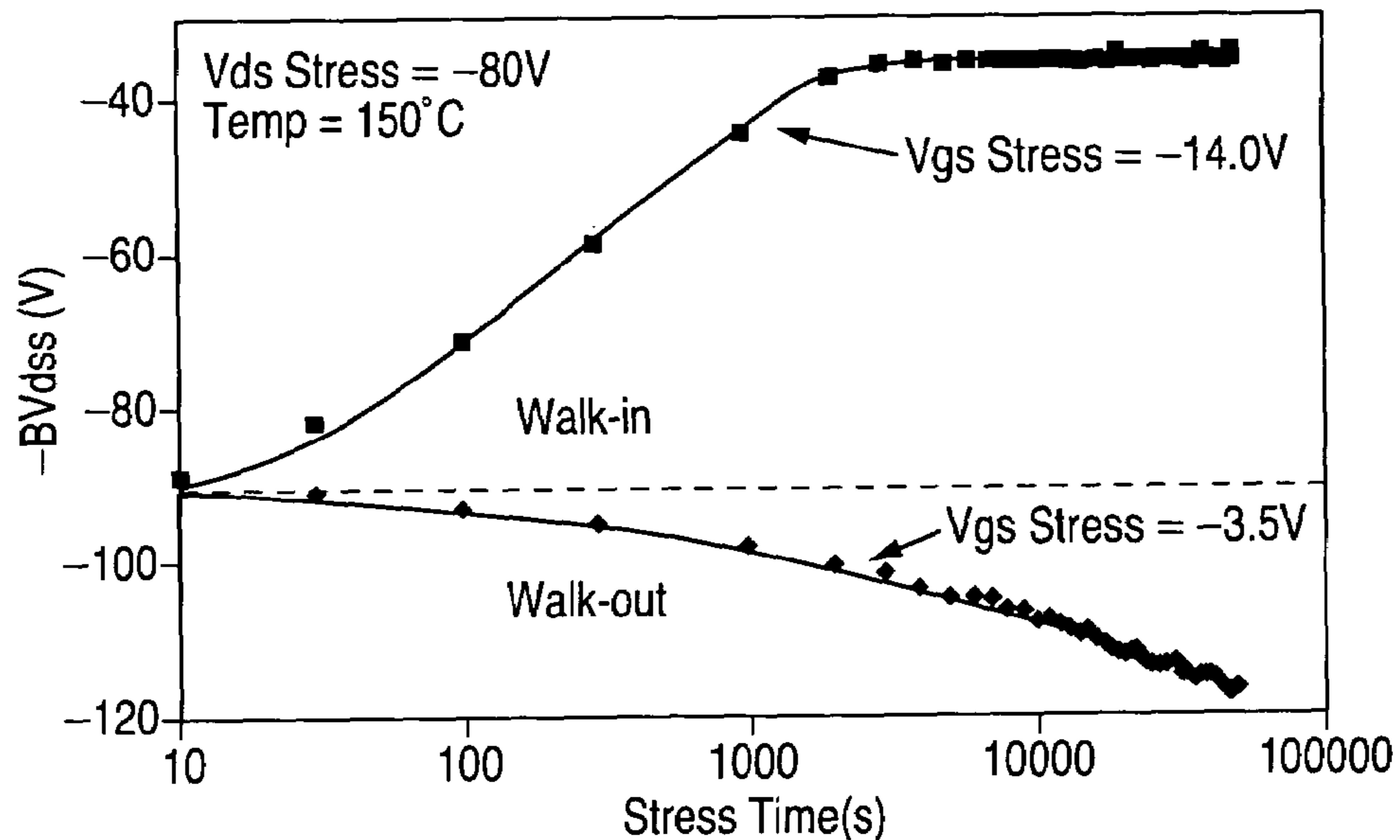
FIG. 2 (PRIOR ART)
