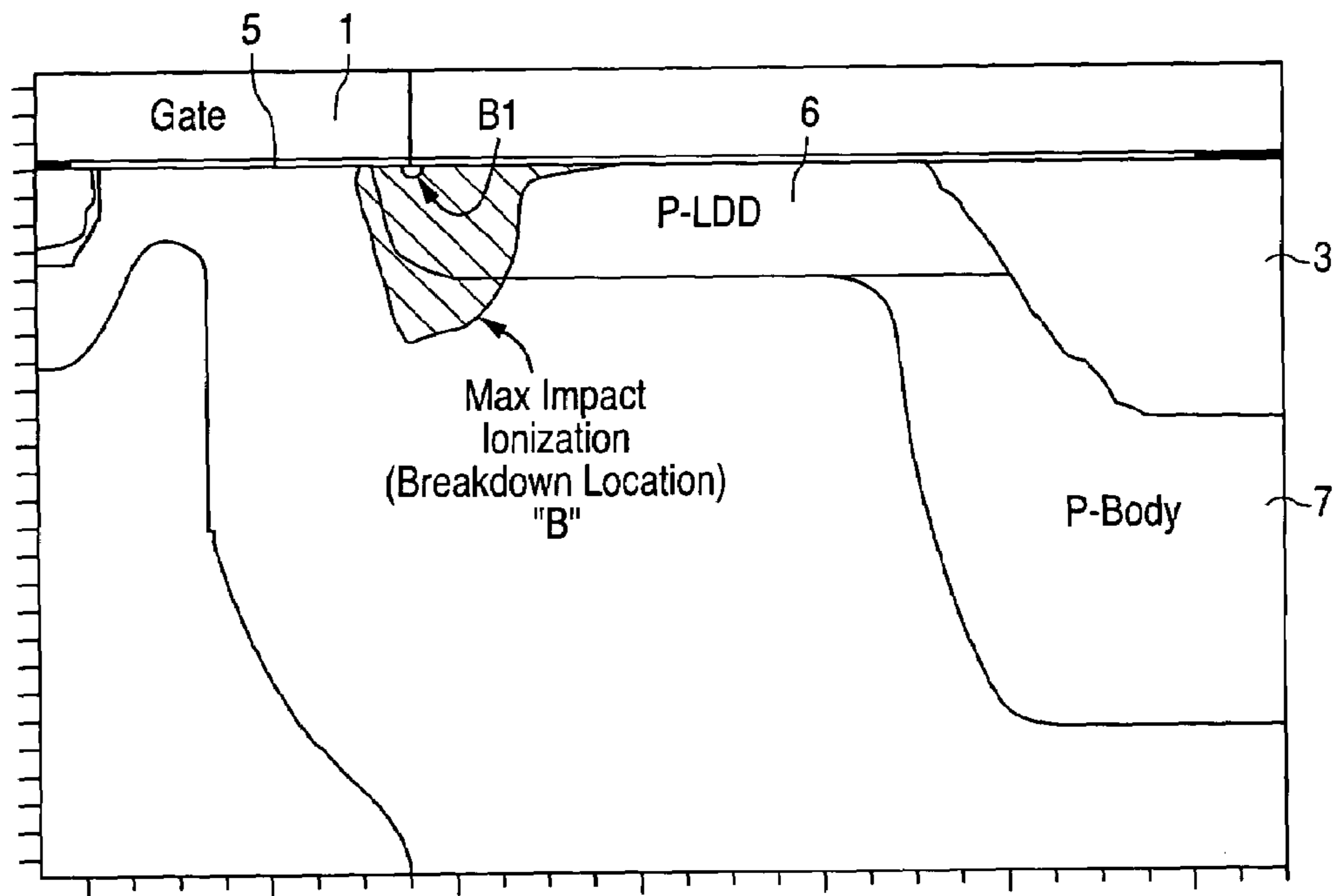
FIG. 5 (PRIOR ART)
