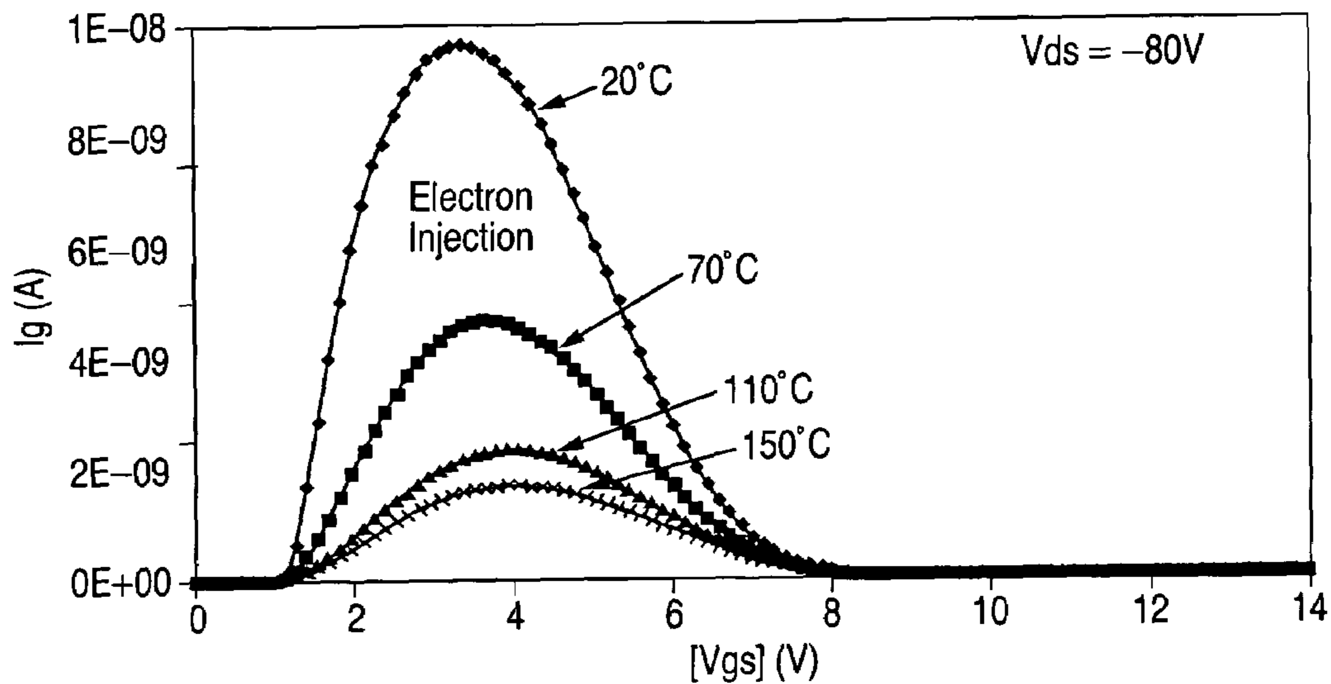
FIG. 5 (PRIOR ART)
