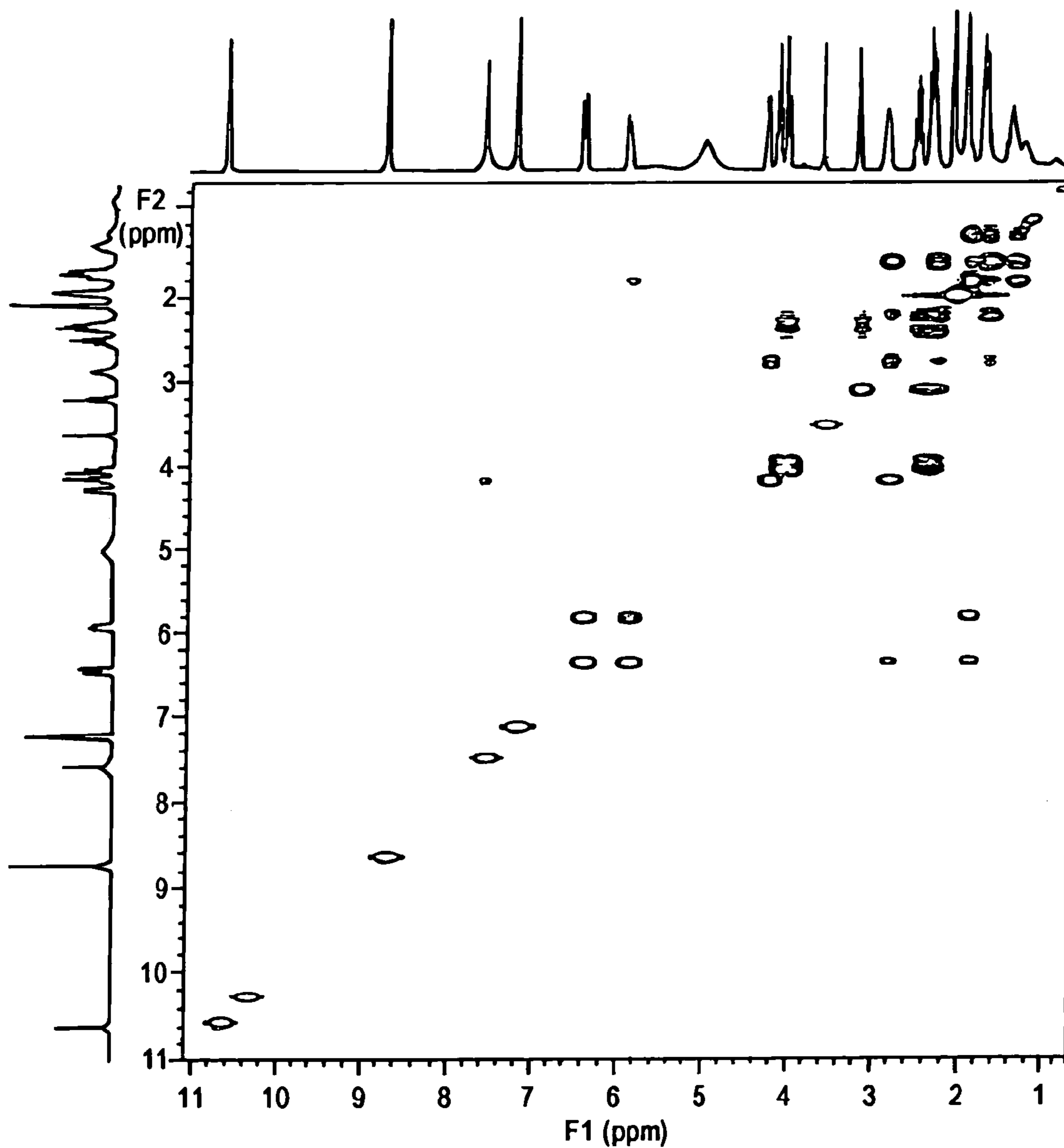
H,H-COSY of salinosporamide A (1), 300 MHz, d 5 -pyridine
