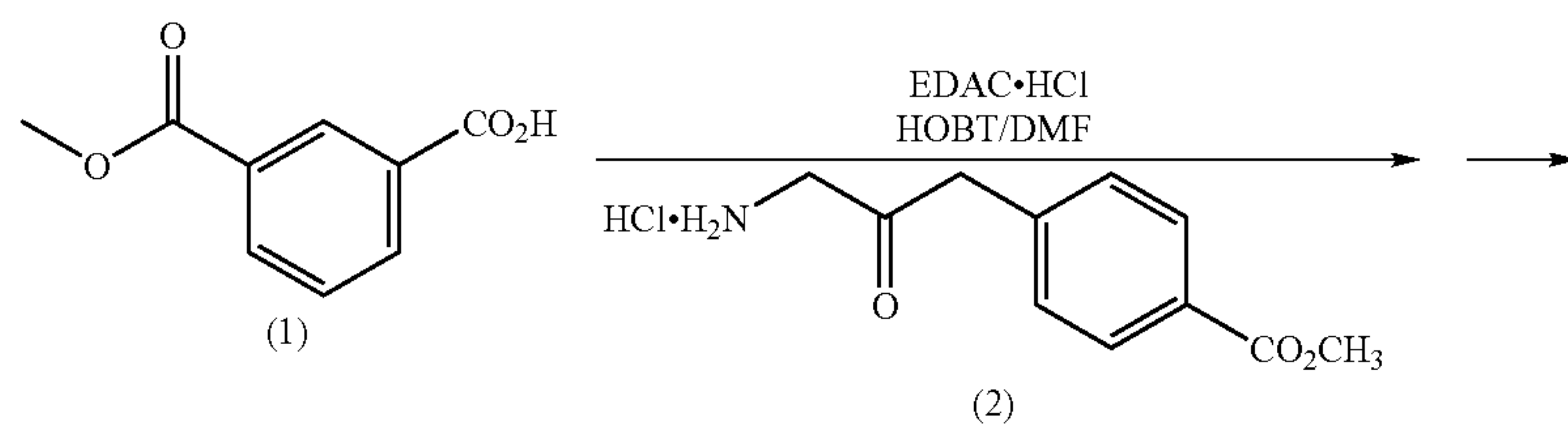
Scheme 10.
