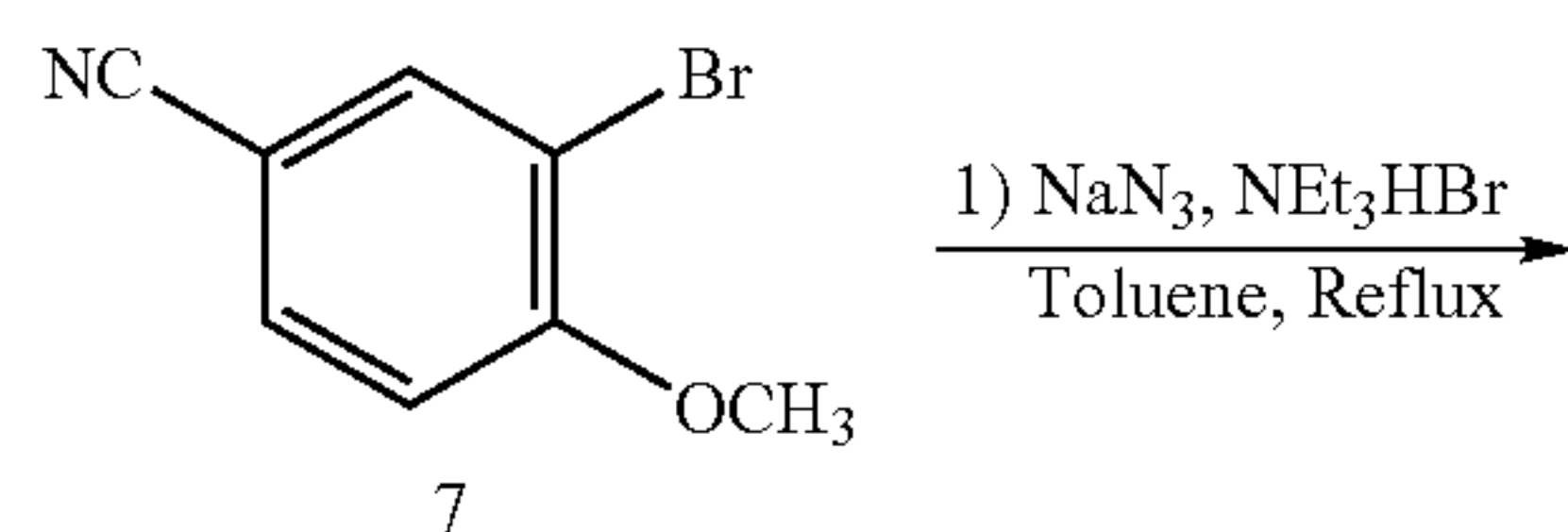
Scheme 2.
