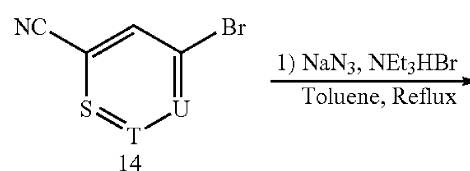
Scheme 3.
