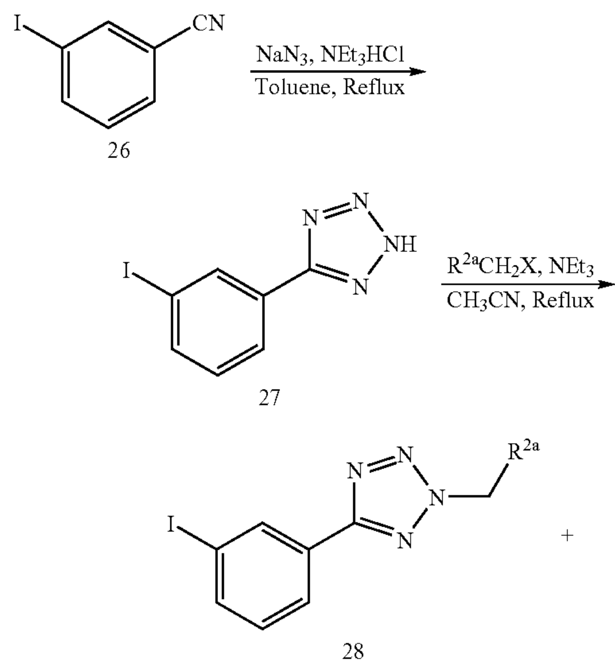
Scheme 5.
