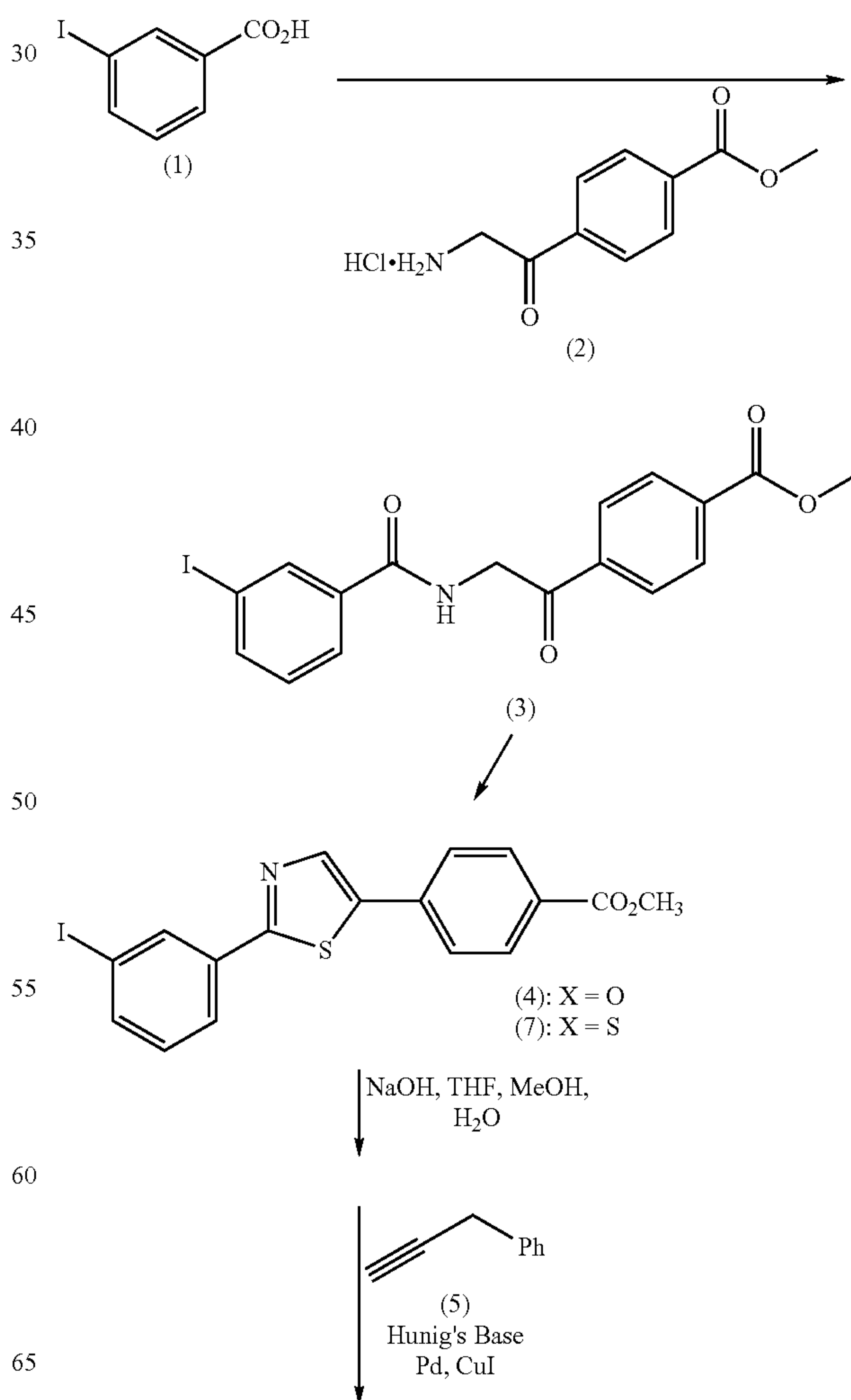
Scheme 6.
