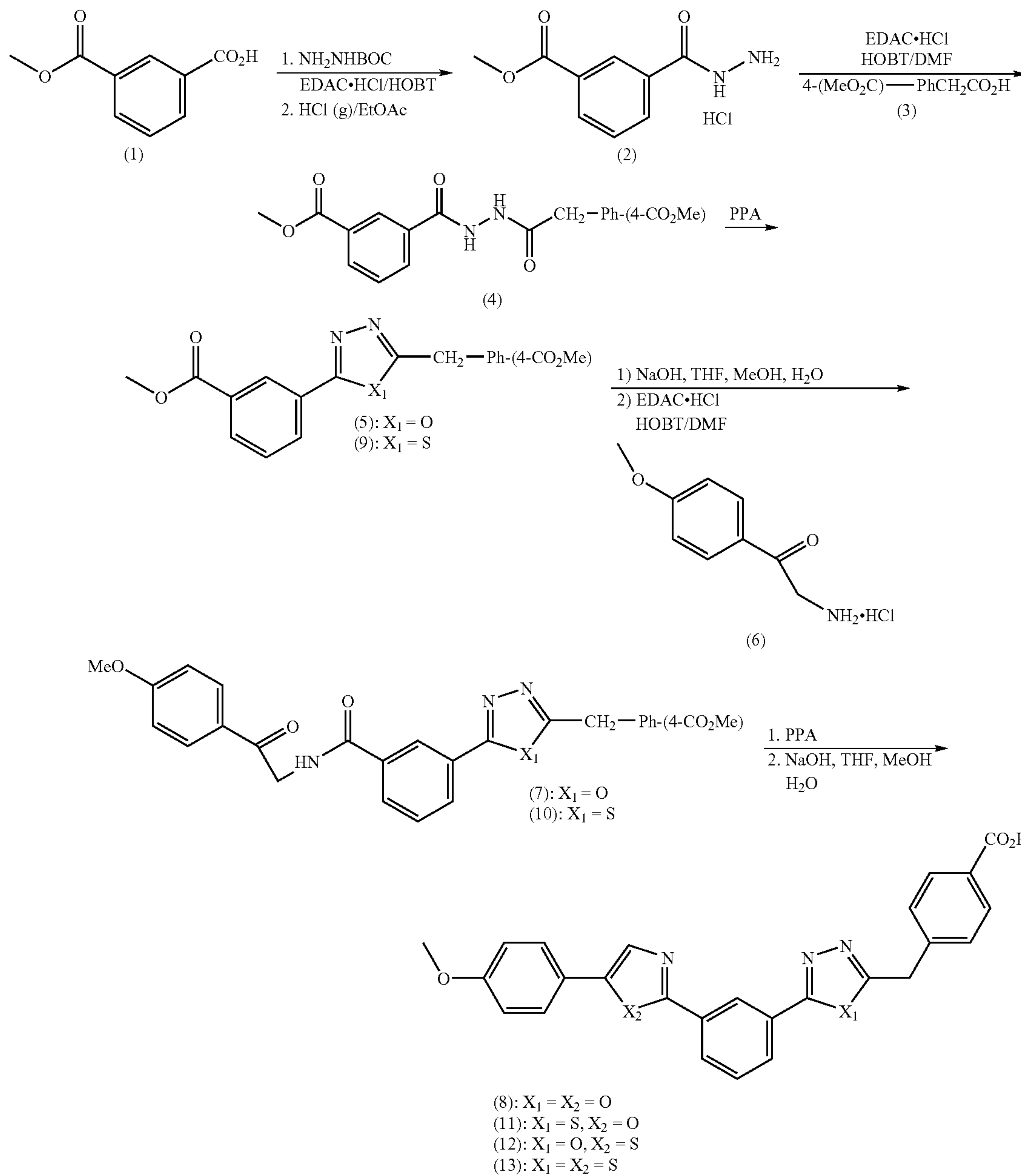
Scheme 9.
