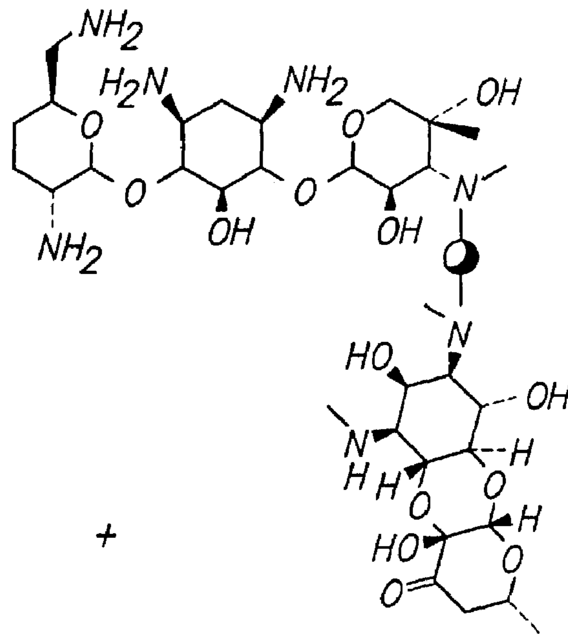
Formula LI-B
