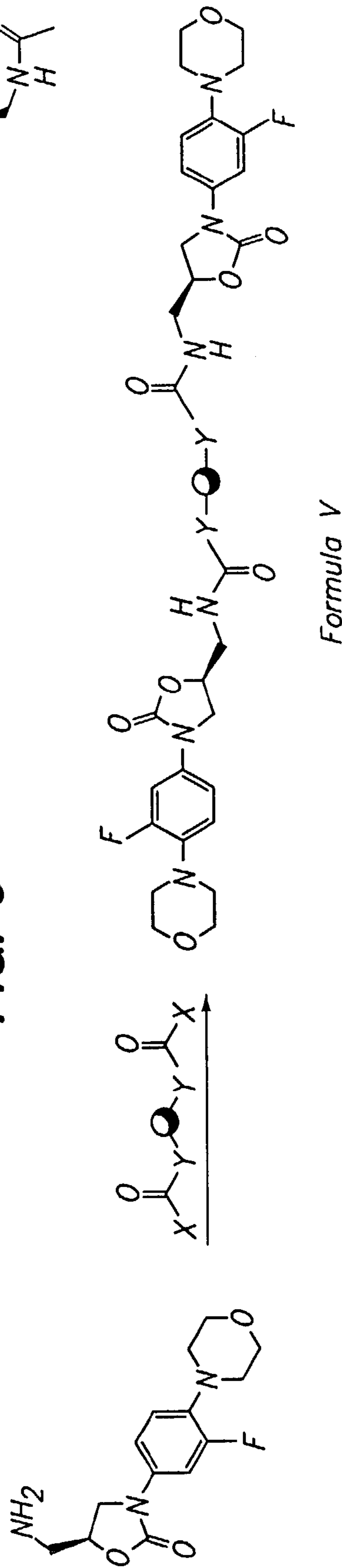
Formula IV
