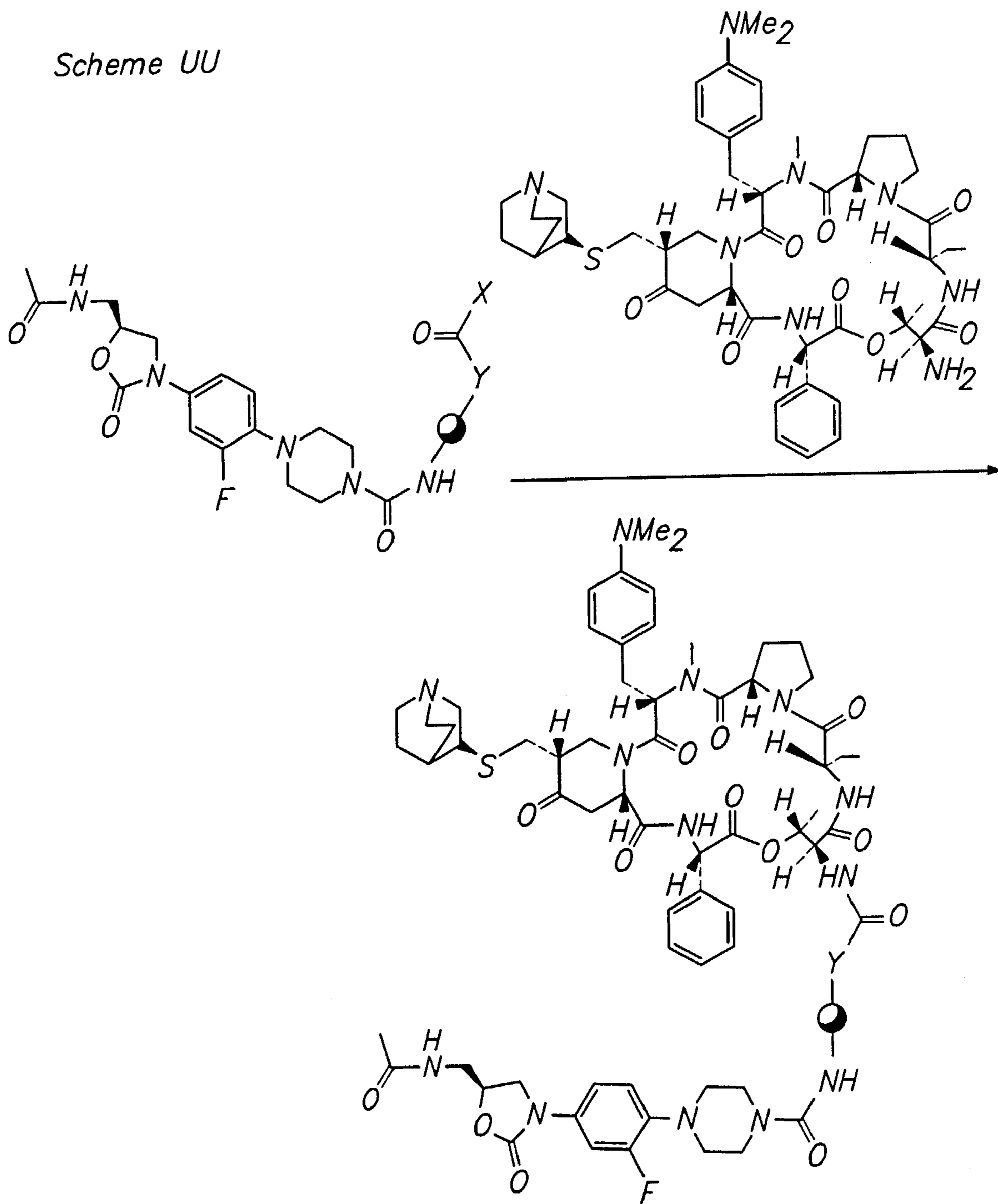
Formula XLVII
