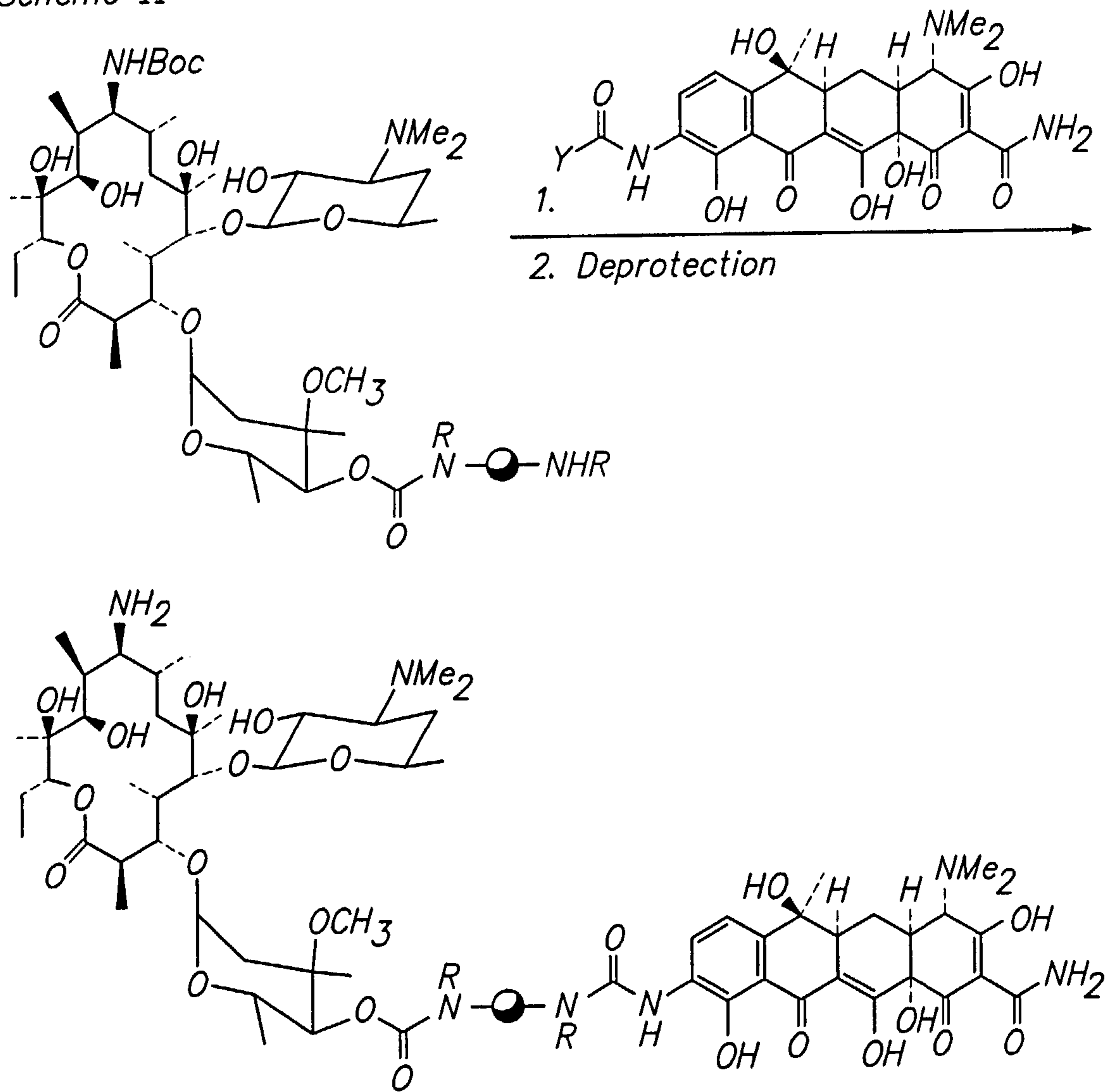
Scheme II
