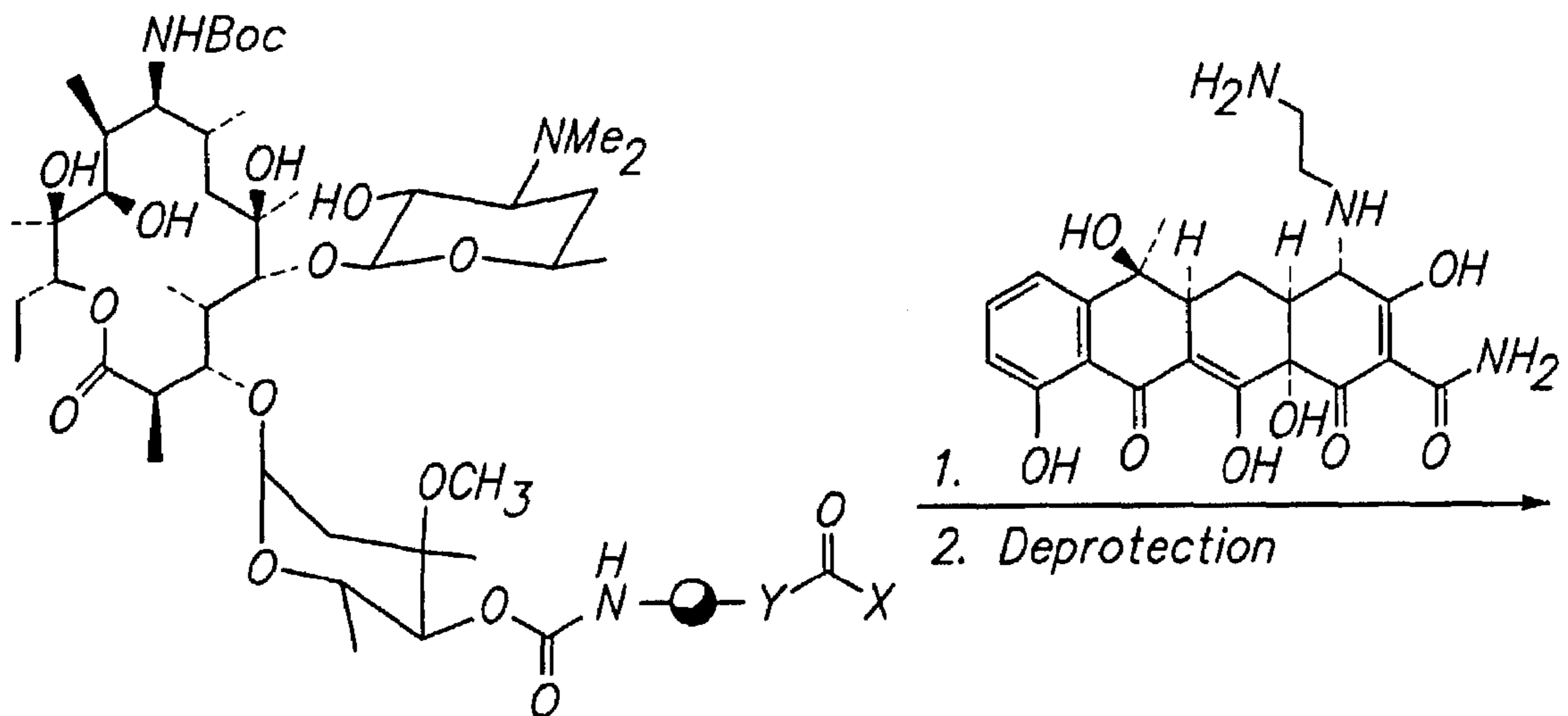
Scheme HH
