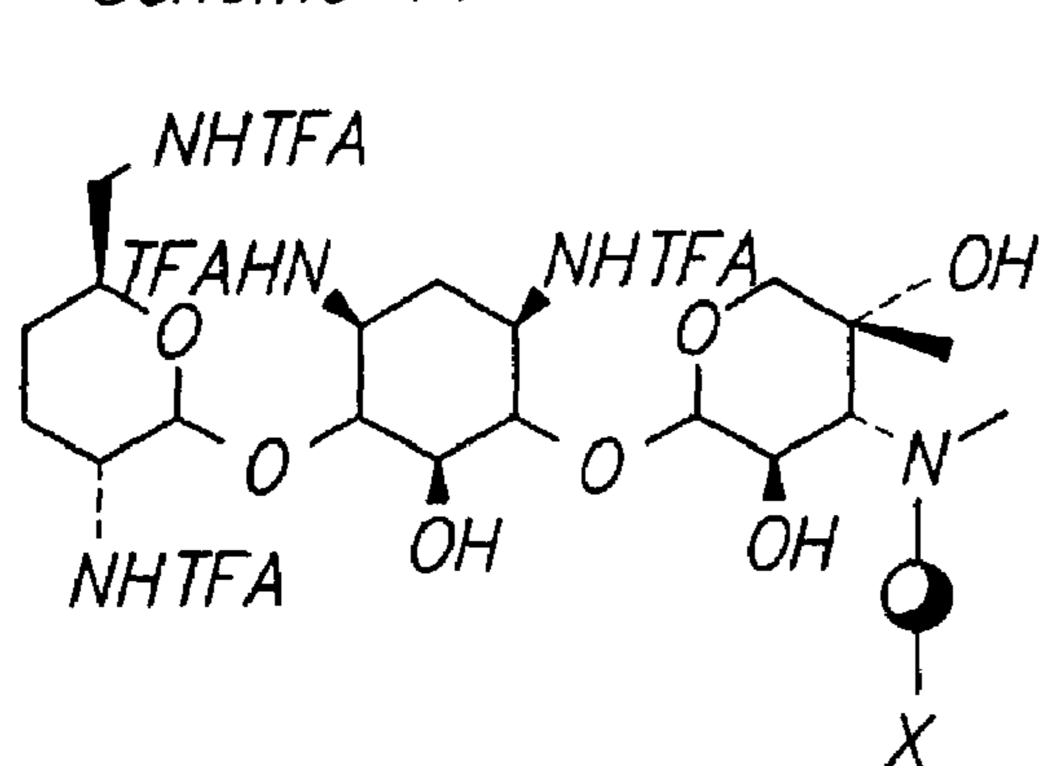
Scheme YY
