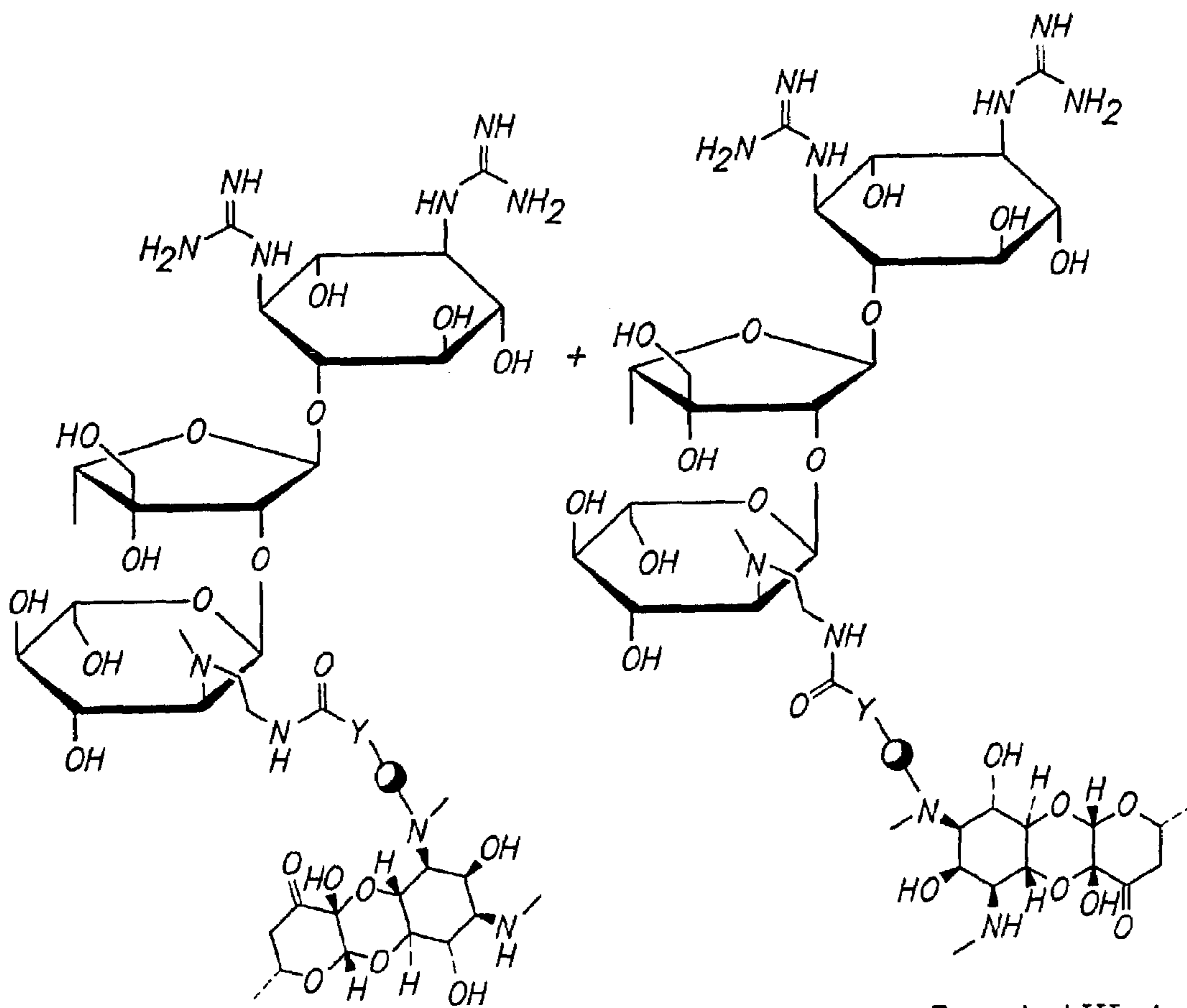
Formula LIII-A
