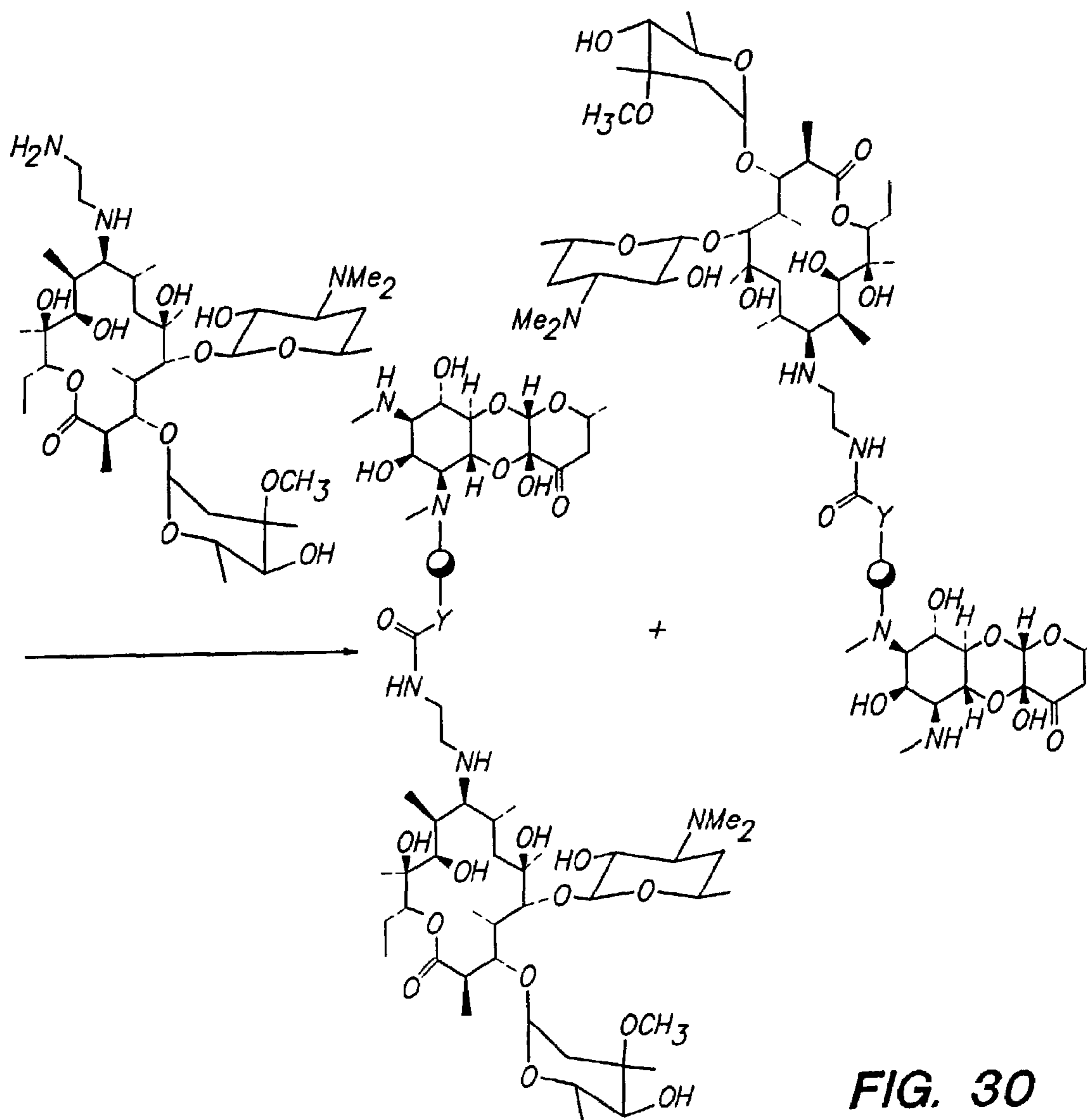
Formula XXXI
