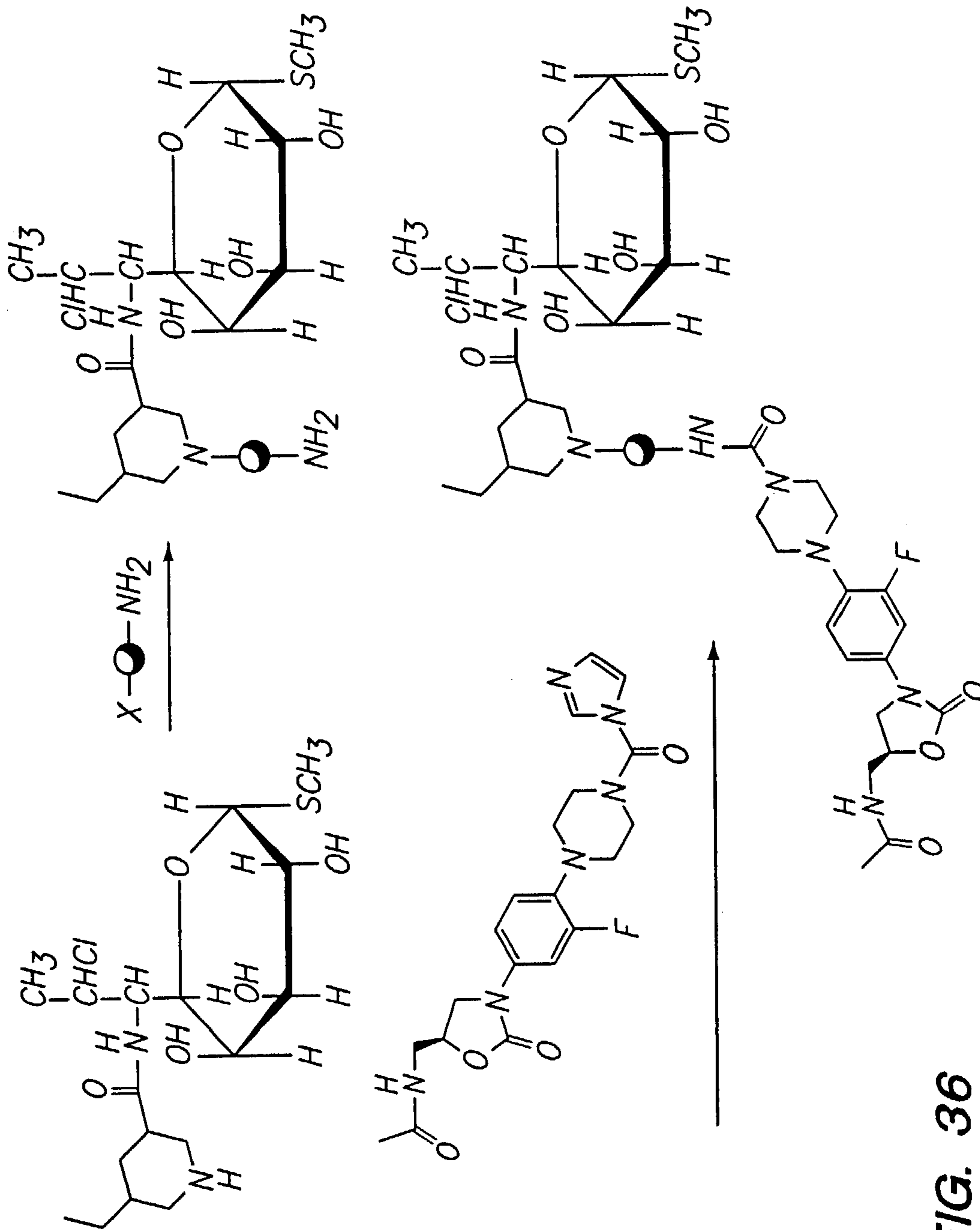
Scheme KK
