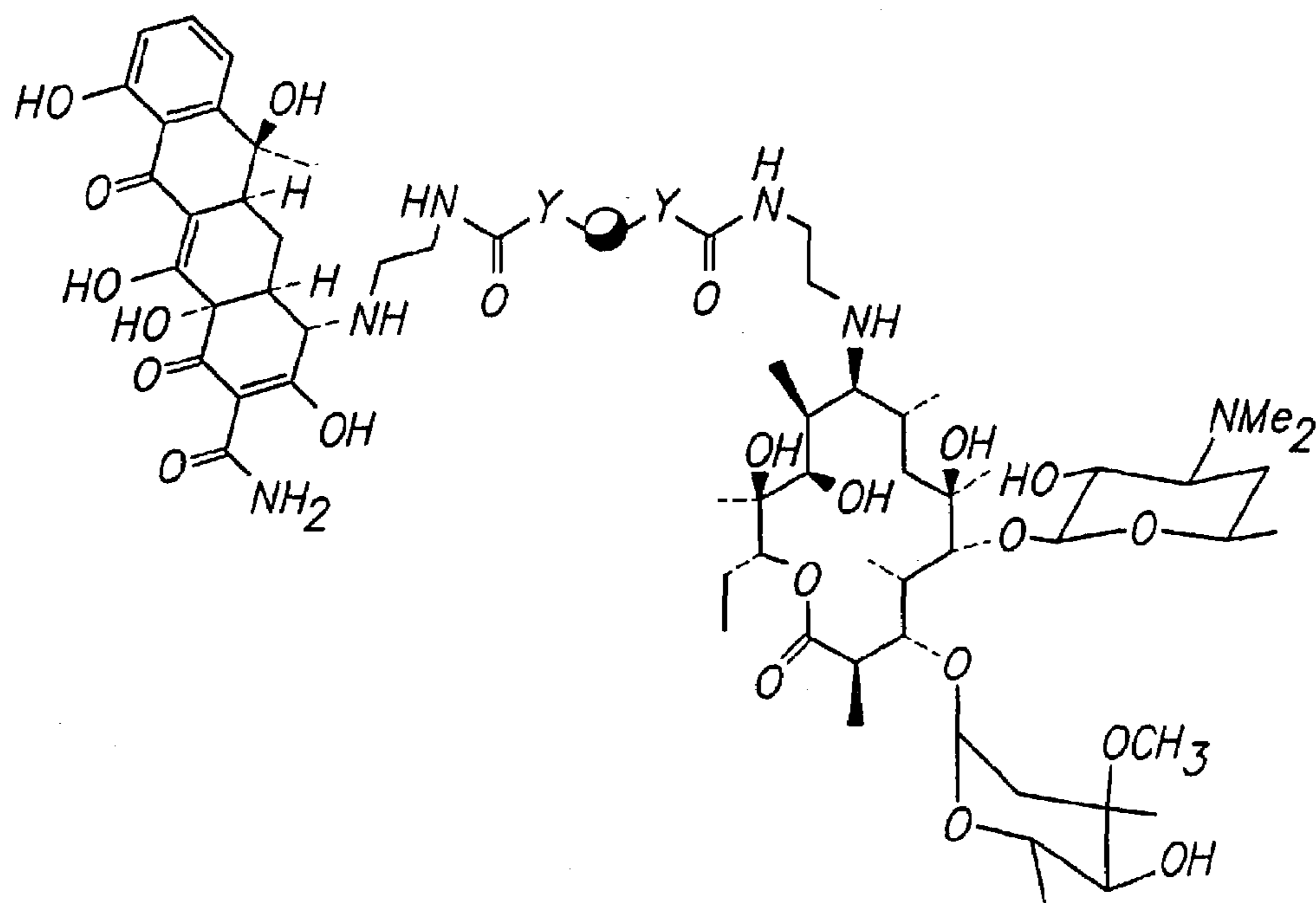
Formula XXXIII
