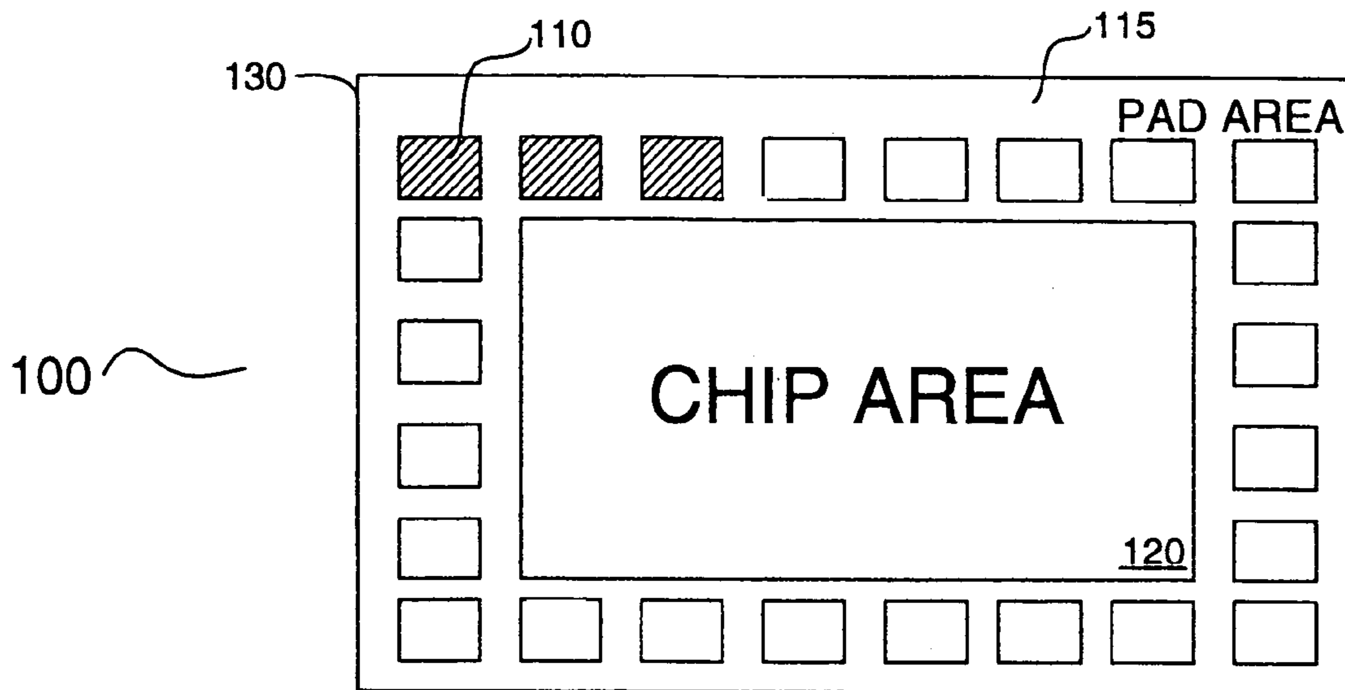
Fig. 1 (Prior Art)
