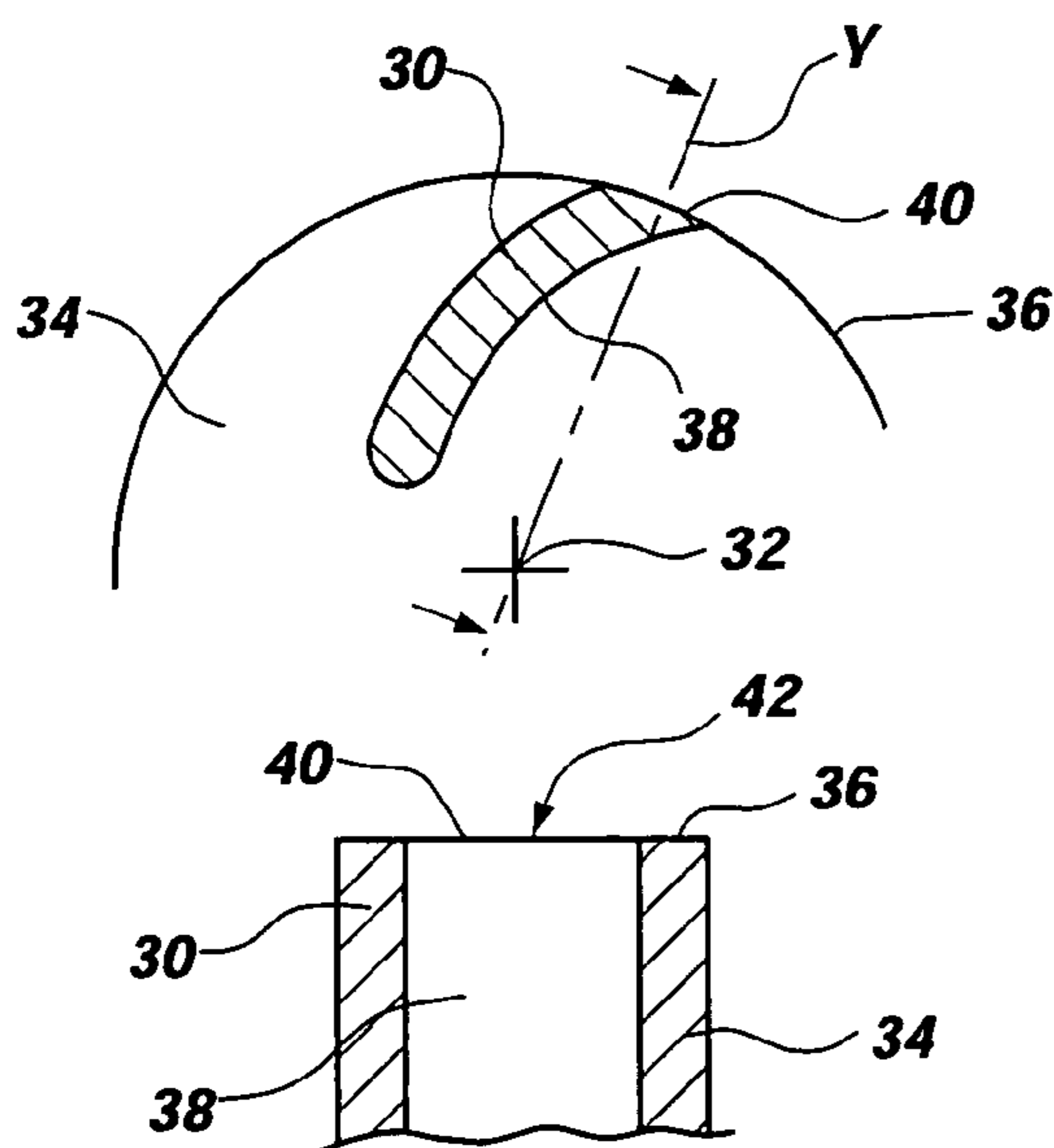
FIG. 3 (PRIOR ART)
