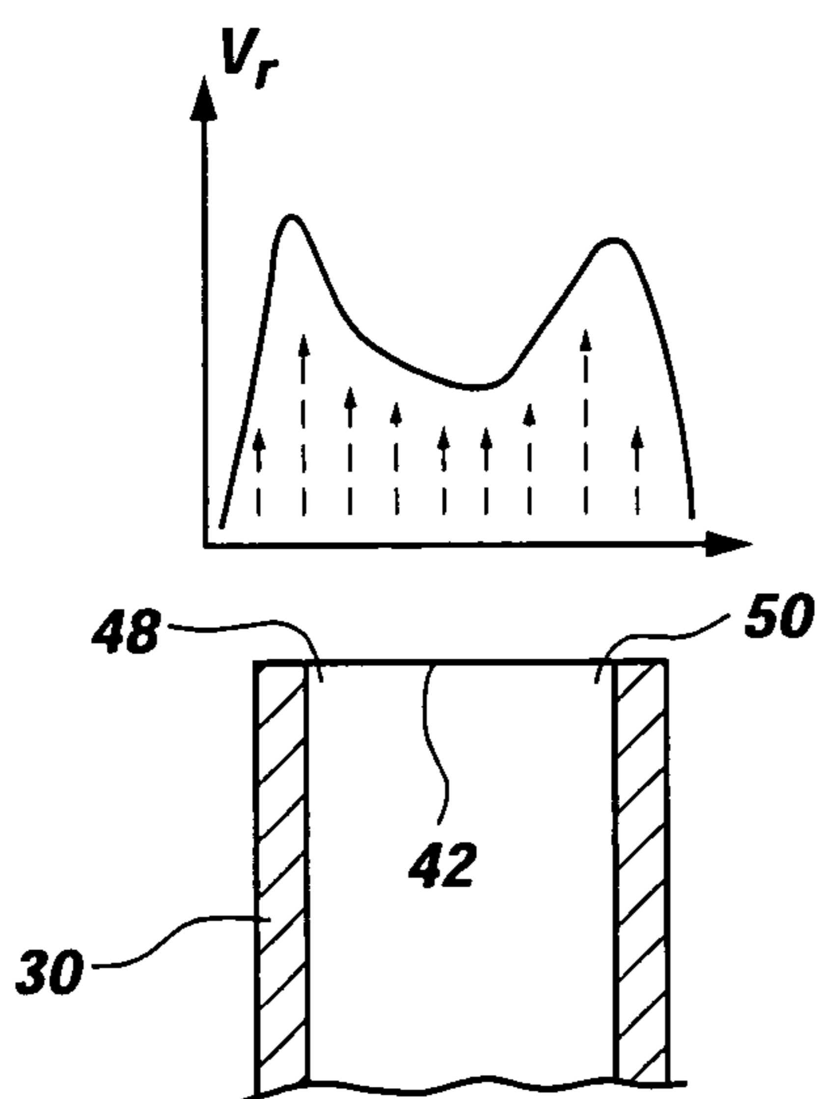
FIG. 5 (PRIOR ART)
