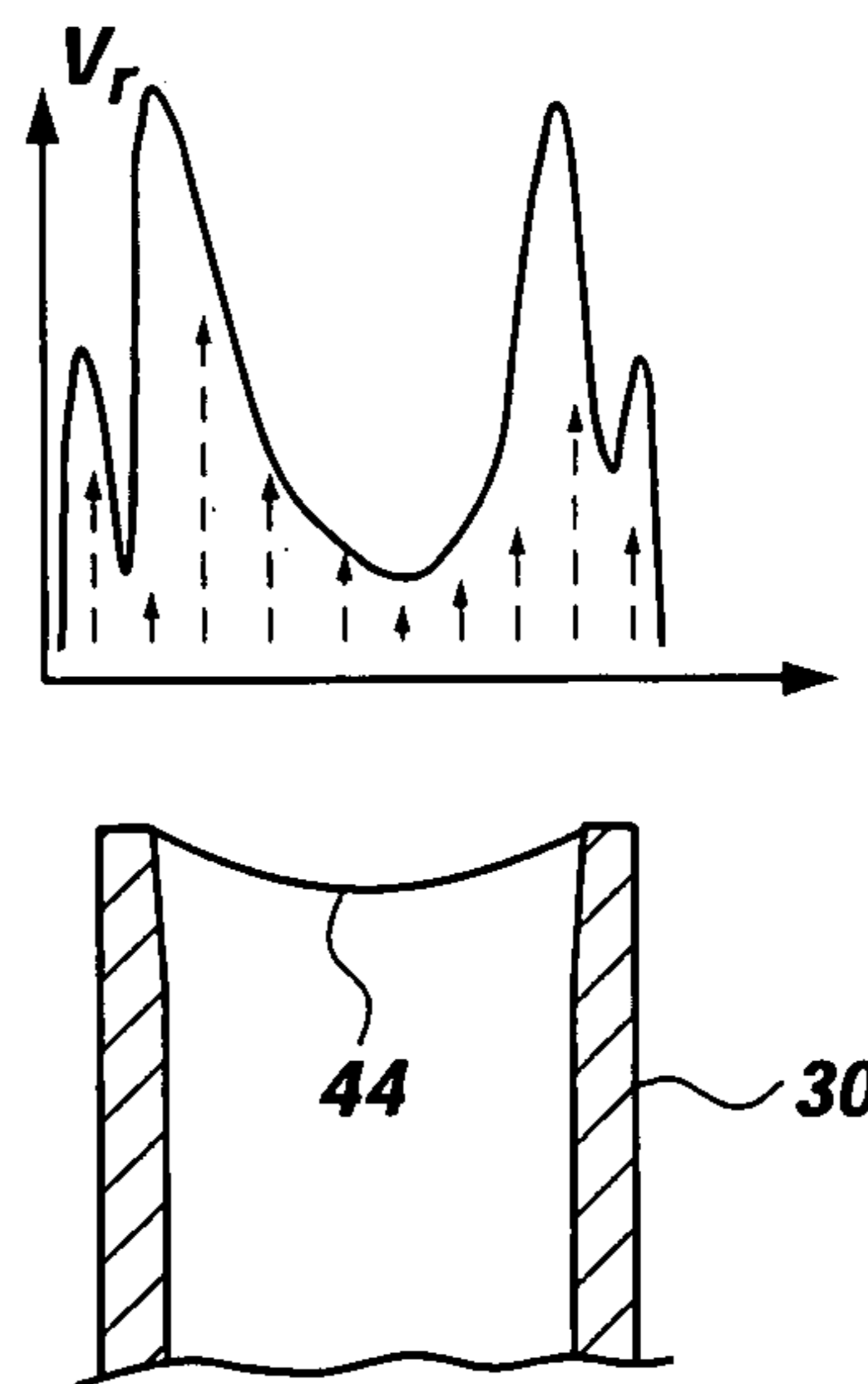
FIG. 6 (PRIOR ART)
