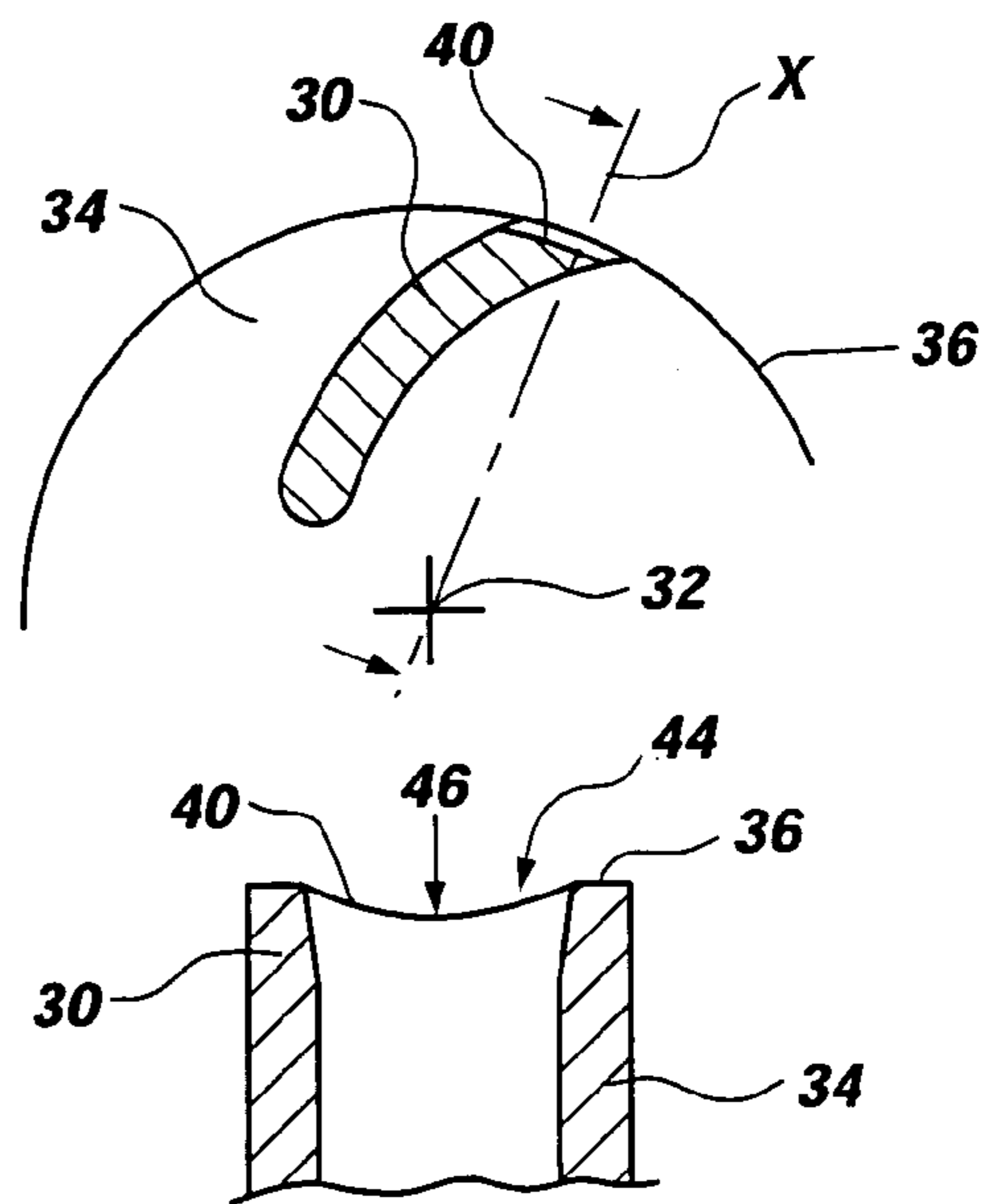
FIG. 4 (PRIOR ART)
