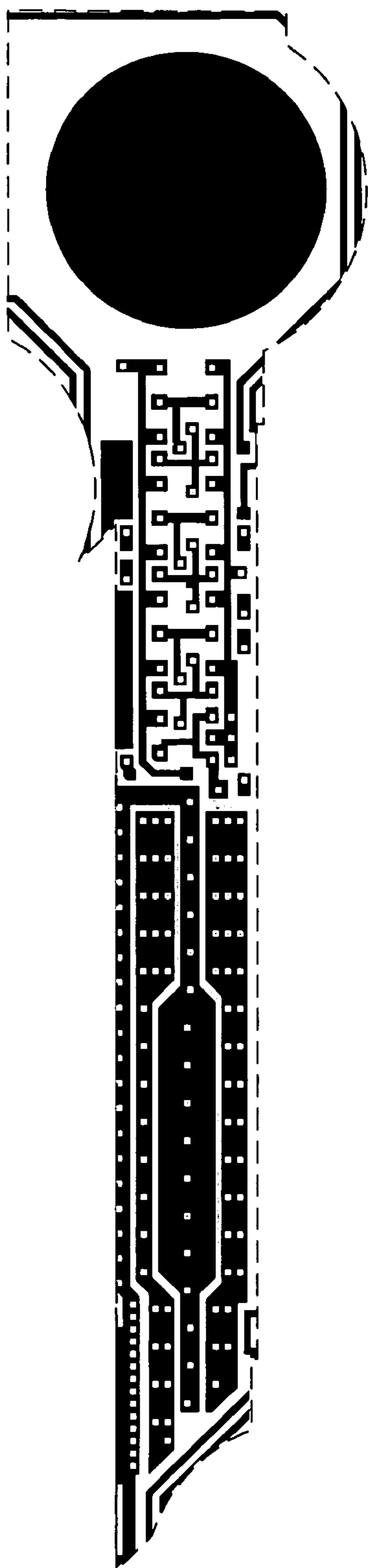
Metal 1 mask
