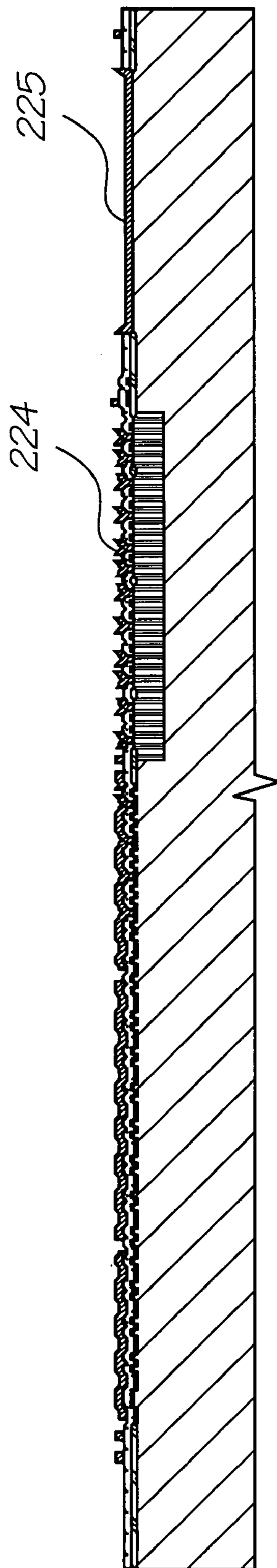
Deposit Metal 1
