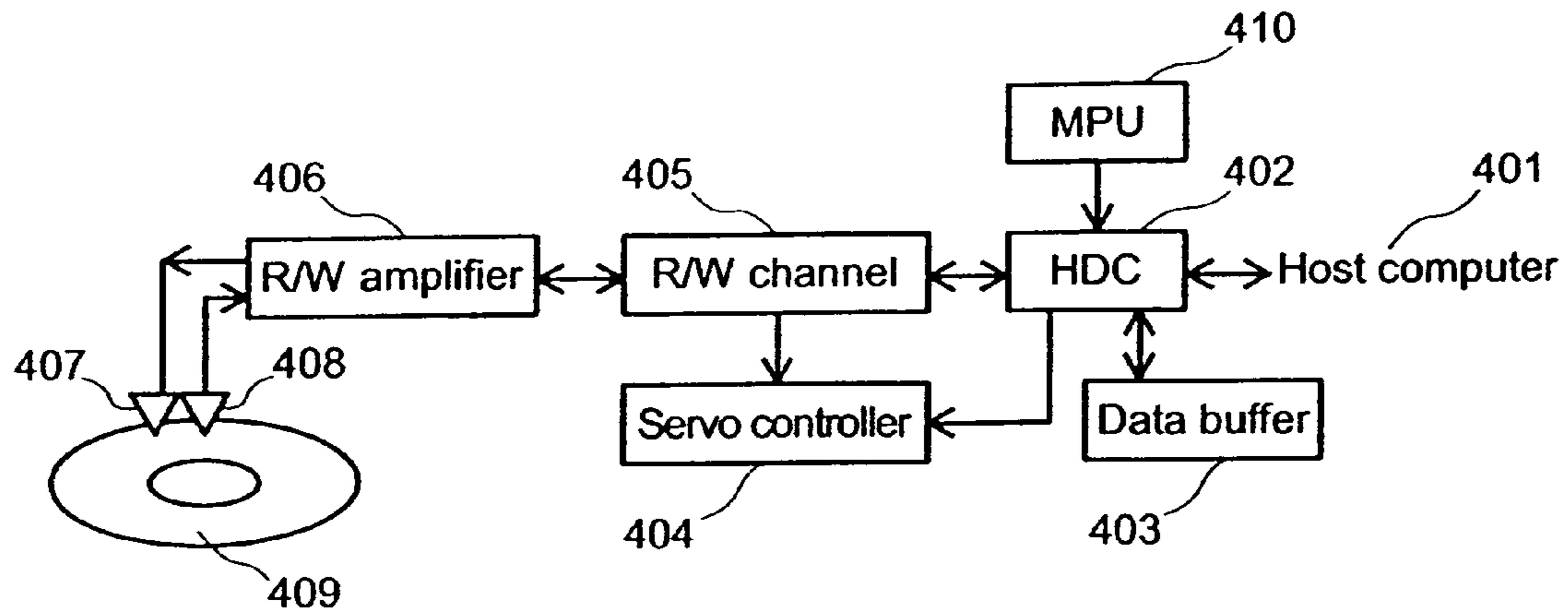
FIG.4 Prior Art
