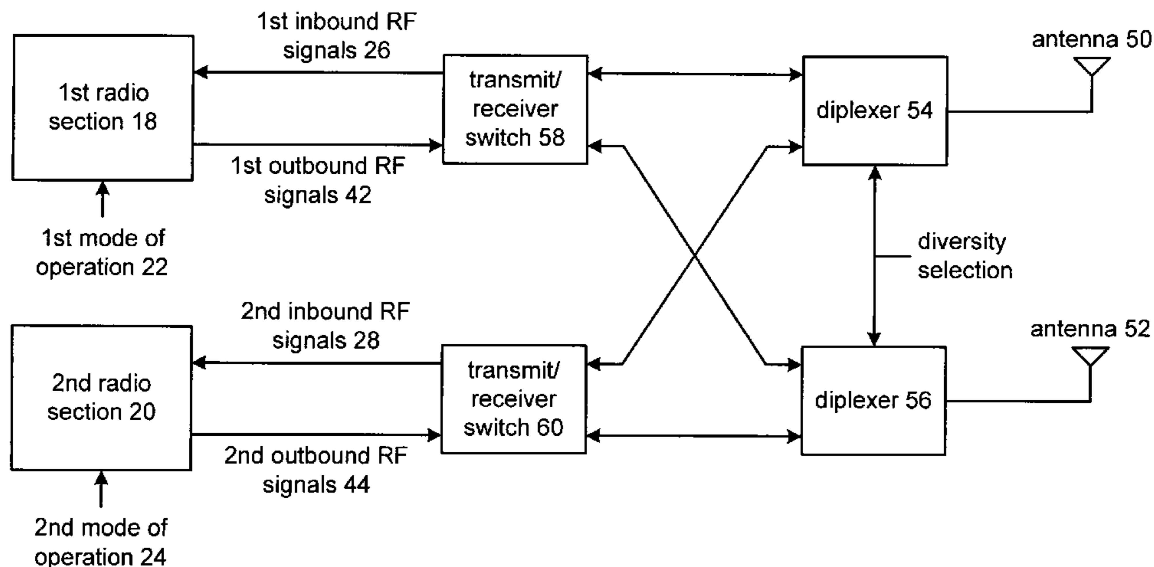
diversity antenna arrangement
