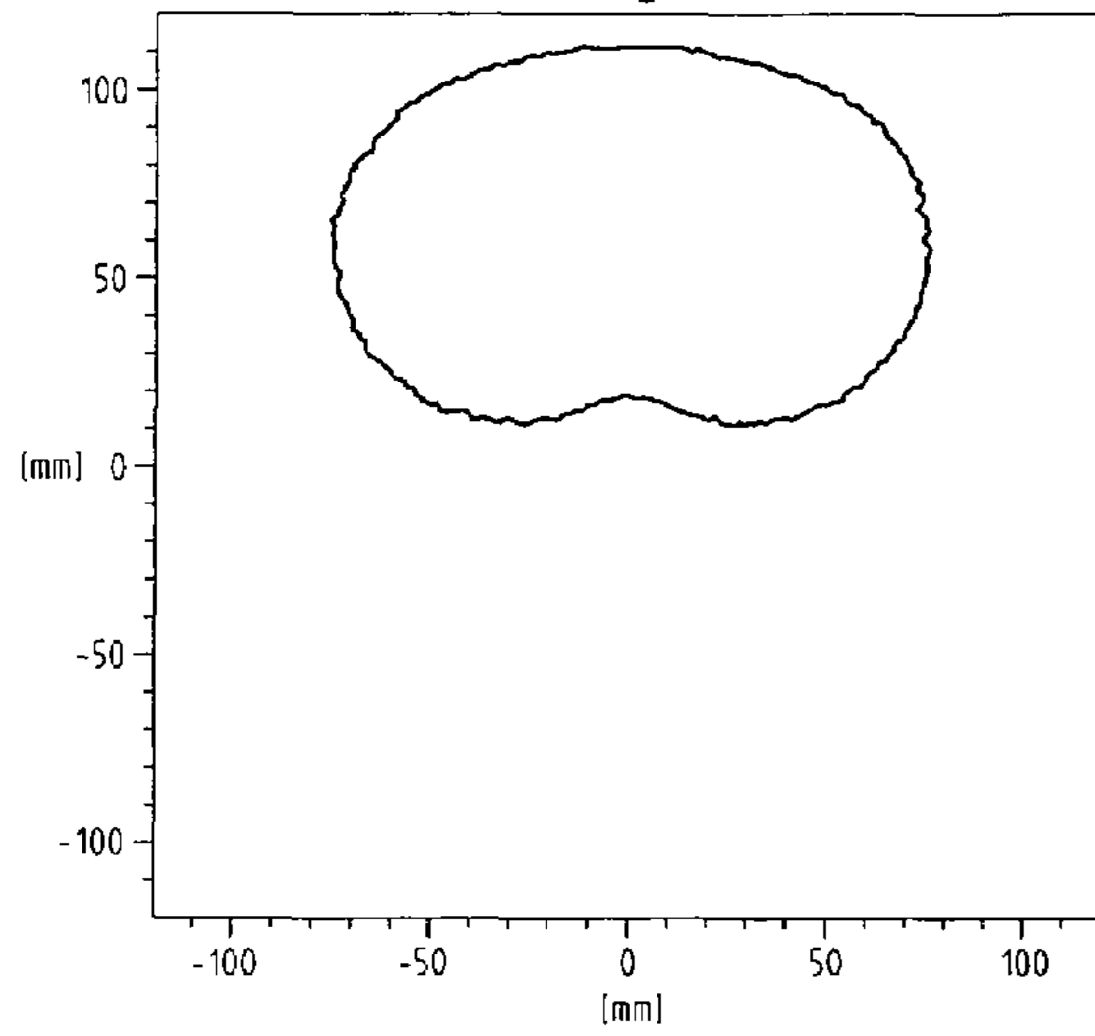
off-axis segment M1
