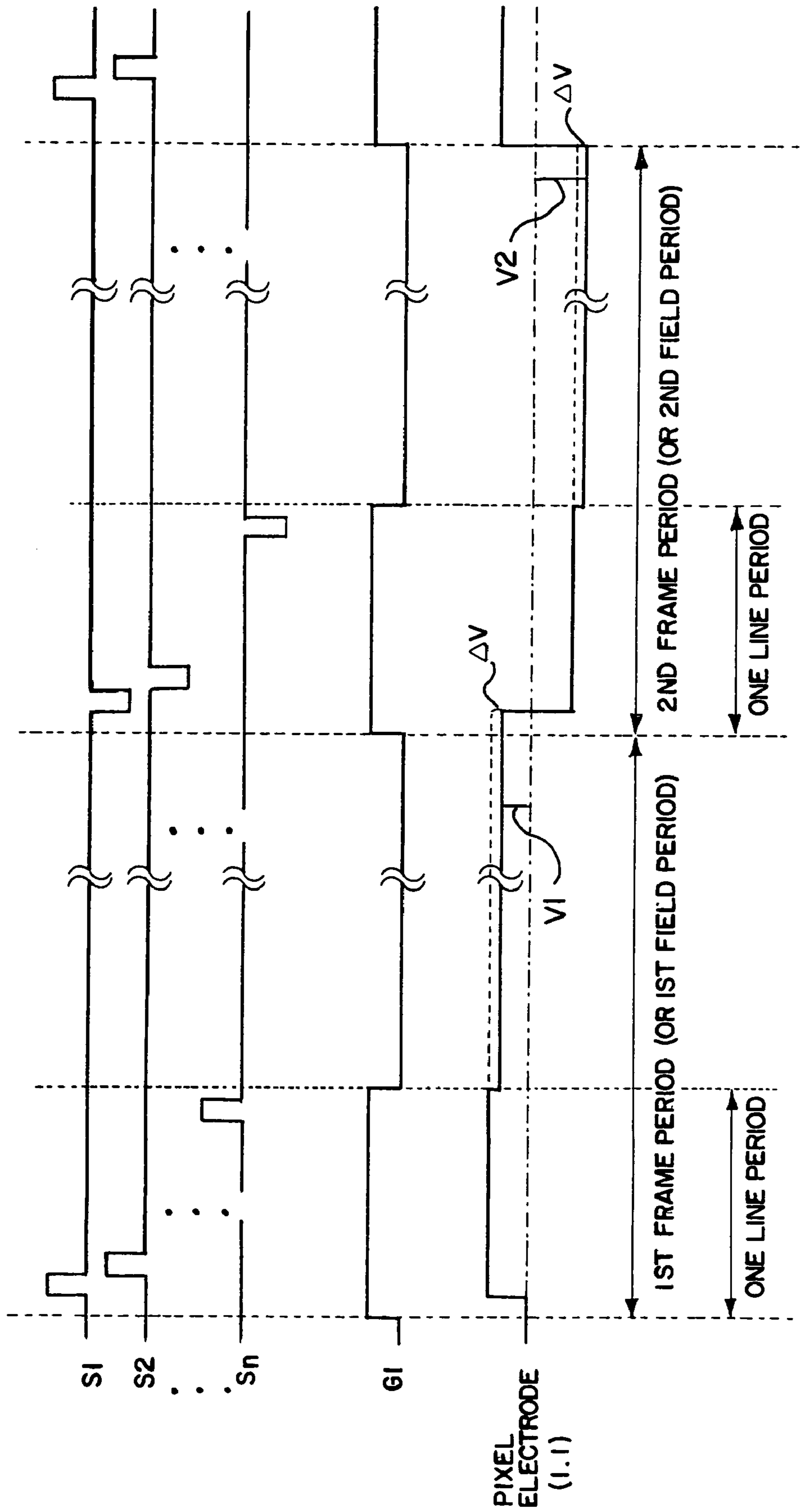
FIG. 24 PRIOR ART
