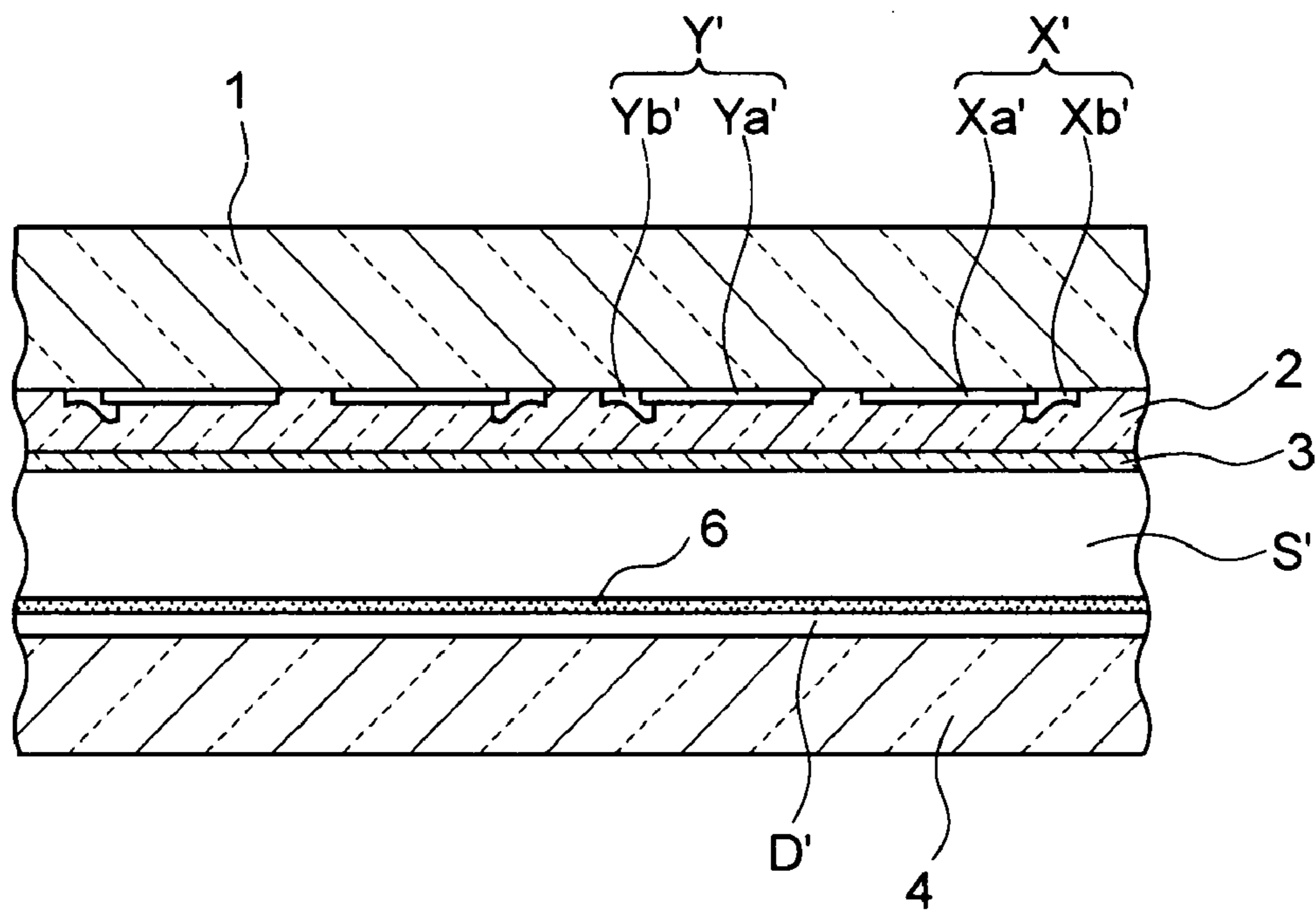
II - II CROSS - SECTION
