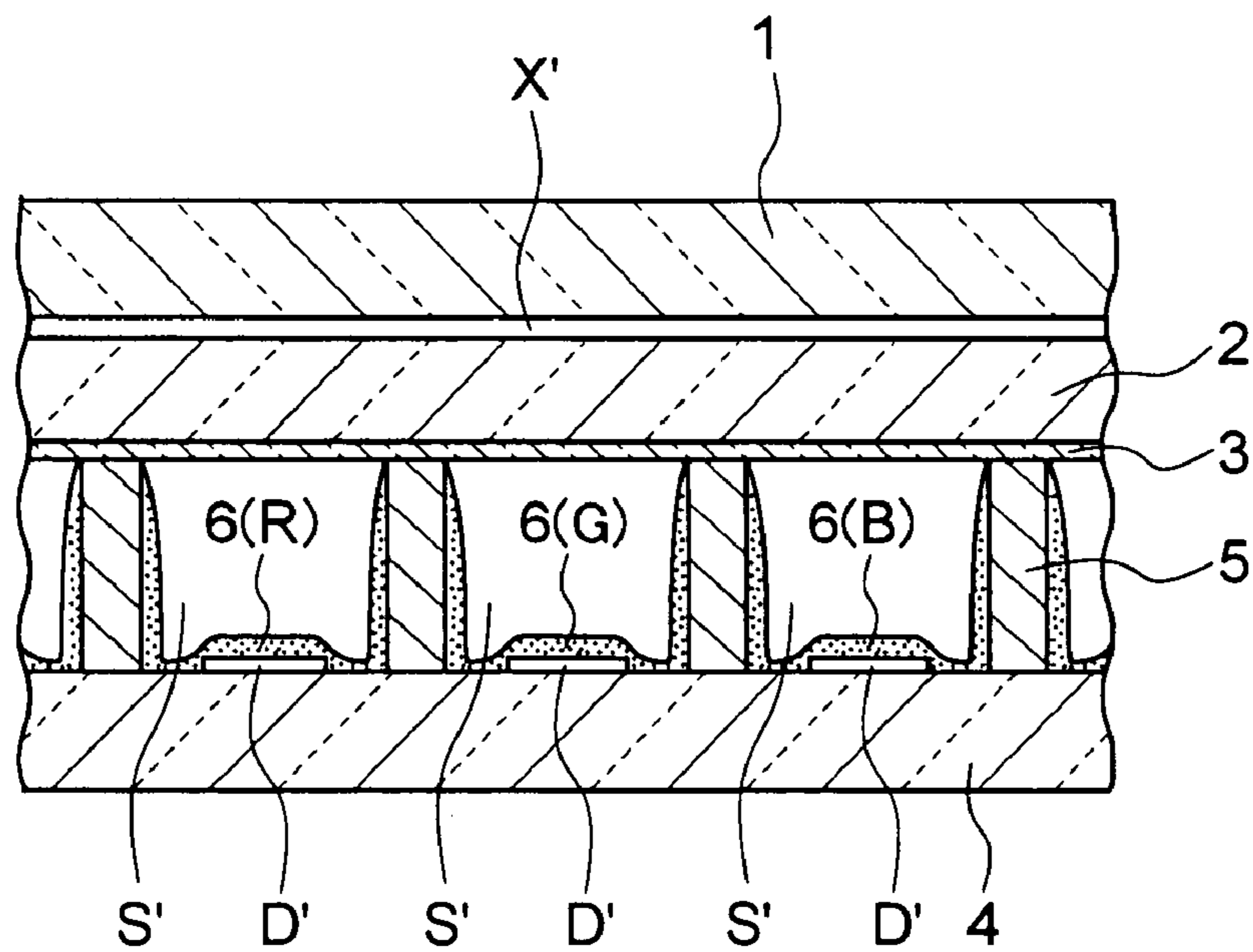
III - III CROSS - SECTION
