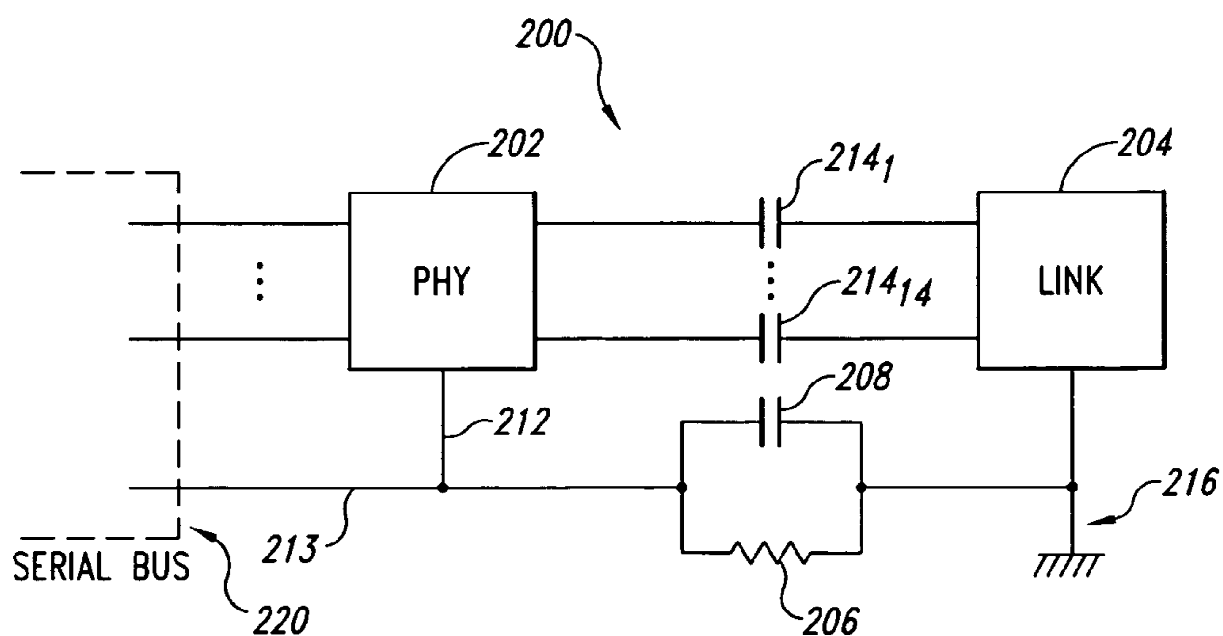
Fig. 2 (Prior Art)
