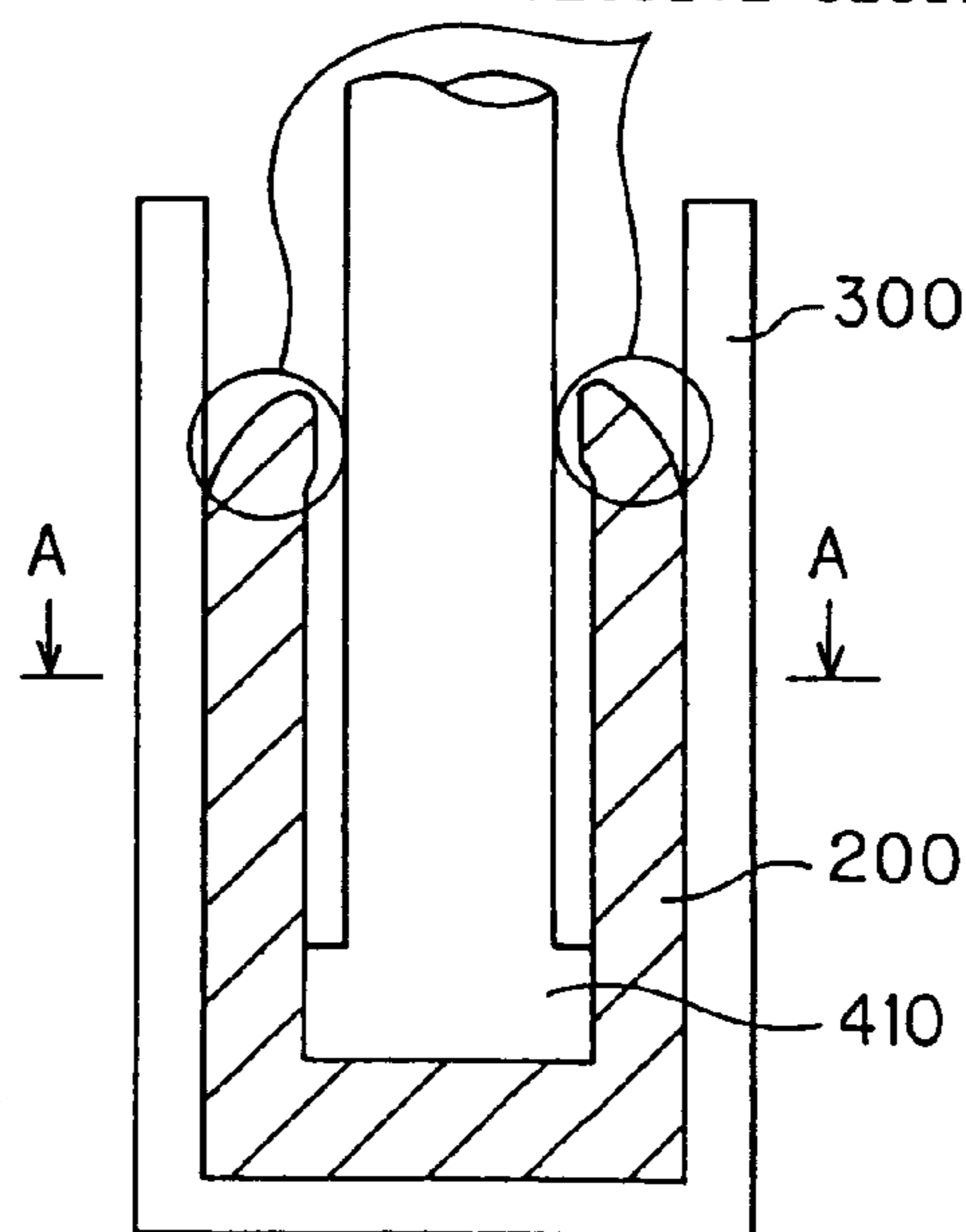
SHAPE-DEFECTIVE SECTION
