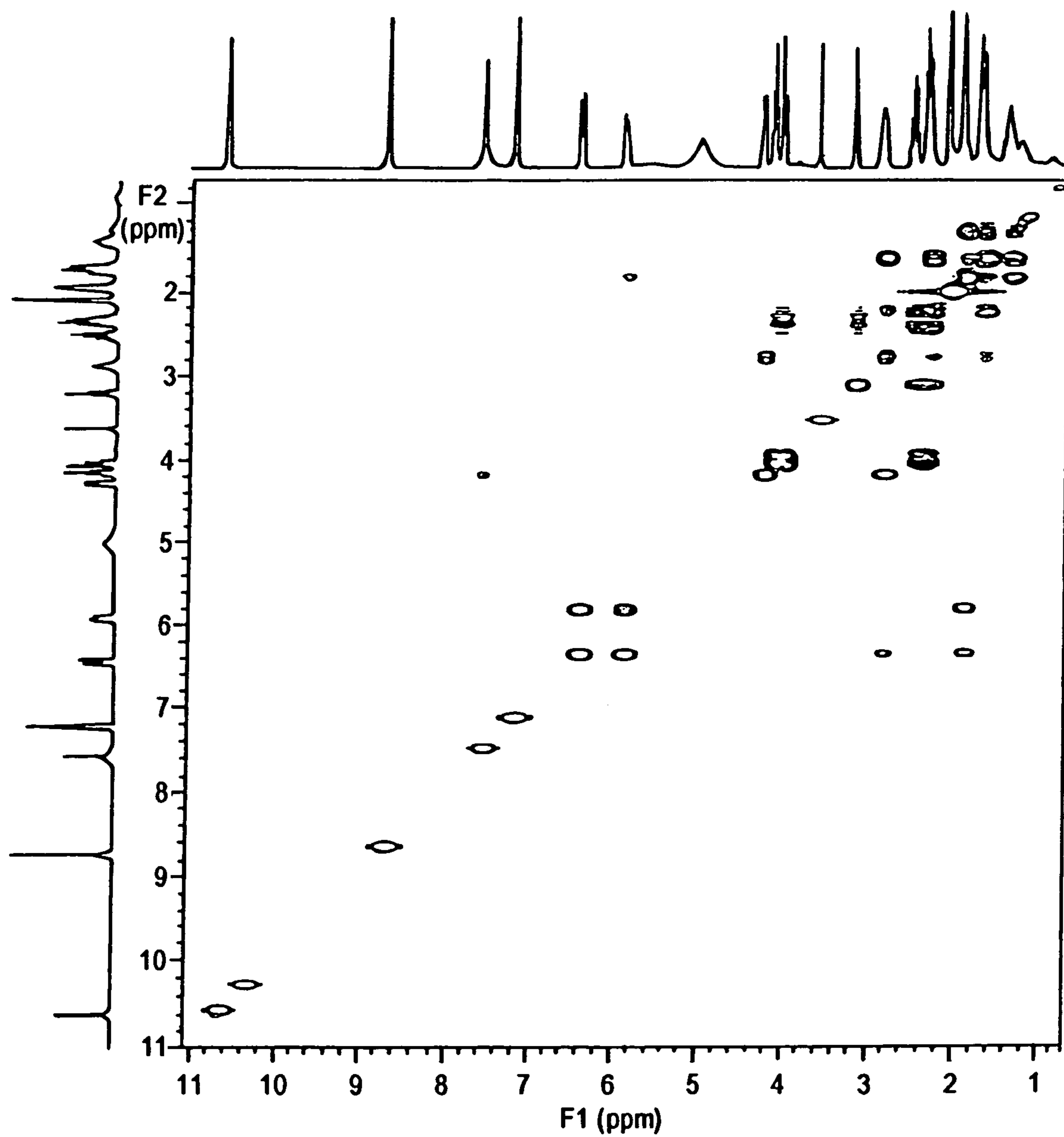
H,H-COSY of salinosporamide A (1), 300 MHz, d 5 -pyridine
