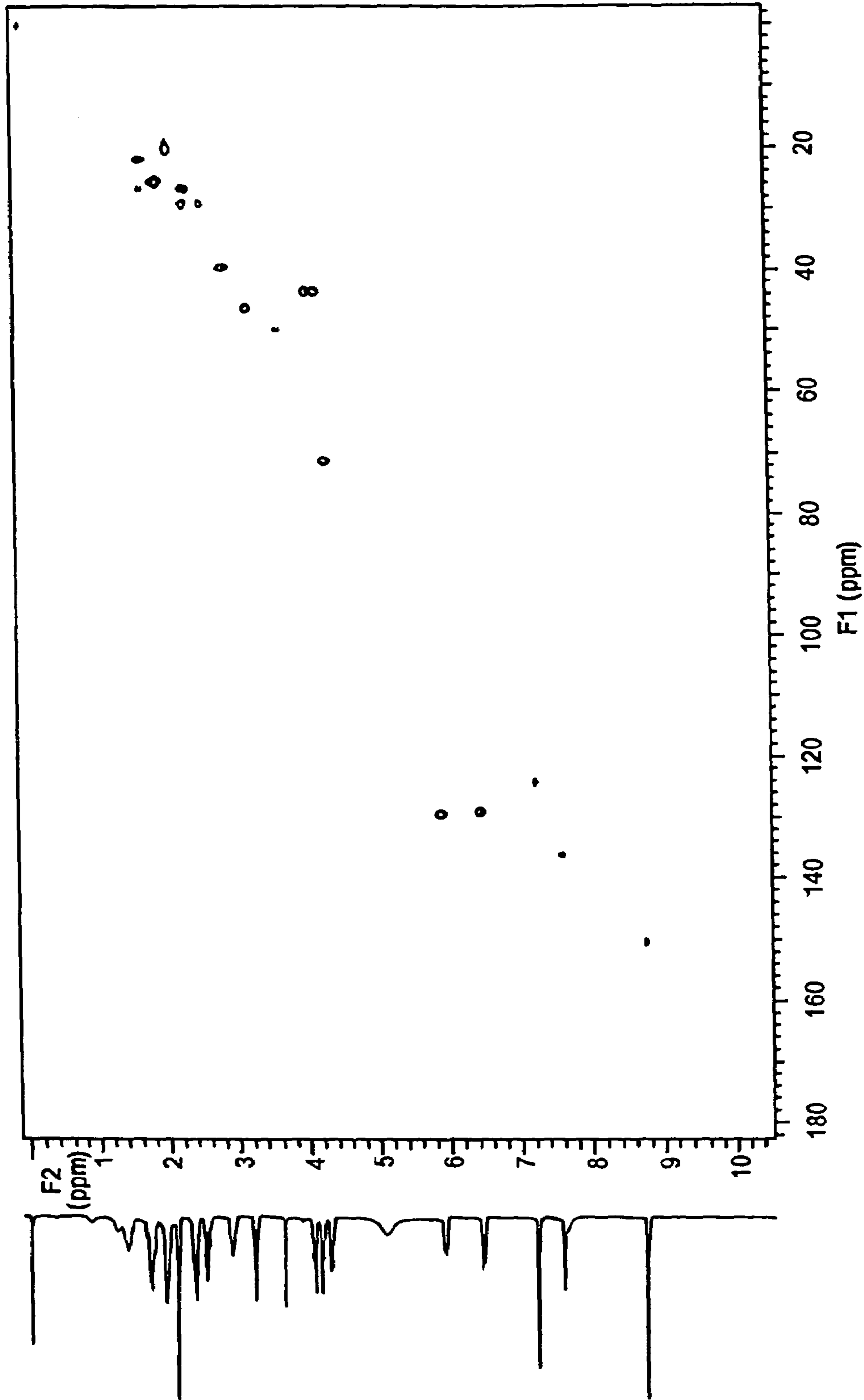
HMQC of salinosporamide A (1), 300 MHz, d5-pyridine
