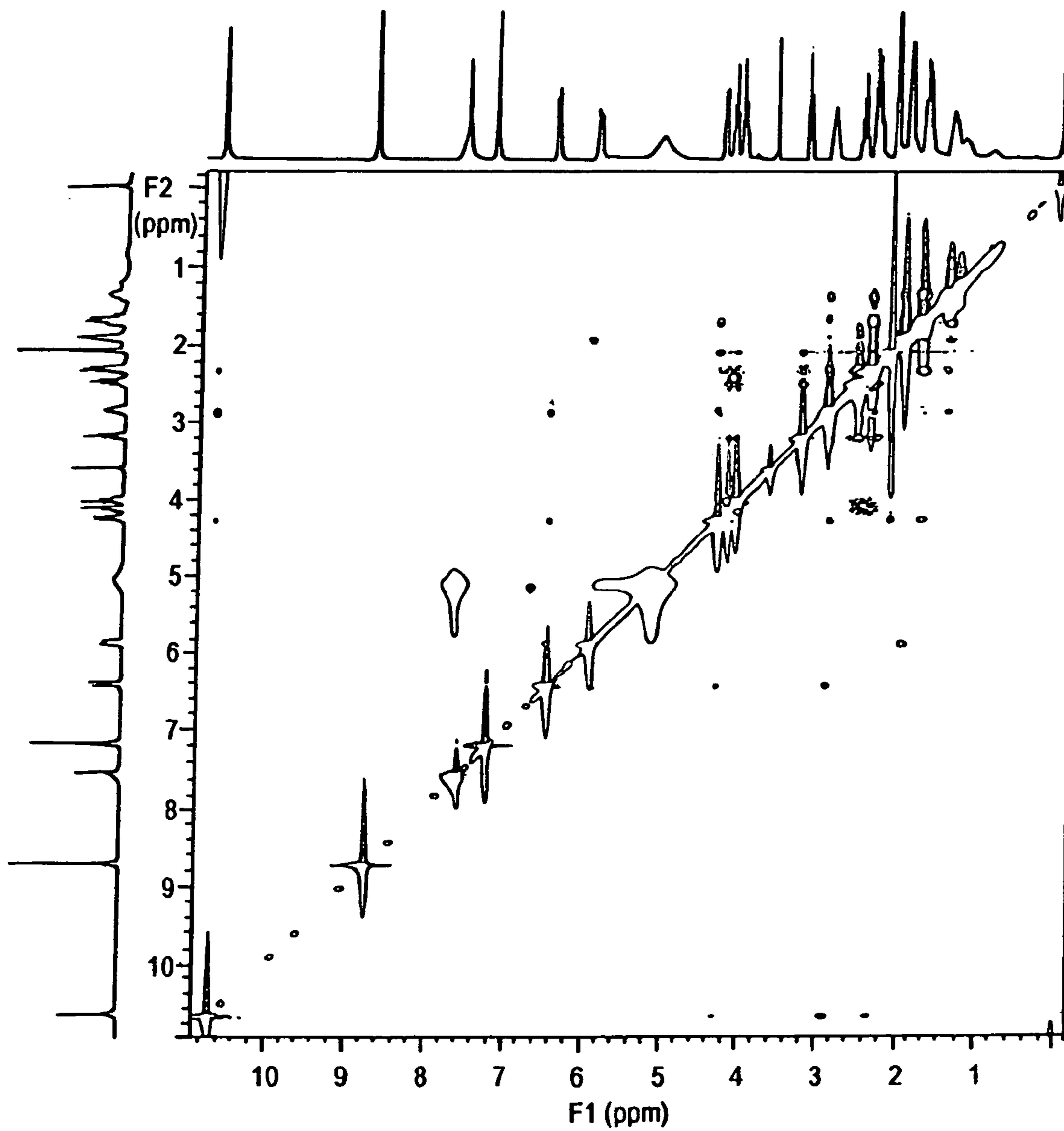
NOESY of salinosporamide A (1), 300 MHz, d 5 -pyridine
