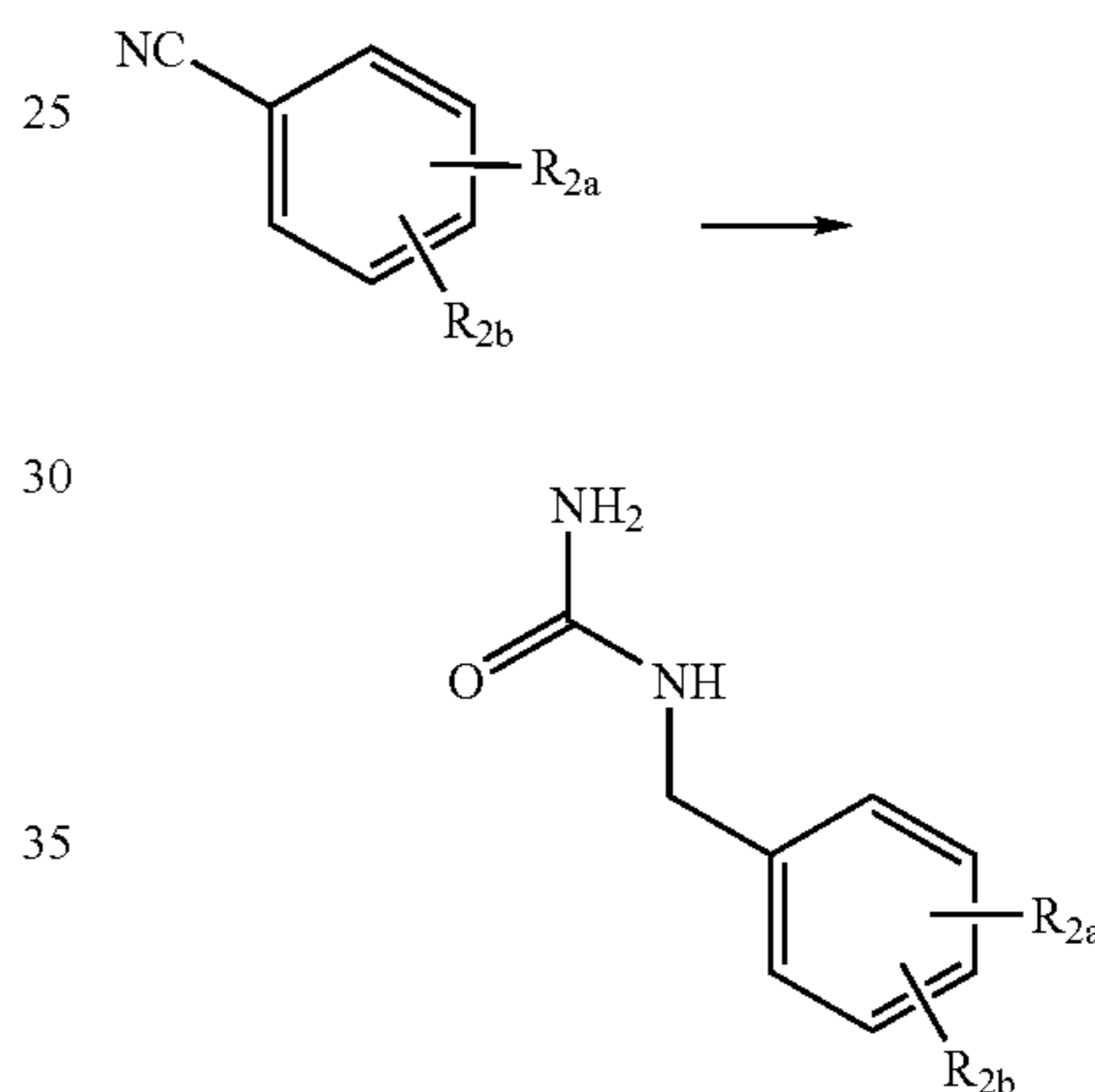
Reaction Scheme 1
