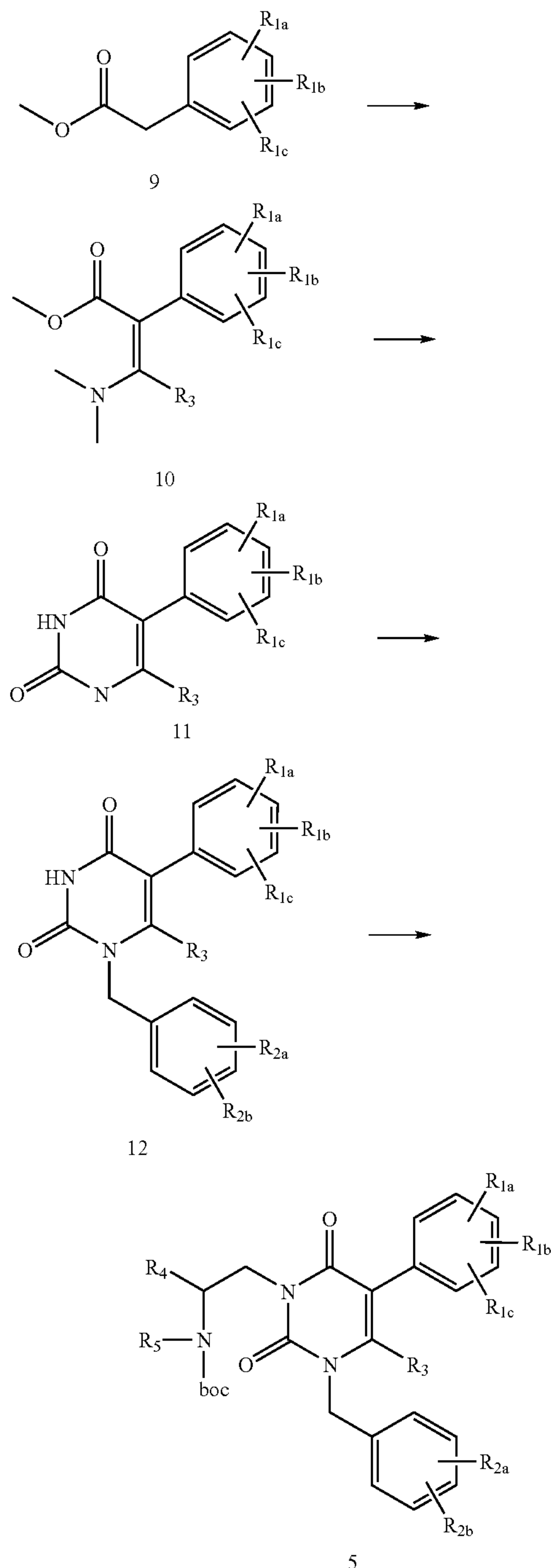
Reaction Scheme 3
