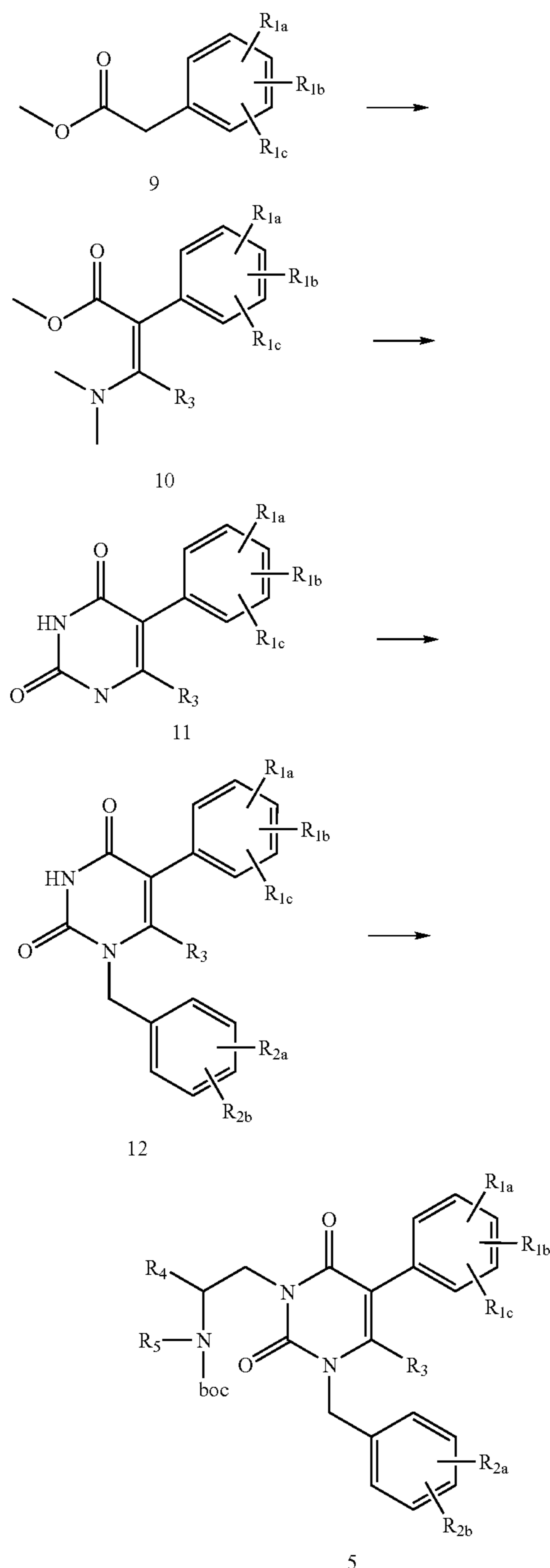
Reaction Scheme 3
