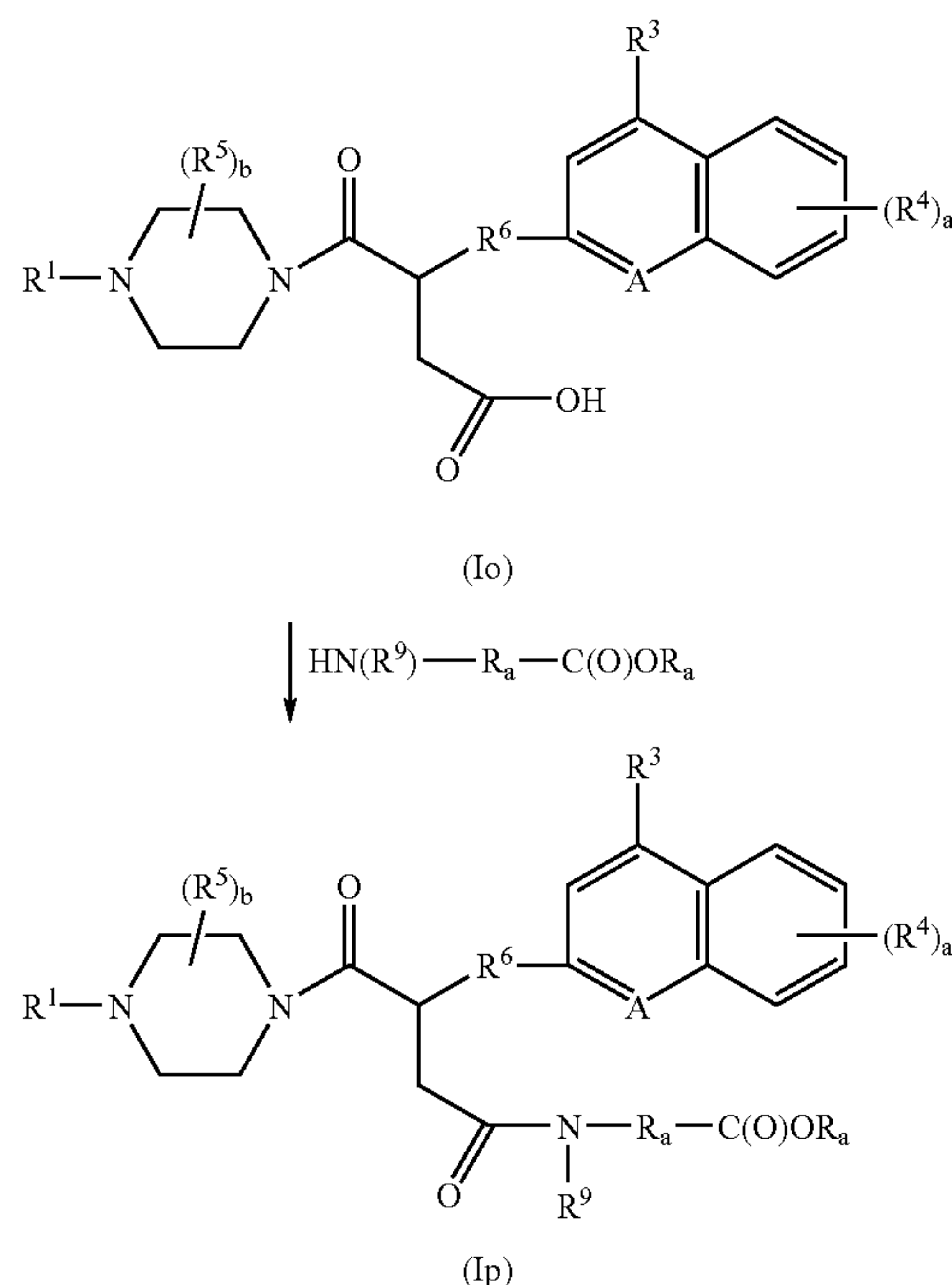
REACTION SCHEME 8
