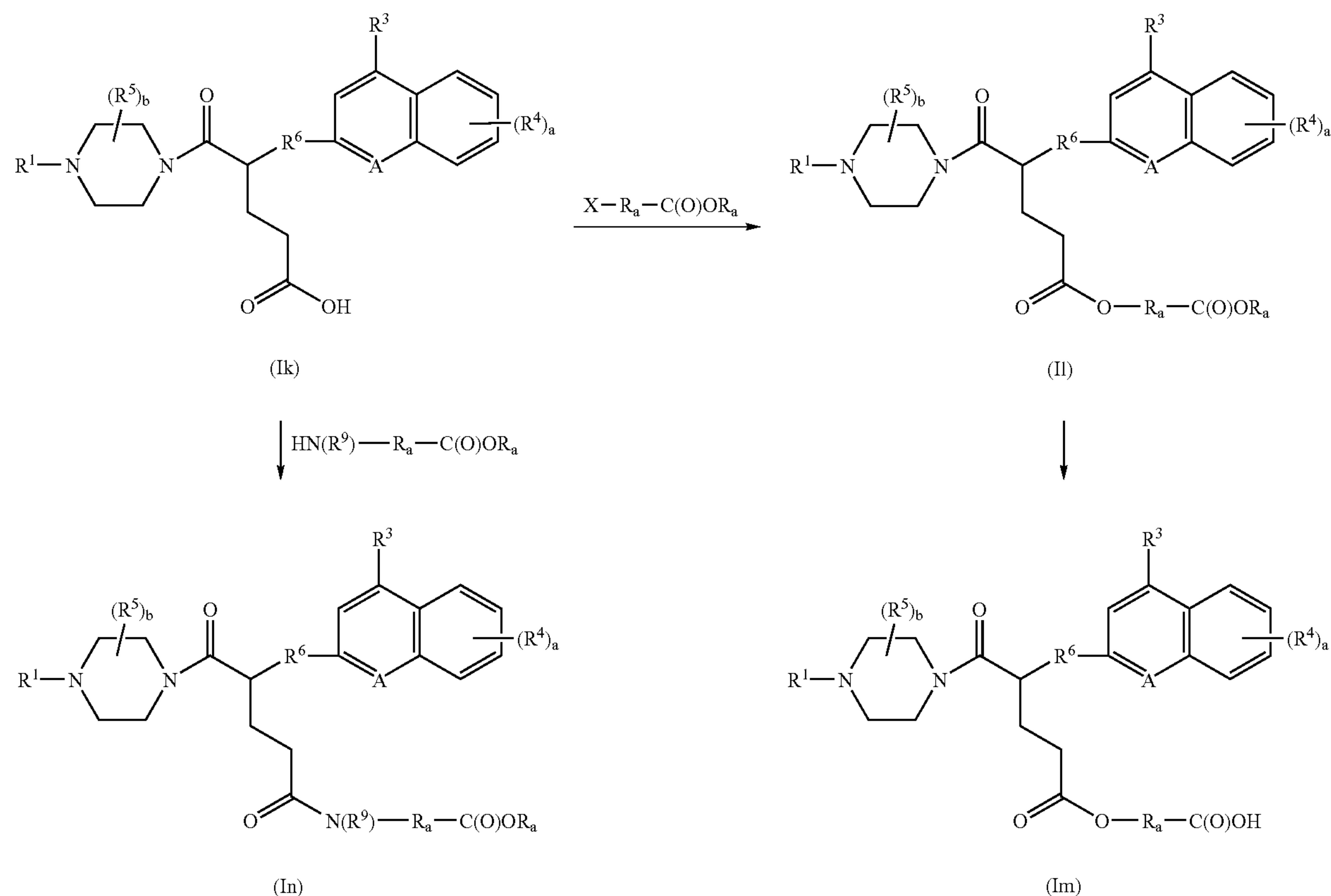
REACTION SCHEME 7
