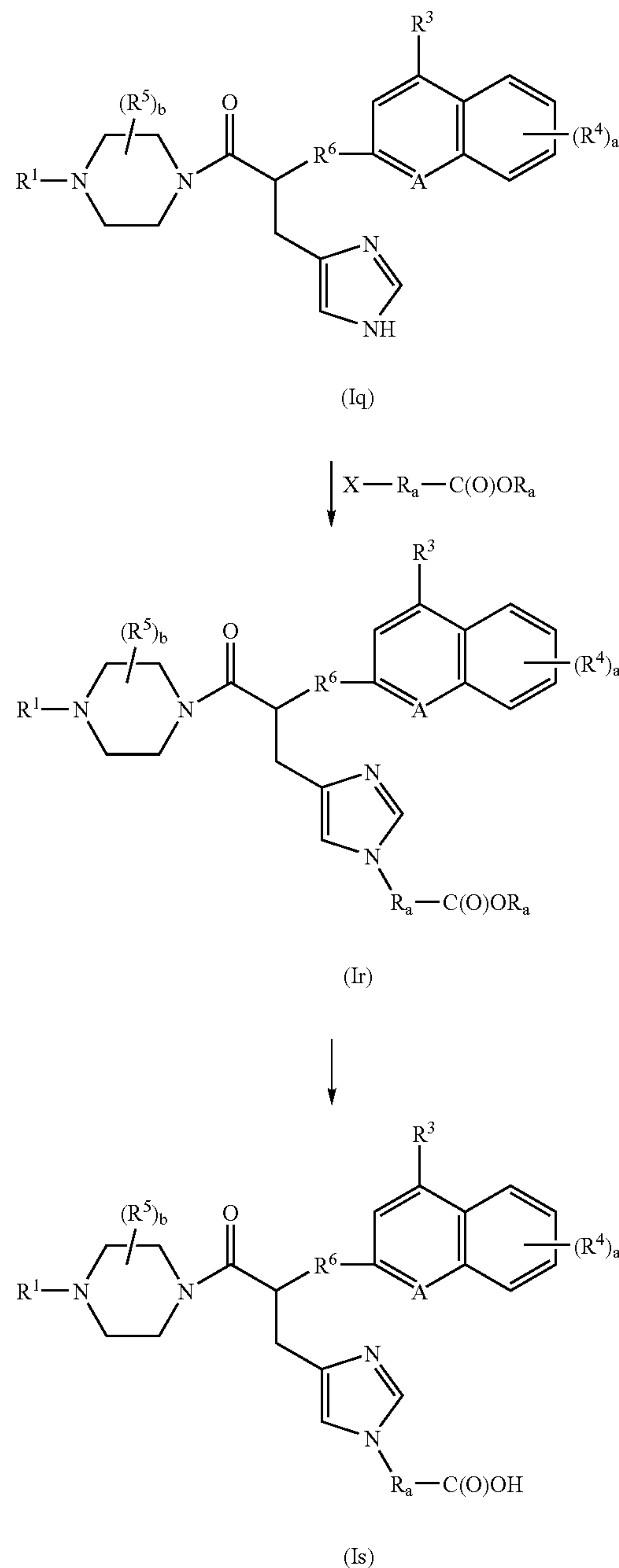
REACTION SCHEME 9
