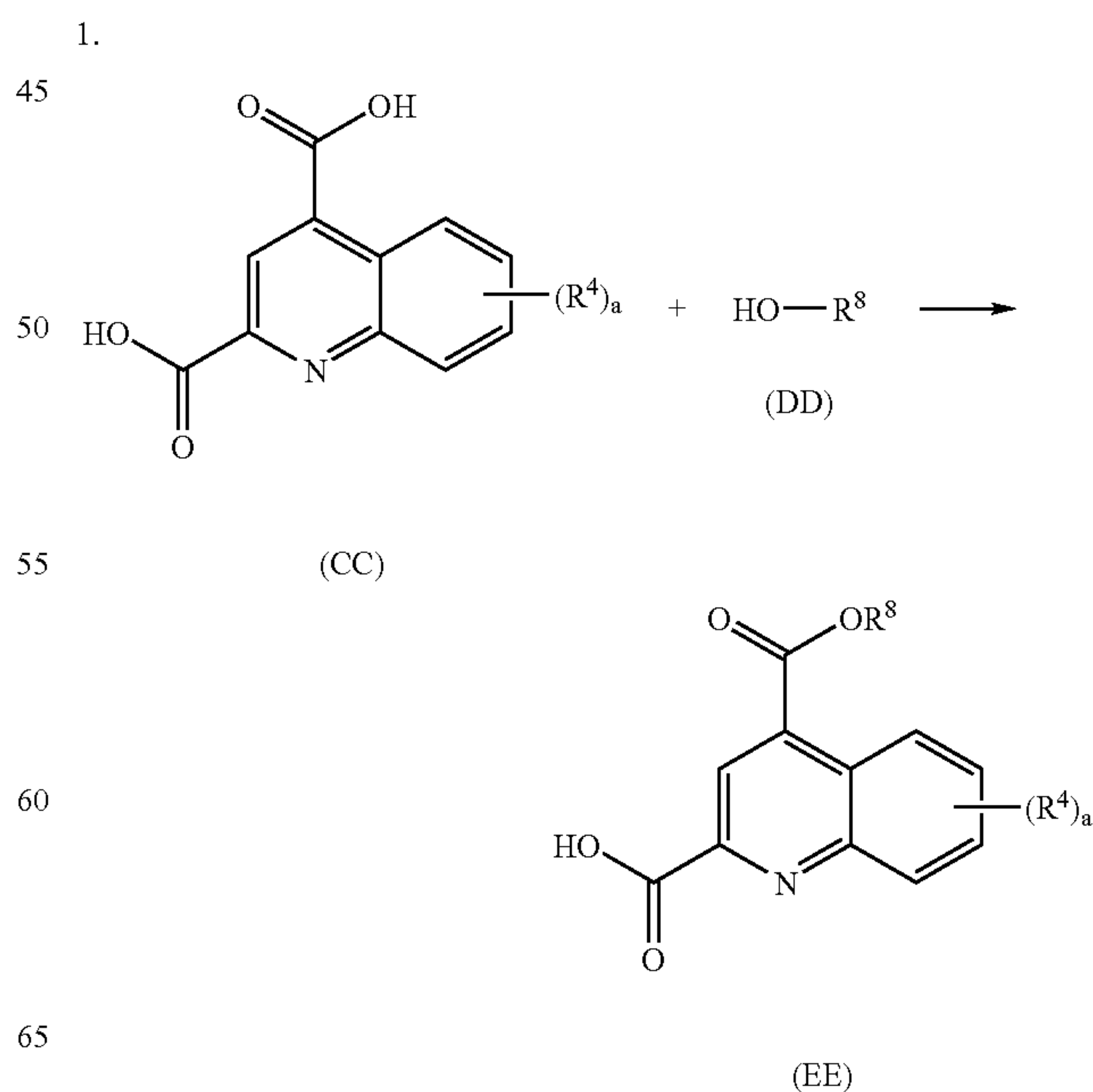
REACTION SCHEME 13
