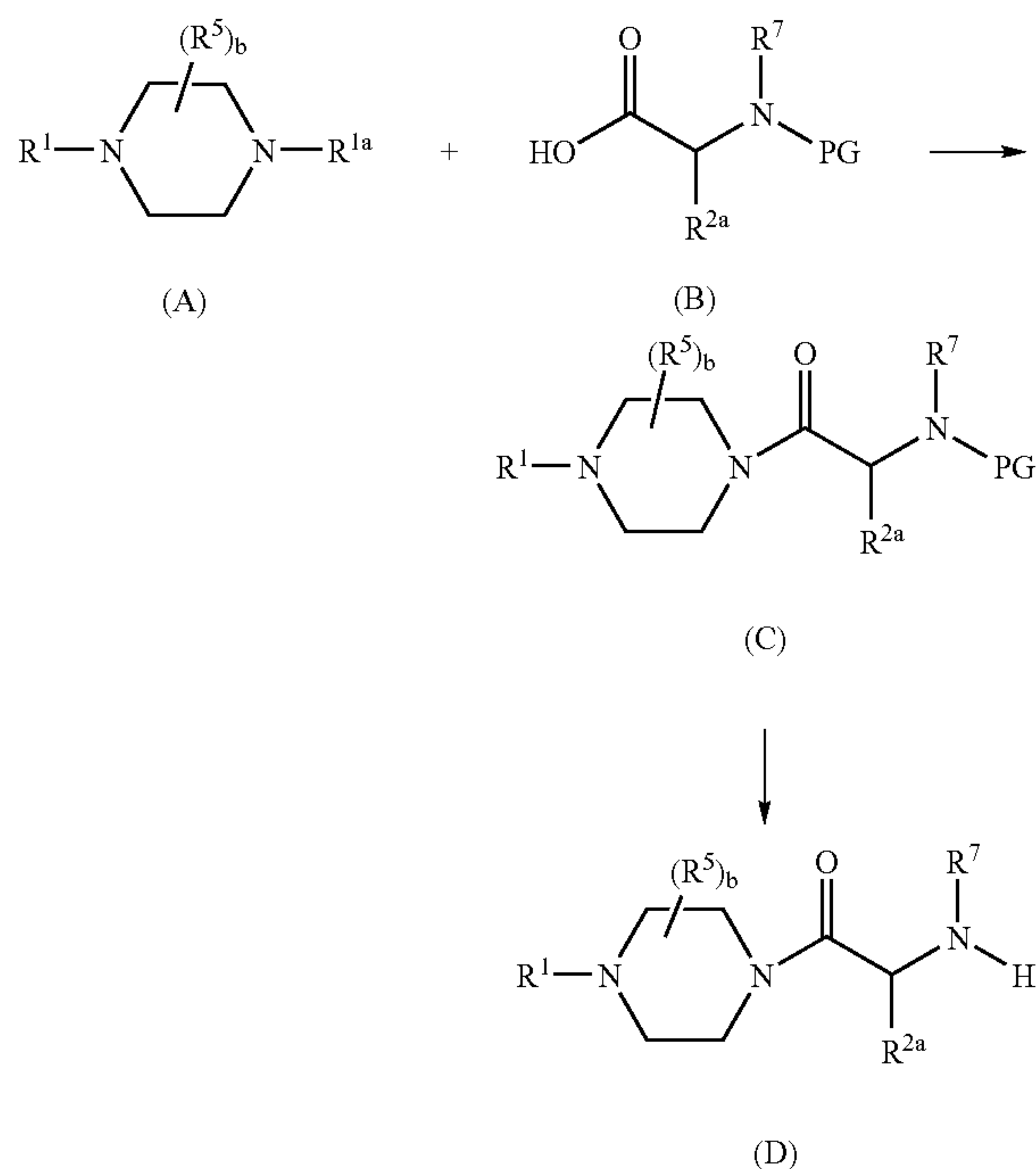
REACTION SCHEME 1
