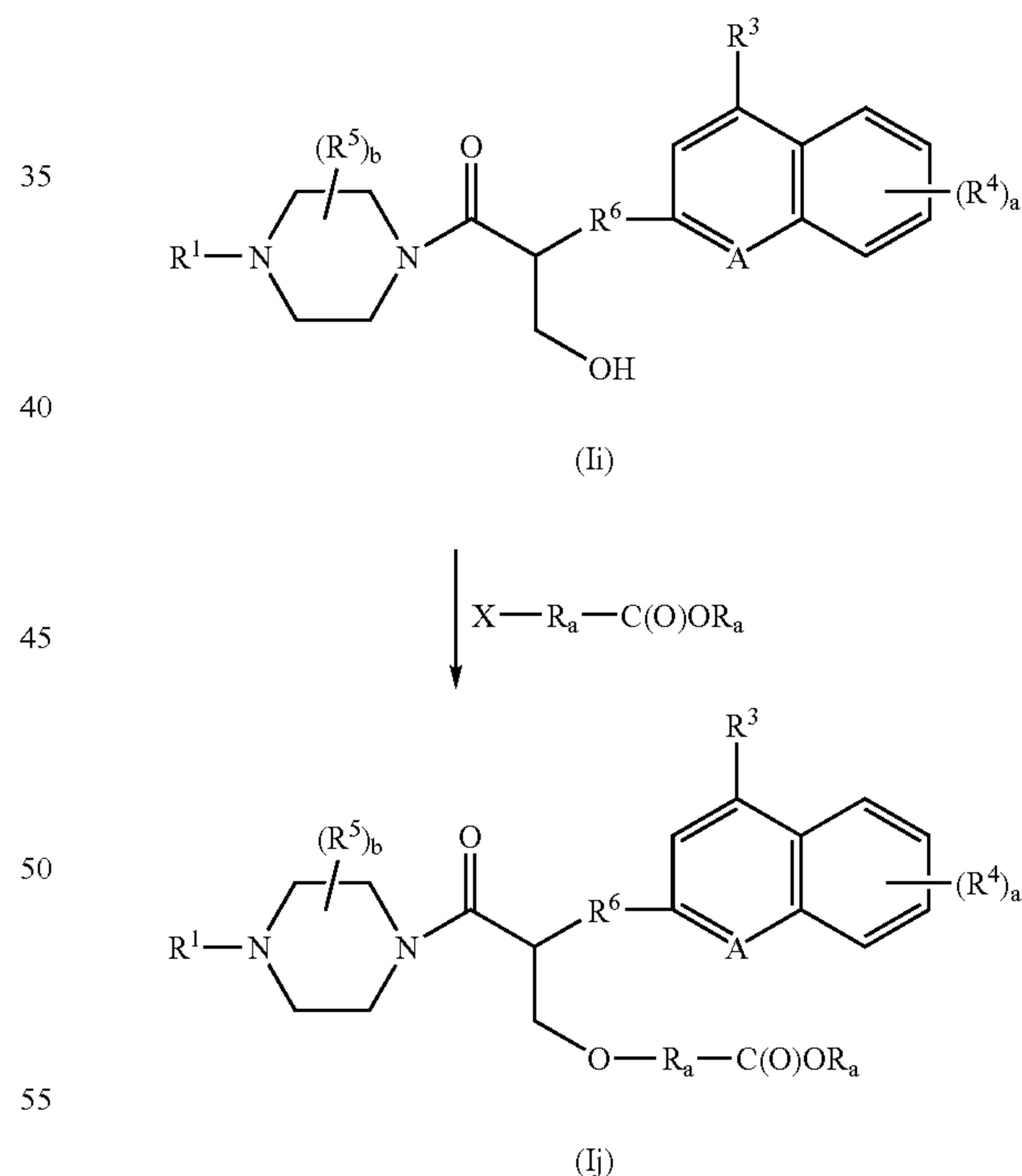
REACTION SCHEME 6
