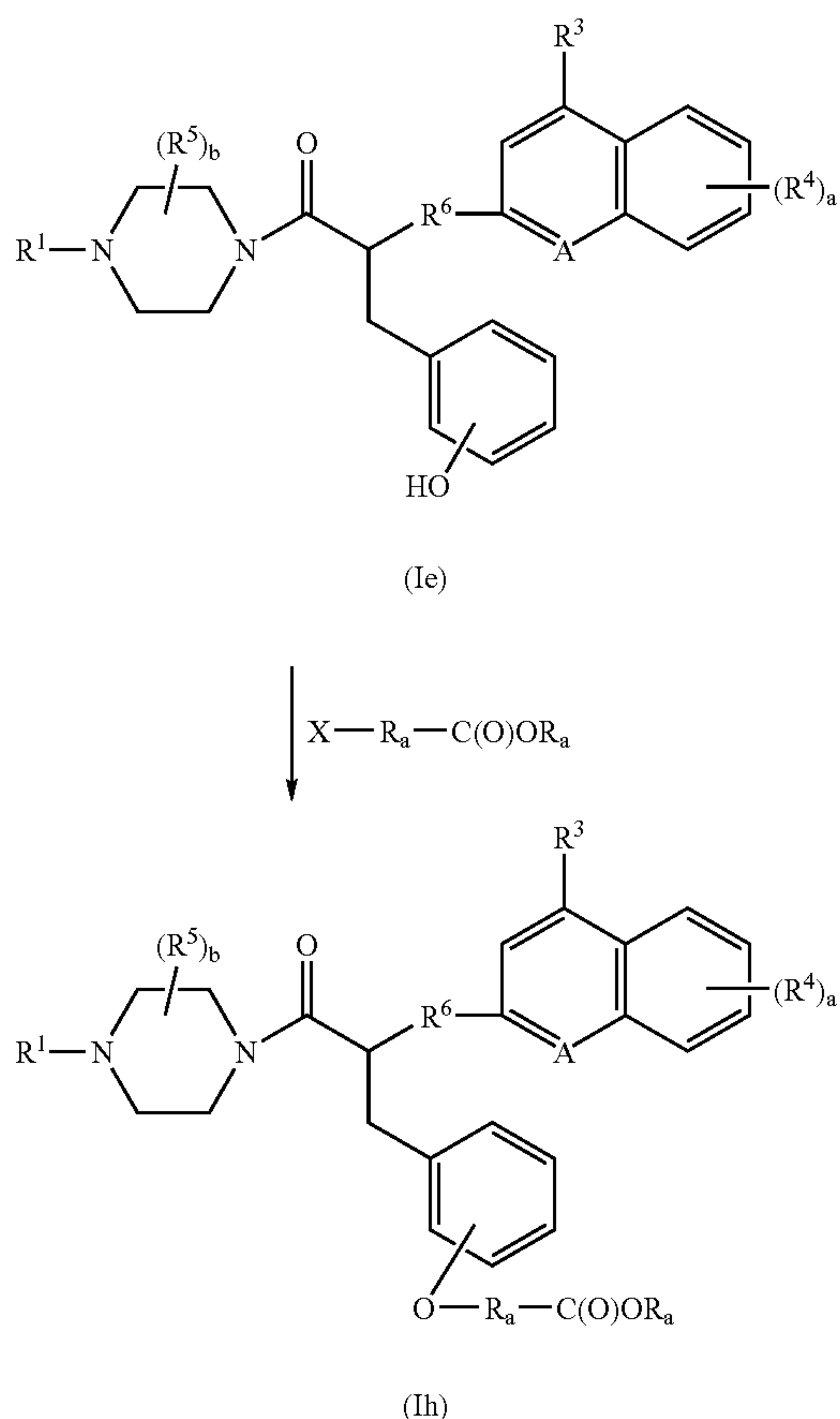
REACTION SCHEME 5
