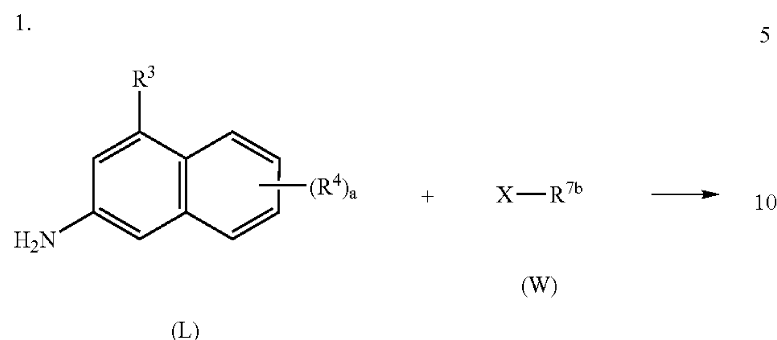
REACTION SCHEME 11
