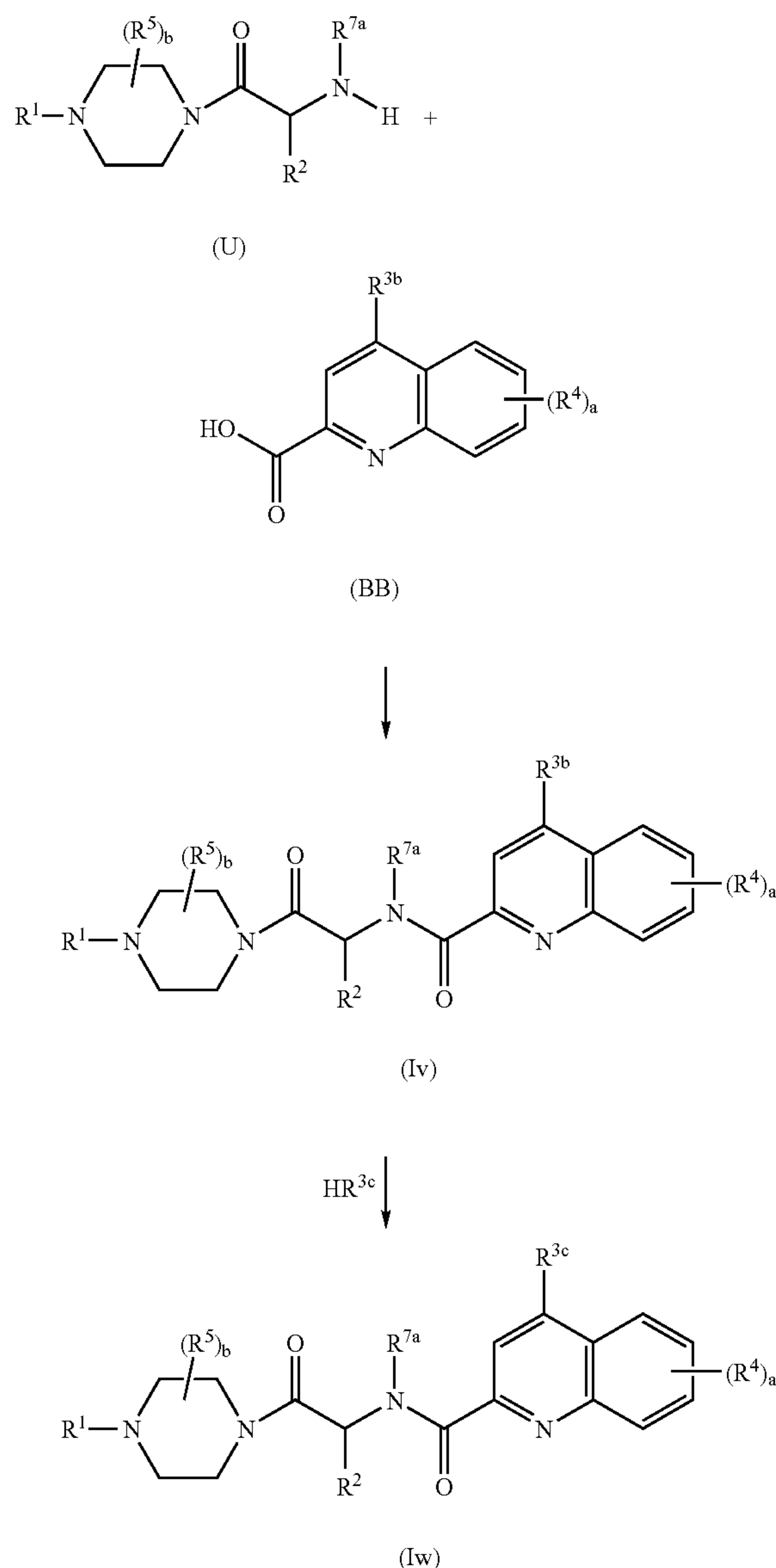
REACTION SCHEME 12
