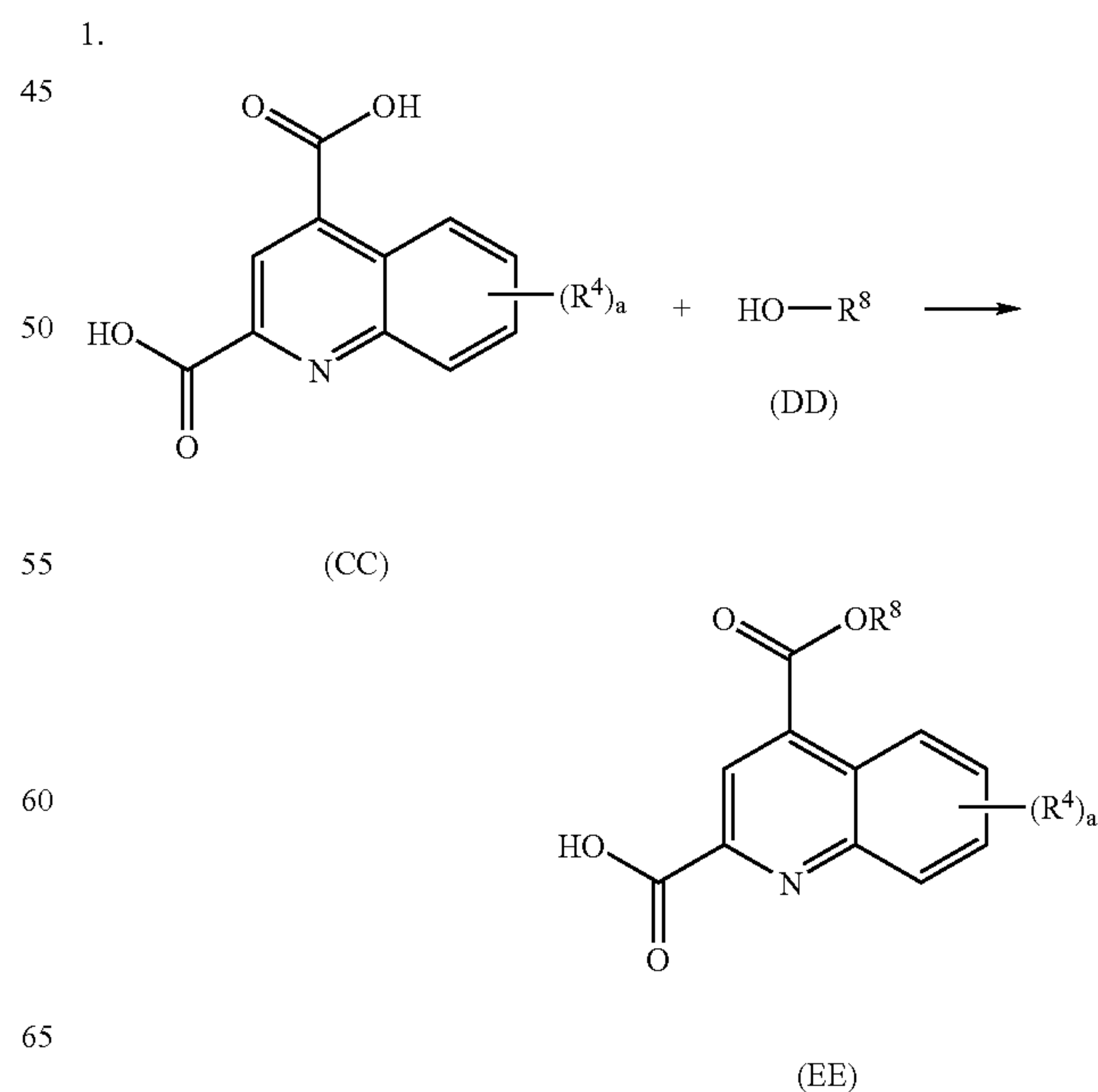
REACTION SCHEME 13
