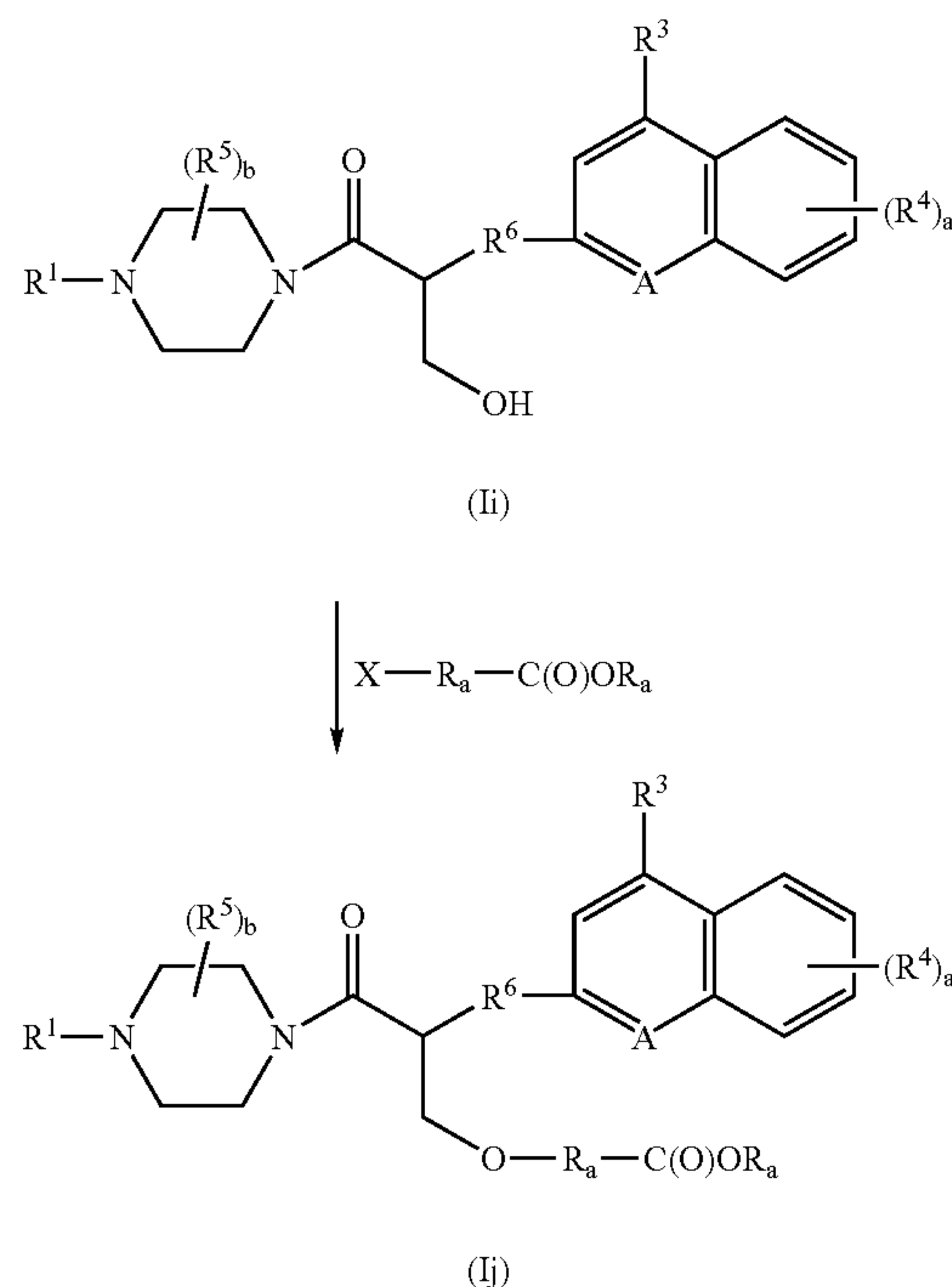
REACTION SCHEME 6
