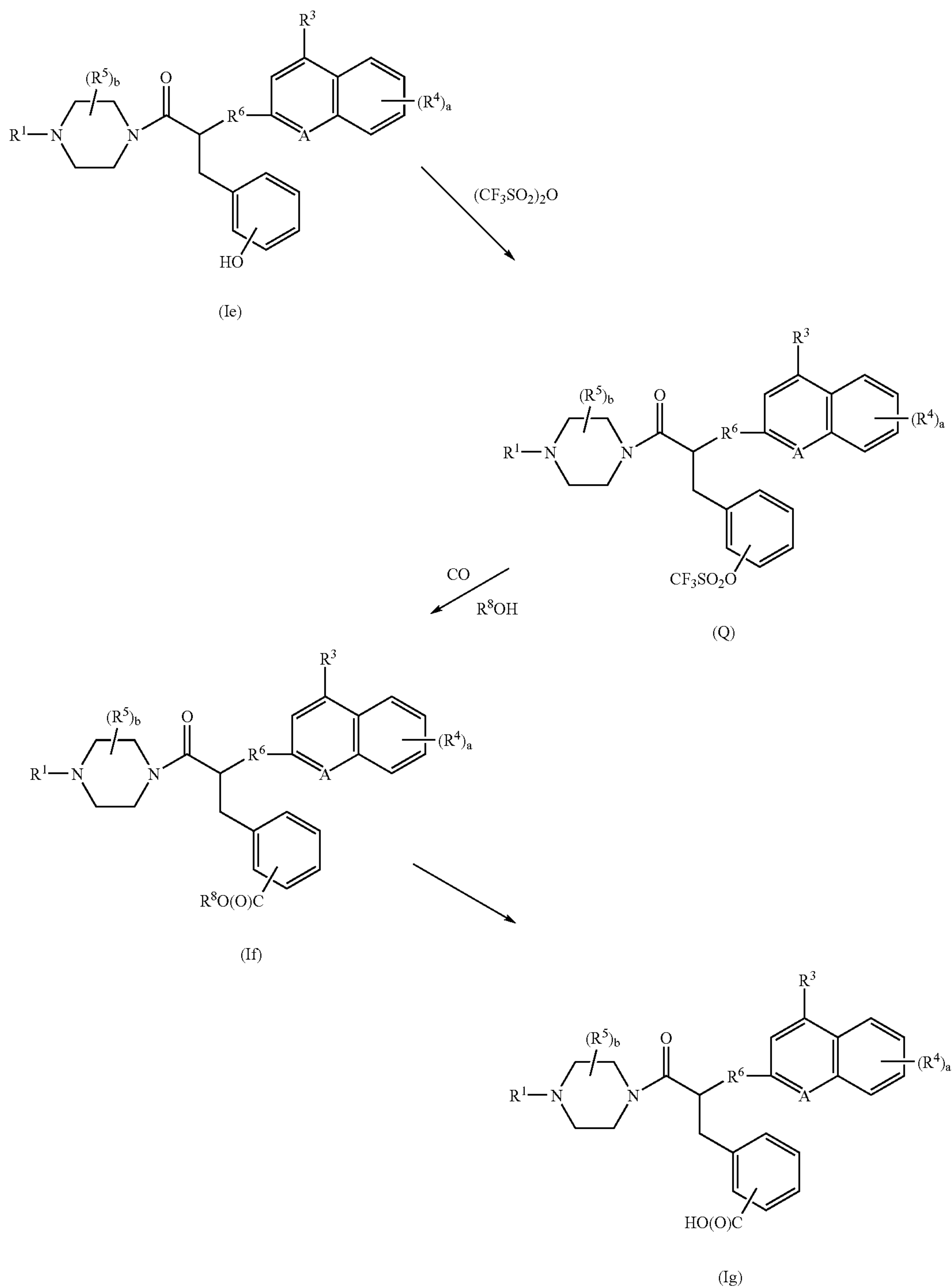
REACTION SCHEME 4
