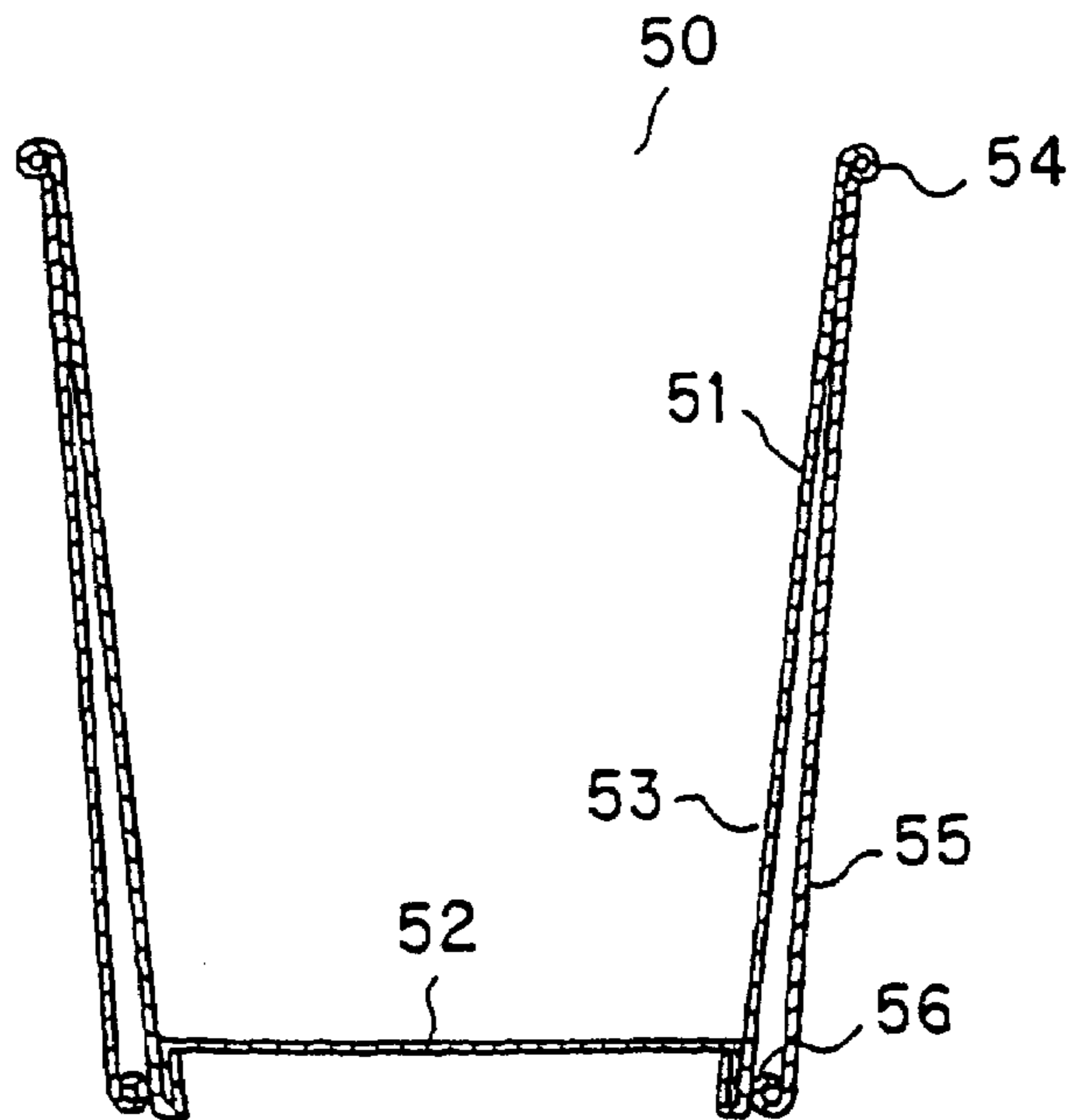
FIG. 43 PRIOR ART
