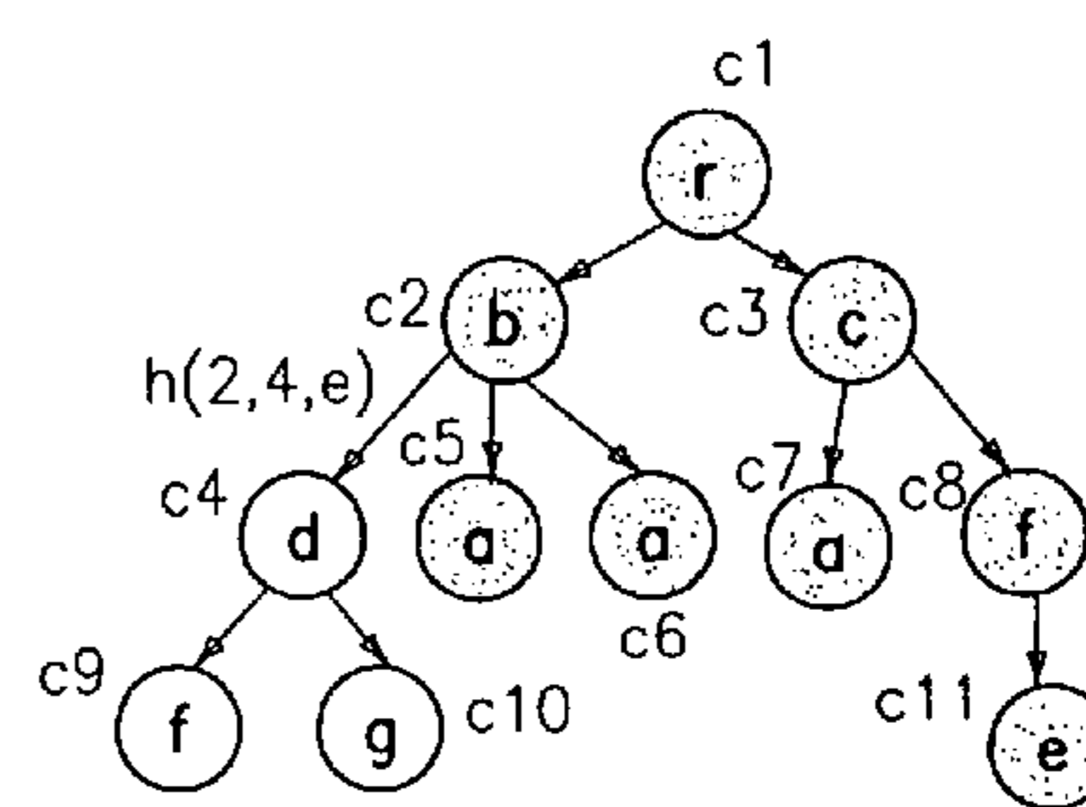
(c) Hint information at node 2 (8/11 nodes traversed)
