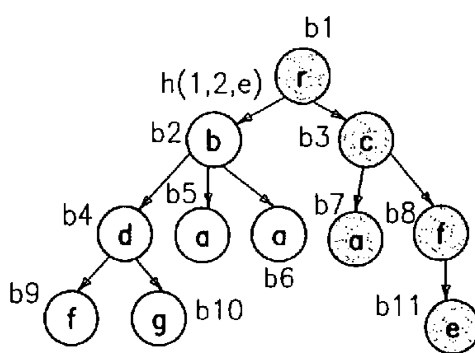
(b) Hint information at node 1 (5/11 nodes traversed)
