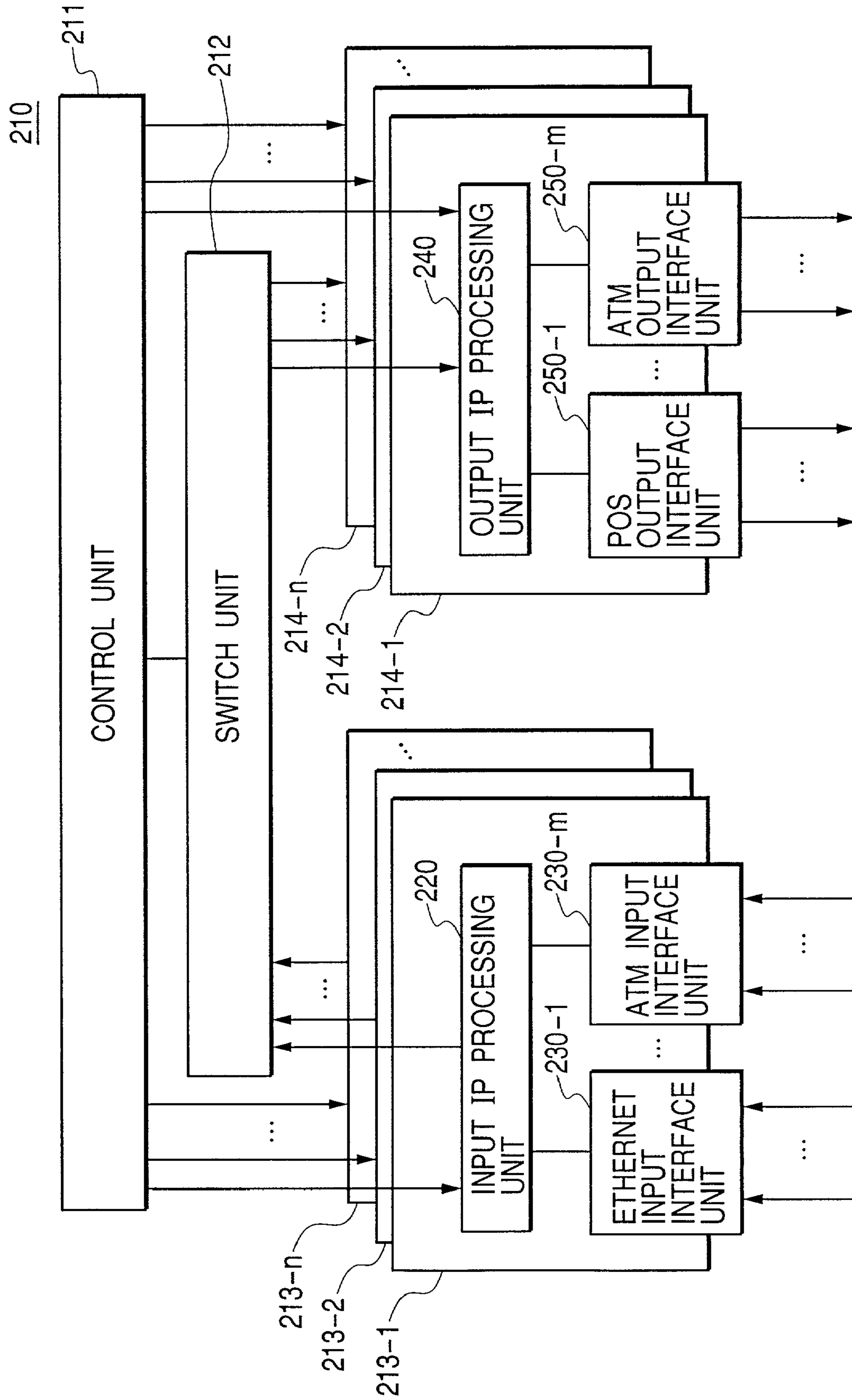
FIG. 23 PRIOR ART
