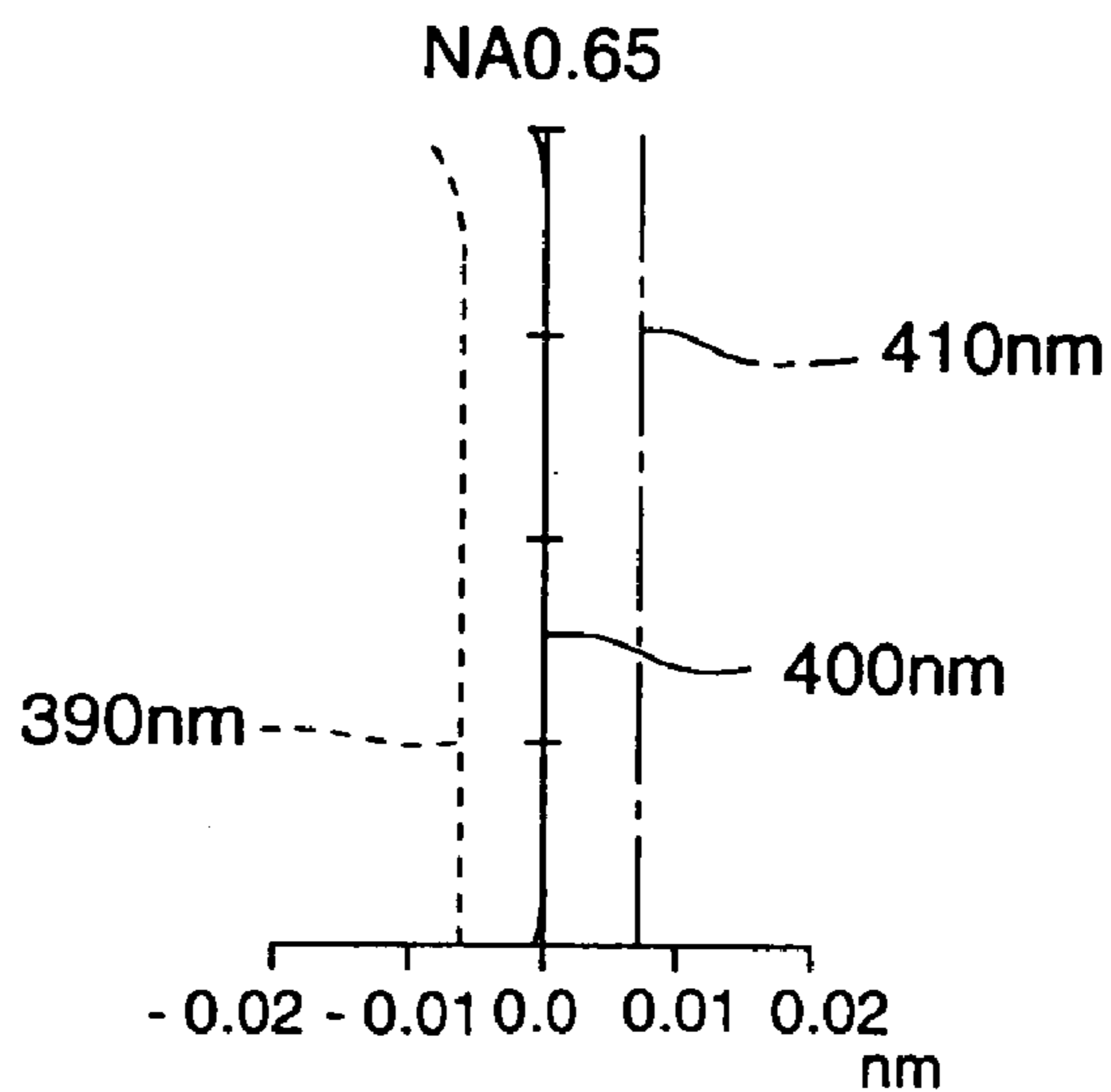
DIAGRAM SHOWING SPHERICAL ABERRATION
